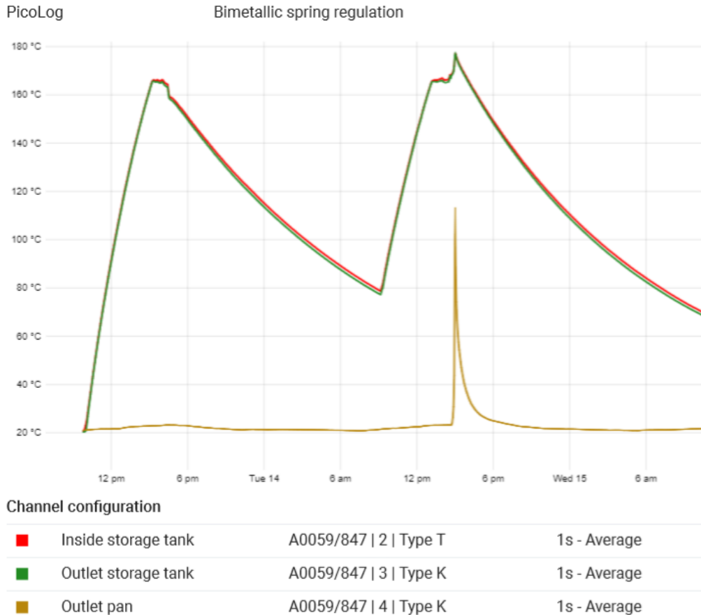
Figure 64: Test of bimetallic spring over 2 days
