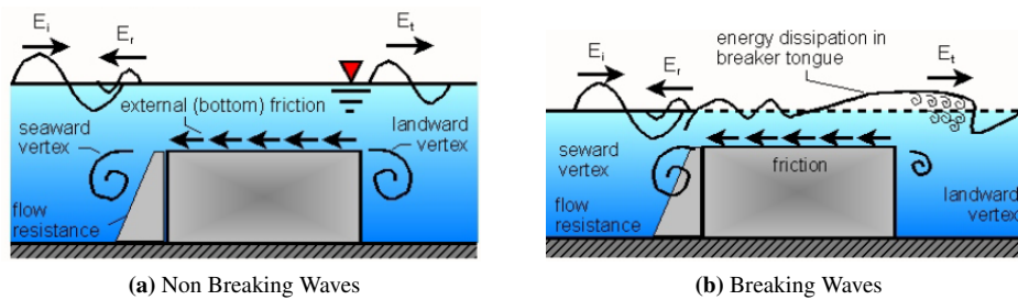
Figure 6.4: Phenomenon Contribution to Energy Loss at Artificial Reef, (Bleck, 2006).
