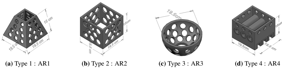
Figure 4.6: Scaled Artificial Reef Units with Designed Dimensions
