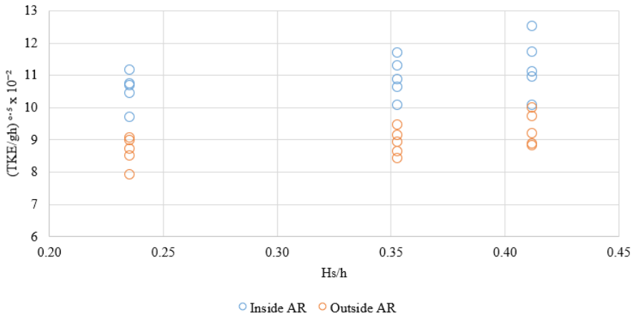
Figure 5.15: Turbulence for Configuration 3
