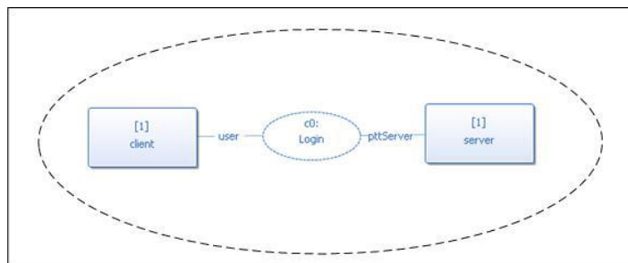
Figure 2-3: Collaboration Login
