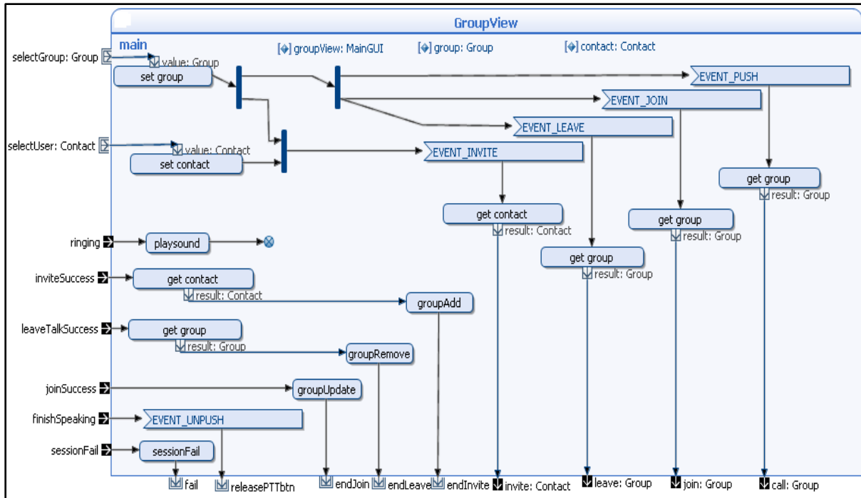
Figure 5-8: Group View building block
