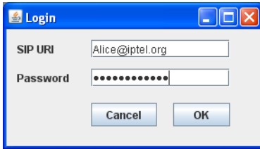
Figure 3-3: Login dialog
