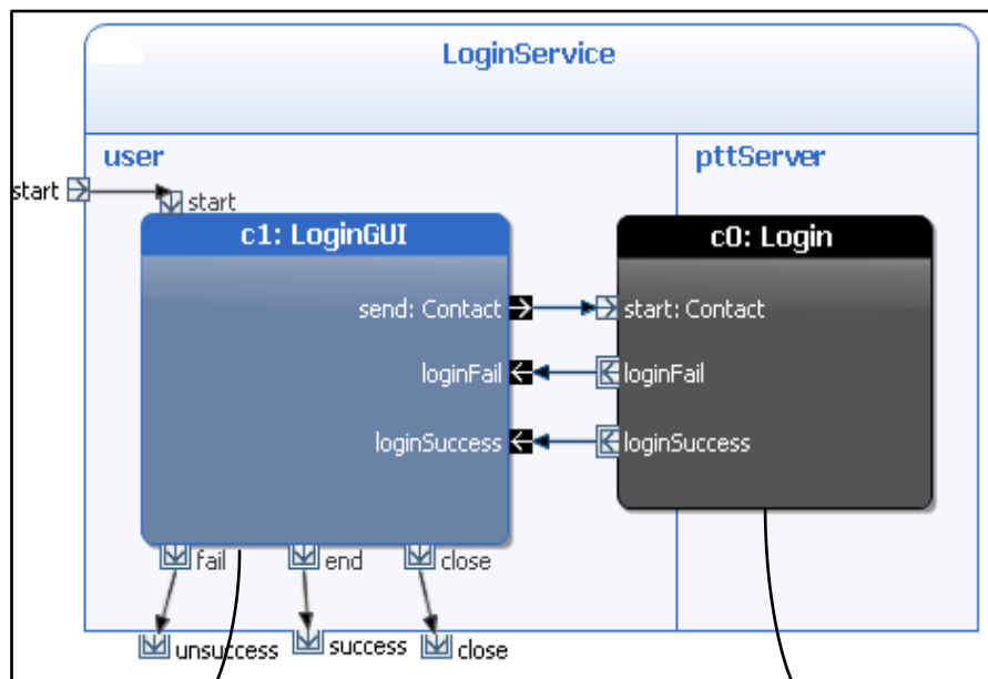
Figure 5-1: Login service building block
