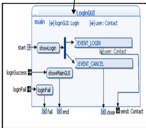
Figure 5-2: LoginGUI building block
