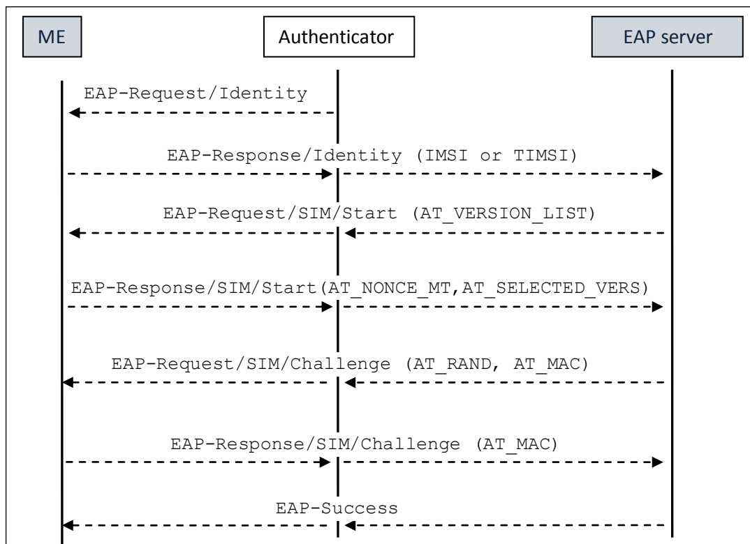
Figure 3.3.2.1: EAP-SIM authentication
