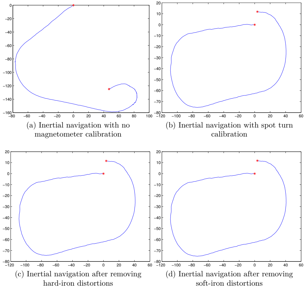
Figure 8.13: Inertial navigation before and after magnetometer calibrations
