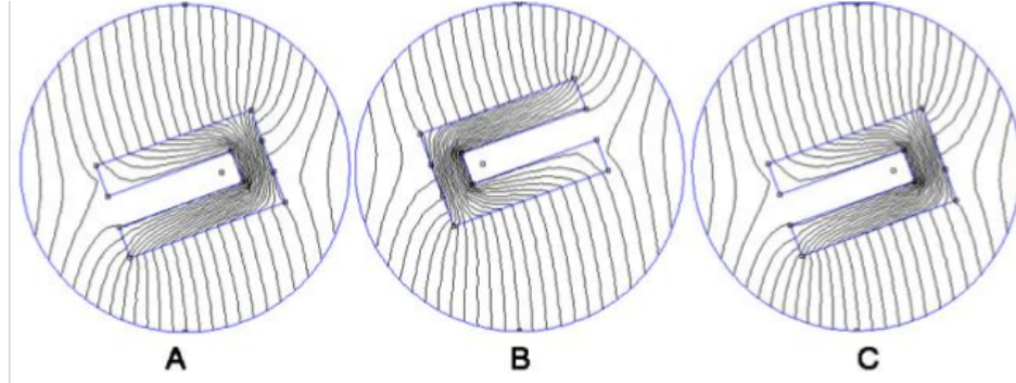
Figure 6.4: Soft Iron Distortion in a Uniform Field [?]
