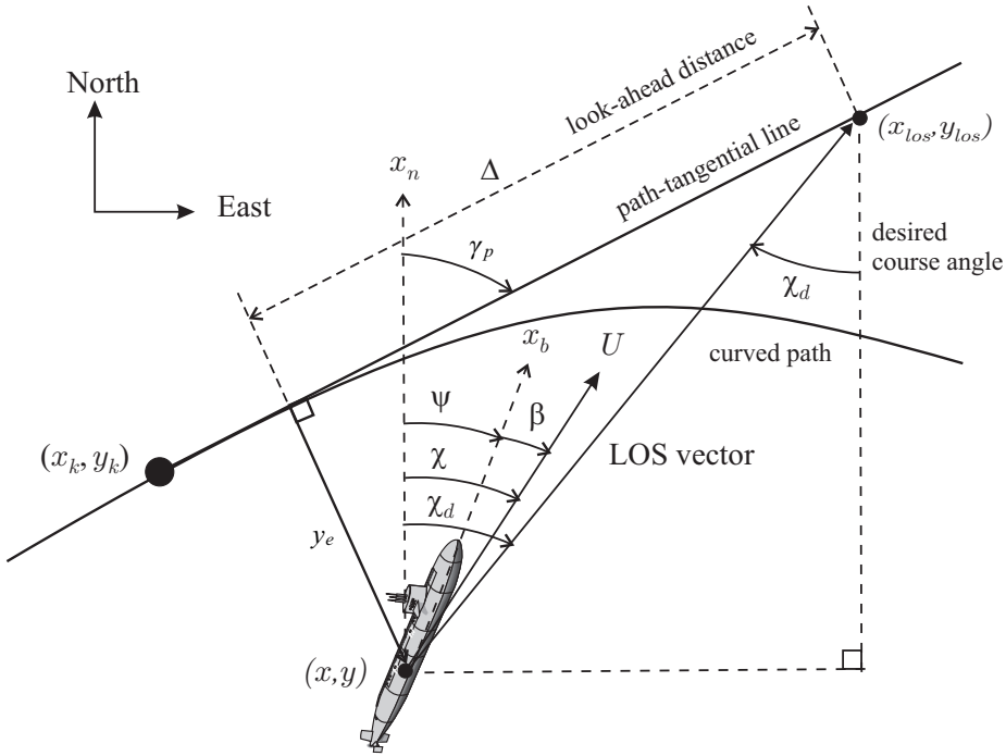
Figure 8.1: Line-of-sight guidance geometry for curved paths.
