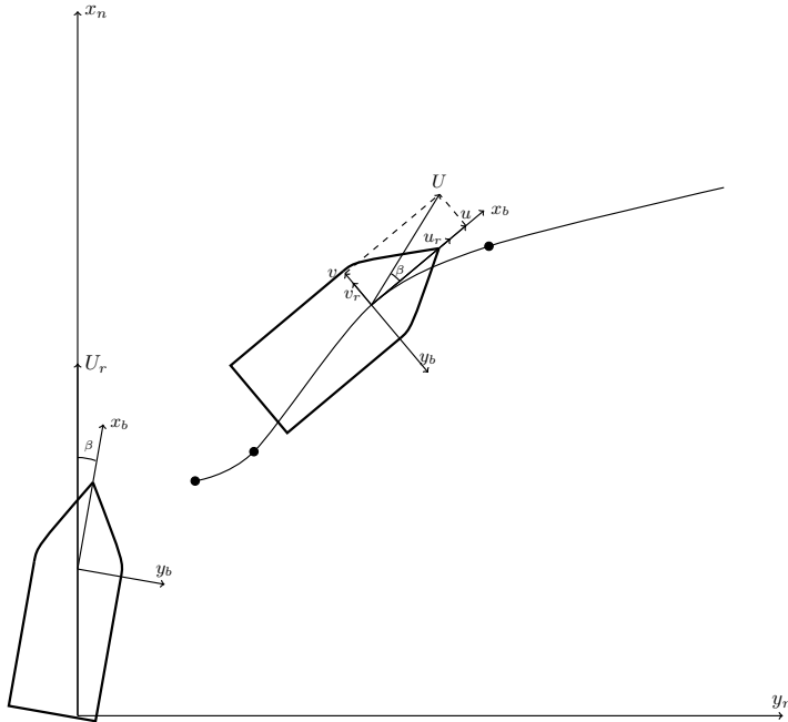
Figure 9.1: Sideslip angle, with a current coming from the east, hence affecting the velocity components.
