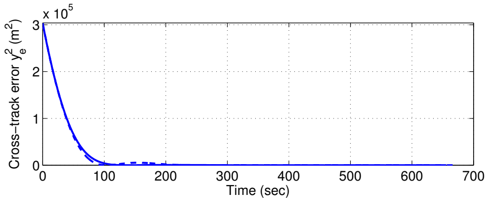
Figure 8.9: Squared cross-track error comparison between the constant LOS algorithm with \Delta_{7,\text{opt}} = 300 \text{ m} (dashed line) and the proposed method (solid line).
