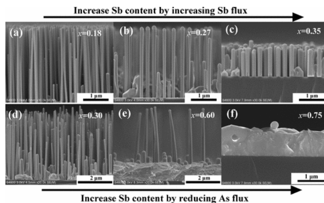
Figure 8. Side-view SEM images of self-catalyzed \text{GaAs}_{1-x}\text{Sb}_x NWs grown on Si(111) substrates by MBE. (a–c) \text{GaAs}_{1-x}\text{Sb}_x NWs with different Sb content were obtained by increasing the Sb flux and corresponding x values are 0.18, 0.27, and 0.35, respectively. (d–f) \text{GaAs}_{1-x}\text{Sb}_x NWs with different Sb content were obtained by reducing the As flux and corresponding x values are 0.30, 0.60, and 0.75, respectively. (Adapted with permission from [44]. Copyright 2014 American Chemical Society.)
