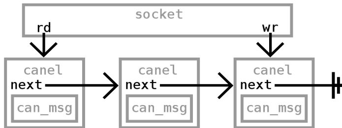
Figure 4.1: Each socket is a FIFO queue, implemented as a singly-linked list.
