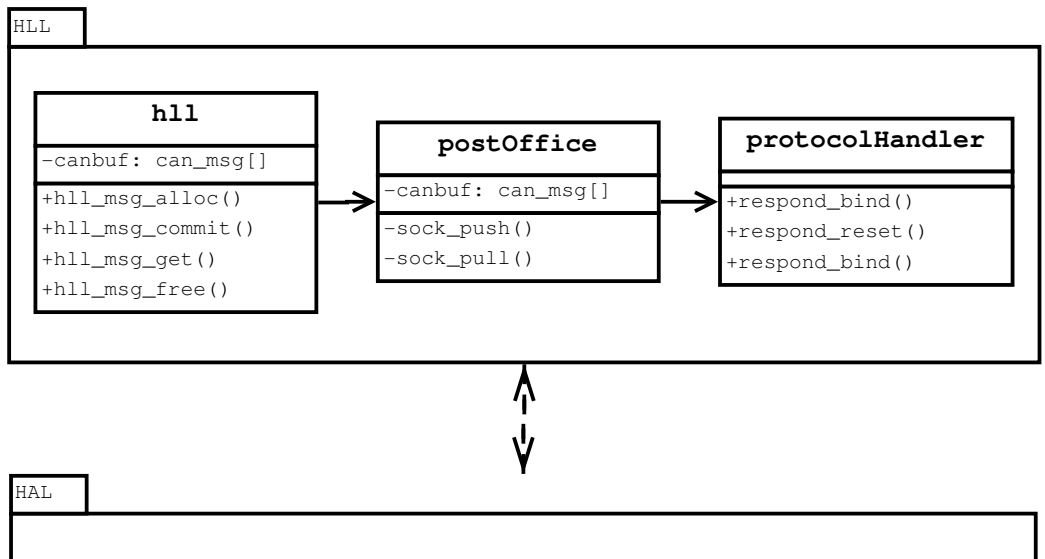
Figure 3.1: Class diagram of HLL. A possible source of confusion is the hll class inside the HLL package.
