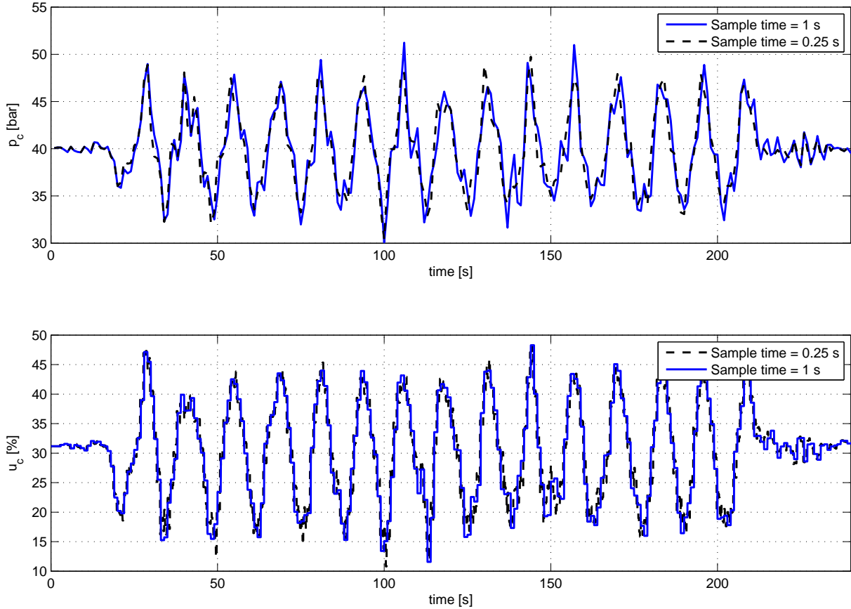
Figure 2.9: Comparison of different control update rates. Choke pressure and control signal.
