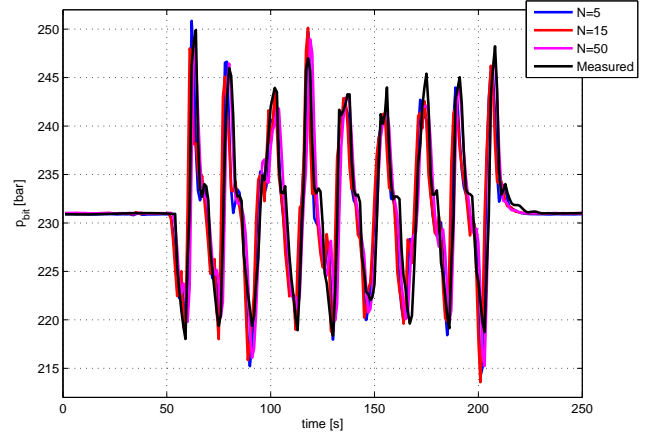
Figure 4. Simulation results compared to measured data, p_{bit} , different number of control volumes.
