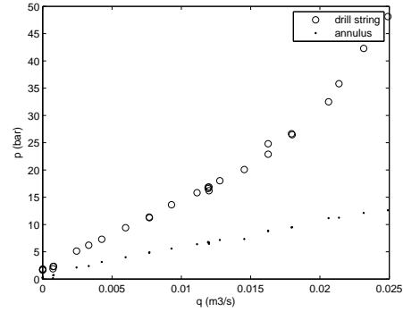
Figure 3. Pressure drops in drill string and annulus, UIIRigg data.
