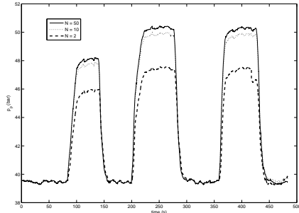
Figure 12. Rotating drill string, different number of control volumes.
