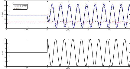
Figure 15. Comparison of control volume method and model reduction by balanced truncation, 7th order models.
