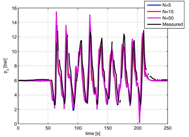
Figure 5. Simulation results compared to measured data, p_c , different number of control volumes.
