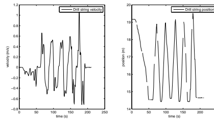
Figure 7. Position and velocity for heave emulation, UIIRigg.
