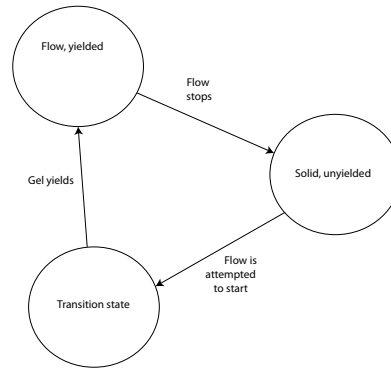
Figure 4. State diagram for gel/liquid behavior.
