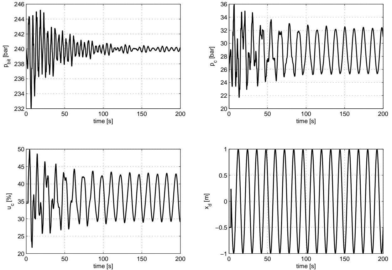
Figure 6.11: Simulation results, IMC without feedback linearization. Bottom hole pressure, choke pressure, control signal and drill string movement. The bottom hole pressure set point is 240 bar.
