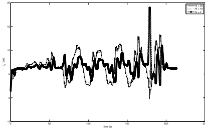
Figure 9. Heave simulation, different number of control volumes.
