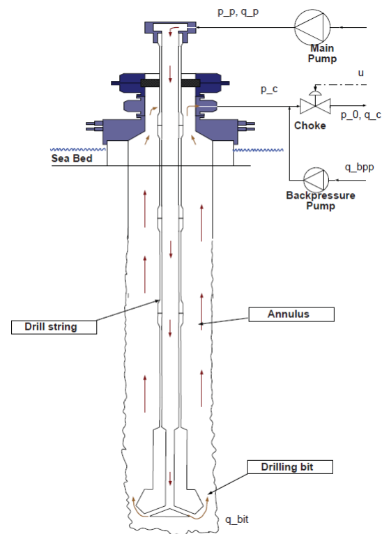
Figure 1. Well and hardware configuration in managed pressure drilling system.
