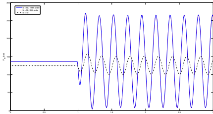
Figure 16. Comparison of control volume method and model reduction by balanced truncation, 39th order models.
