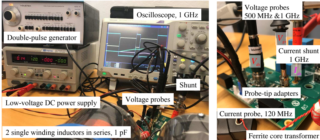
(a) Hardware setup.
