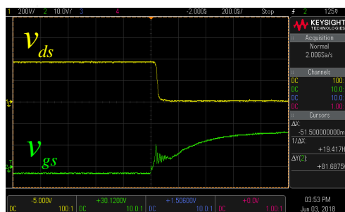
(b) Measured v_{ds} and v_{gs} during turn-on.
