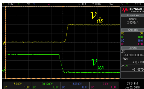
(a) Measured v_{ds} and v_{gs} during turn-off.
