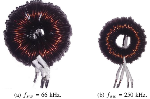
Fig. 11. Switching at 66 kHz requires 2 \times stacked sendust core, CS358060, with 70 turns giving 565 \mu\text{H} , whereas at 250 kHz, only a 1 \times stacked sendust core, CS330060, is sufficient, leading to a dramatic reduction in the size of the inductor.
