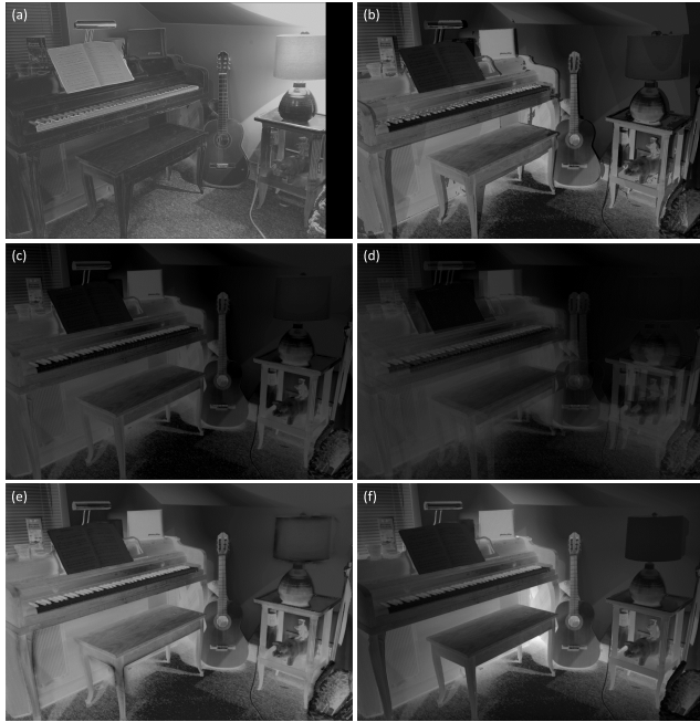
FIGURE 19. JND profiles of “Piano” stereo pair obtained using different 3D-JND models. (a) BJND map, (b) JJND map, (c) MJND map, (d) SJND map, (e) HJND map, (f) DJND map.
