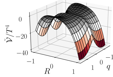
FIG. 3. Normalized R -dependent part of the effective potential in the \chi M model at T = \mu = 200 MeV, and \Delta = 150 MeV.
