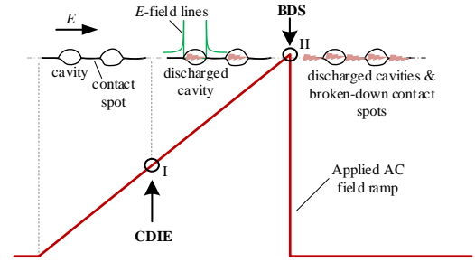
Figure 3. Modeled mechanisms of the cavity discharge and the breakdown of contact spots in parallel with applied field ramp.
