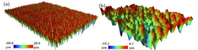
Figure 5. 3D XLPE surface profiles ground by #500: (a) Roughness profile. (b) Waviness profile.
