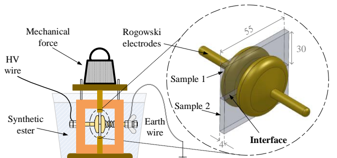
Figure 4. Illustration of the test set-up. All dimensions are in mm, electrode diameter = 40 mm. The interface is 4-mm, parallel to the direction of the field.
