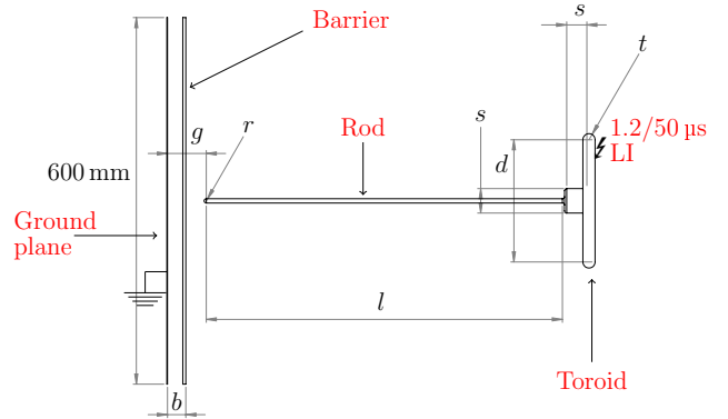
Fig. 1. Rod-barrier-plane model. See table I for parameters. The Lexan barrier was 600x600x5 mm, the ground plane of 600x1000x1 mm. Toroid dimensions: d = 200 mm, t = 20 mm, s = 40 mm.
