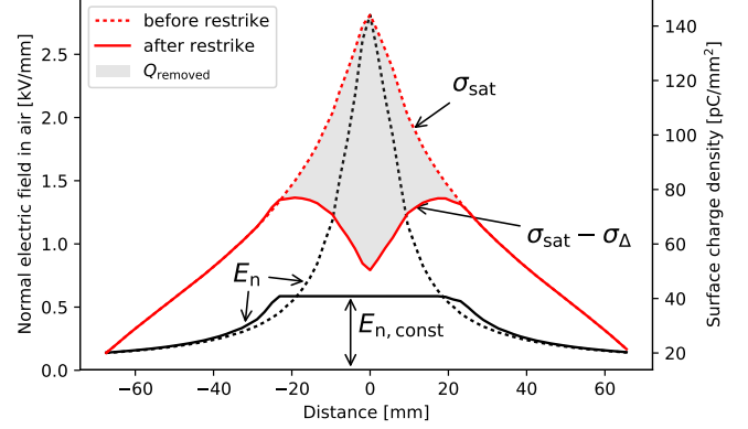
Fig. 2. Charge density and normal field distributions before and after a simulated restriking. The presented values correspond to the configuration 3 in table I. The value of Q_{\text{removed}} is equal to 5% of the total saturation charge and has been estimated iteratively so that U = U_{i,\text{res}} .
