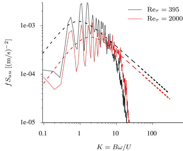
Fig. 8: Spectra of the stream-wise velocity fluctuations for Re_\tau = 395 and Re_\tau = 2000 with von Kármán fitting.
