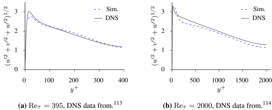
Fig. 6: RMS of velocity fluctuations in nondimensional units for the channel-flow simulations.
