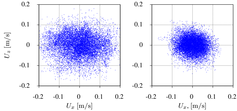
Fig. 7: Scatter plot of the stream-wise and span-wise velocity fluctuations at the channel centerline. Left: Re_\tau = 395 ; Right: Re_\tau = 2000 .
