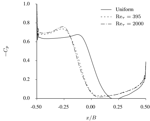
Fig. 15: Time-averaged pressure coefficient on a surface of the BD10 section for different flow conditions.
