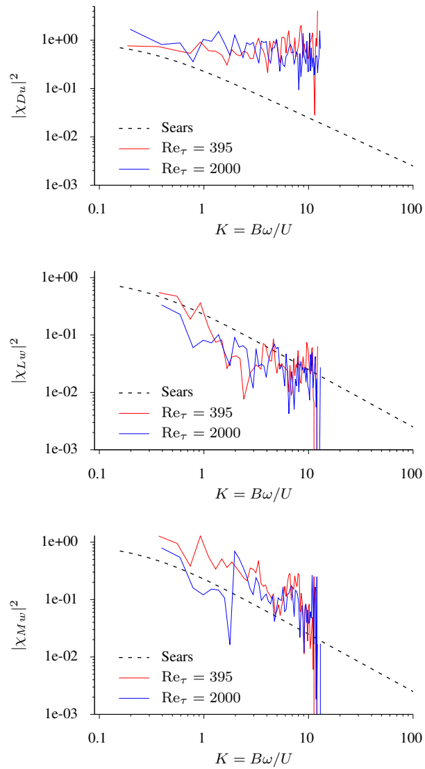
Fig. 14: Aerodynamic admittance functions.
