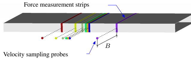
Fig. 10: Velocity and force sampling layout.
