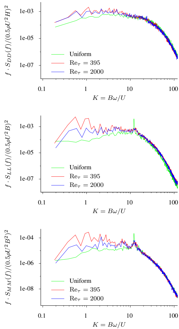
Fig. 13: Normalized spectra of the drag, lift and pitching moment for uniform inflow, Re_\tau = 395 and 2000.
