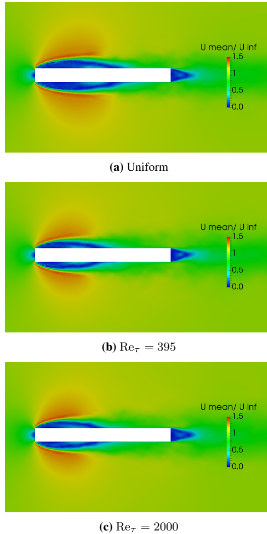
Fig. 16: Contours of time-averaged flow velocity divided by \bar{U}_b for different flow conditions.
