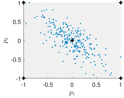
Fig. 3. Multivariate plot of the two parameters. The points \mathbf{p}_j \in \{(-1, -1), (1, -1), (0, 0), (-1, 1), (1, 1)\} are represented by the black '+' and the gray shaded area represents the univariate limits of the two parameters.
