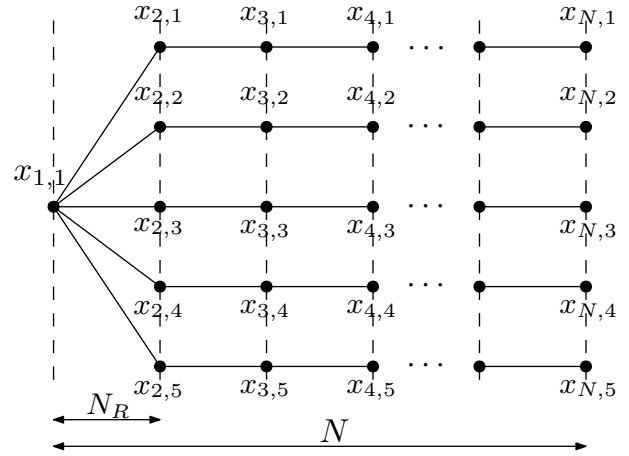
Fig. 1. Schematic representation of a scenario tree generated for M = 5 models and a robust horizon of N_r = 1 .
