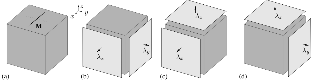
Figure 7: (a) Unit cube of a transversely isotropic tissue consisting of one family of fibers with the orientation \mathbf{M} parallel to the x -direction, initially subjected to uniaxial deformations in the x -, y - and z -directions followed by a series of planar biaxial deformations (b) in the xy -plane; (c) in the xz -plane; (d) in the yz -plane.
