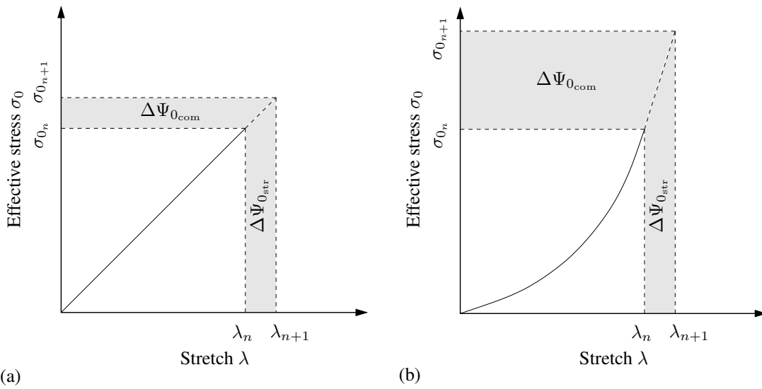
Figure 15: Qualitative sketch showing the relationship between the effective stress \sigma_0 and stretch \lambda , and the incremental change from \sigma_{0n}-\lambda_n to \sigma_{0n+1}-\lambda_{n+1} at a typical time step \Delta t = t_{n+1} - t_n : (a) linear; (b) nonlinear material behavior with the corresponding changes in the effective complementary energy \Delta\Psi_{0,com} and the effective strain energy \Delta\Psi_{0,str} .
