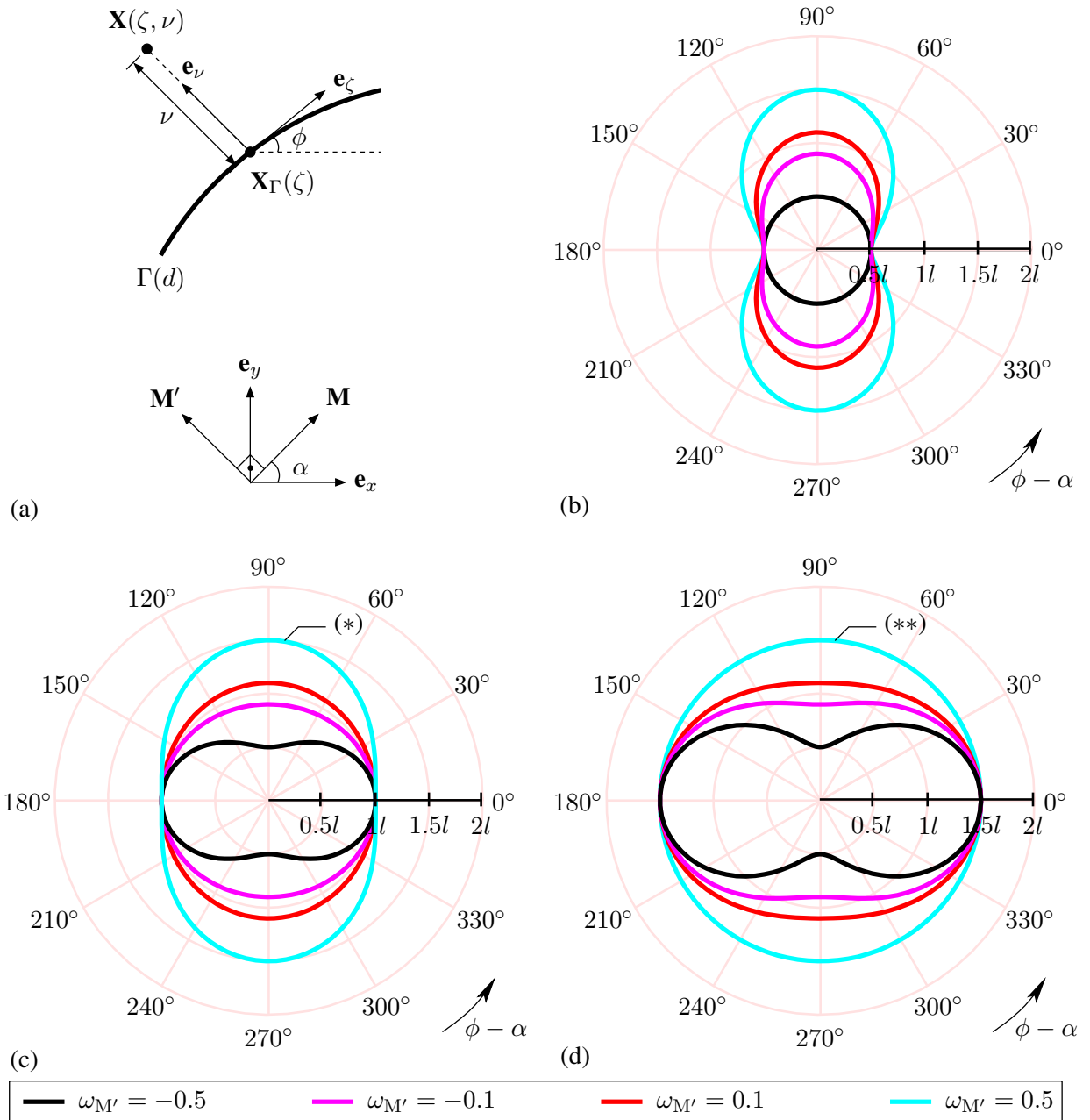
Figure 4: (a) Geometric profile of the sharp crack \Gamma \in \mathcal{B} at point \mathbf{X}_\Gamma(\zeta) together with the global and local coordinates systems (x, y) and (\zeta, \nu) , respectively. Polar plots of the effective length scale parameter l_e(\phi, \alpha) shown for an orthotropic case ( \mathbf{M} \perp \mathbf{M}' ) in (17), with the anisotropy parameter (b) \omega_M = -0.5 ; (c) \omega_M = 0.0 ; (d) \omega_M = 0.5 . The values assumed by the other anisotropy parameter \omega_{M'} are shown in color (see the legend).
