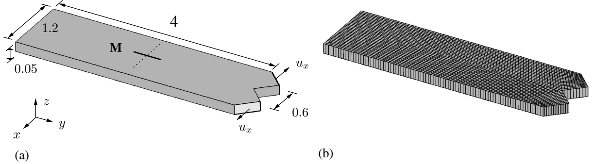
Figure 12: (a) Geometry of the strip with a single family of fibers with orientation \mathbf{M} in the y -direction, corresponding to the collagenous component of the material. The strip is torn apart by means of a displacement u_x applied at the two arms in the positive and negative x -direction; (b) finite element mesh of the corresponding geometry. Dimensions are provided in millimeters.
