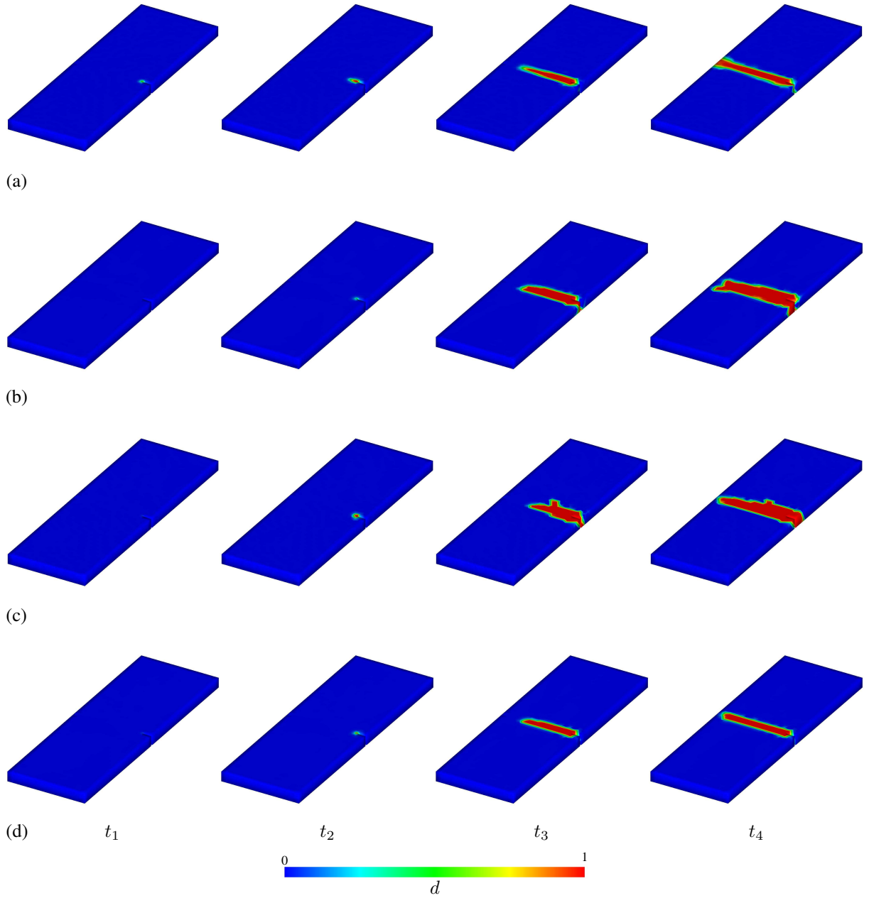
Figure 10: Evolution of the crack phase-field d in a notched strip of a hypothetical tissue uniaxially elongated: (a) energy-based criterion; (b) Tsai-Wu criterion; (c) principal stress criterion; (d) Hill criterion. The particular instants t_1, t_2, t_3 and t_4 manifest snapshots, compare with Figure 11.
