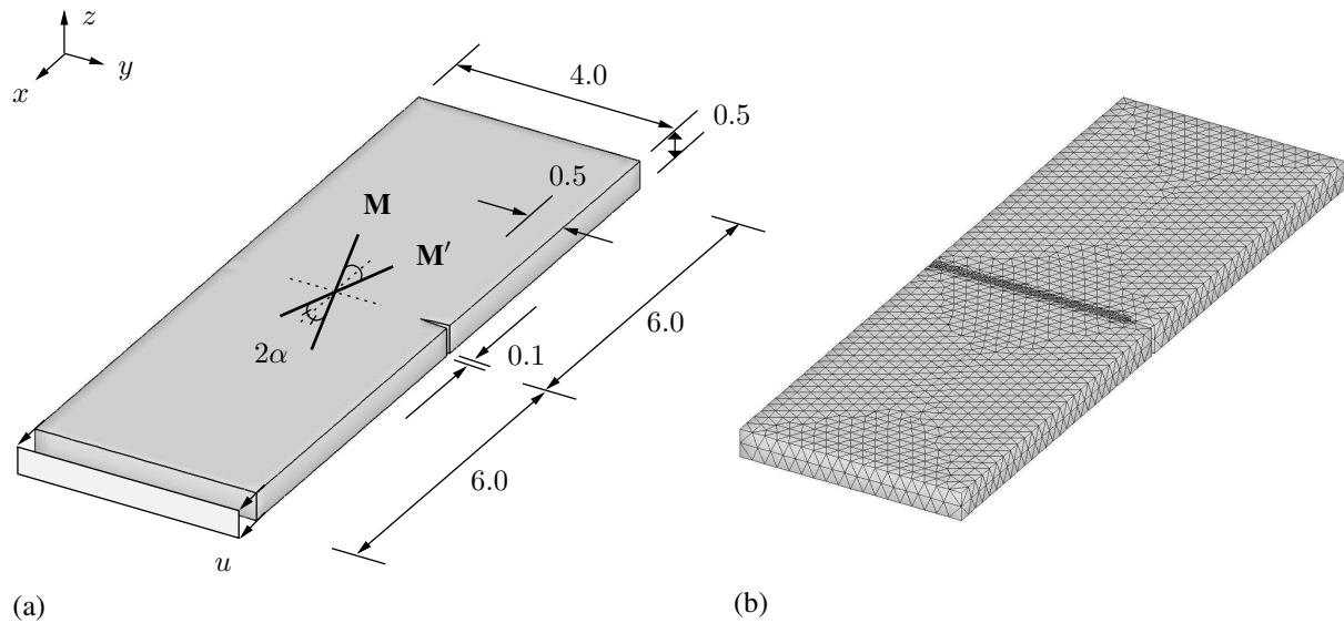
Figure 9: (a) Geometry of the strip with two families of fibers oriented in the directions \mathbf{M} and \mathbf{M}' and symmetrically arranged with respect to the x -axis by an angle \alpha . The strip is uniaxially loaded by means of a displacement u ; (b) finite element mesh of the corresponding geometry with refinement beyond the notch. Dimensions are provided in millimeters.
