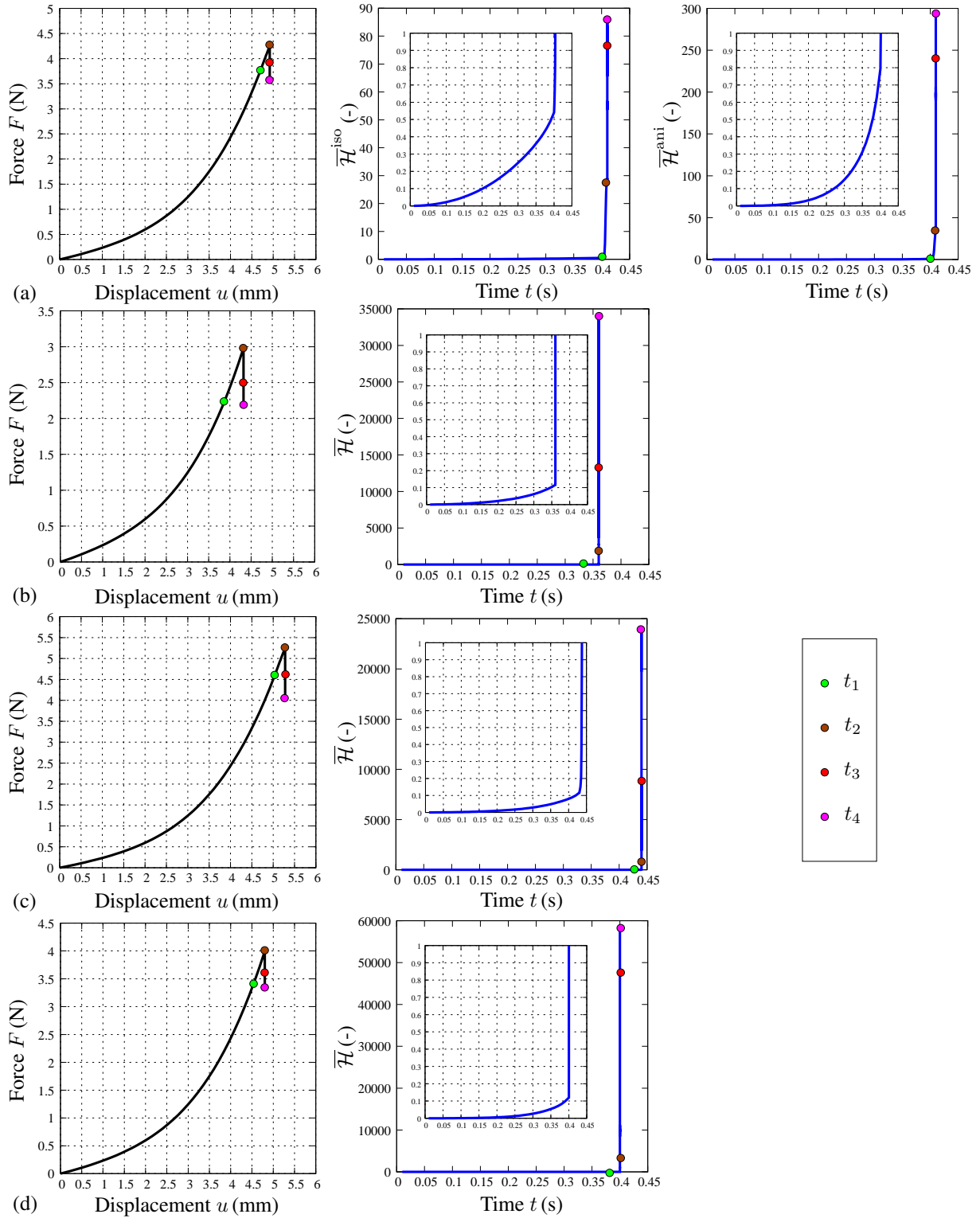
Figure 11: Plots corresponding to force F vs displacement u and to crack driving force \bar{\mathcal{H}} vs time t , with regard to (a) energy-based criterion; (b) Tsai-Wu criterion; (c) principal stress criterion; (d) Hill criterion. The particular instants t_1, t_2, t_3 and t_4 manifest the snapshots in the previous figure (Figure 10), and are also indicated here on curves. Zoom-in views for the \bar{\mathcal{H}}-t curves are also shown.
