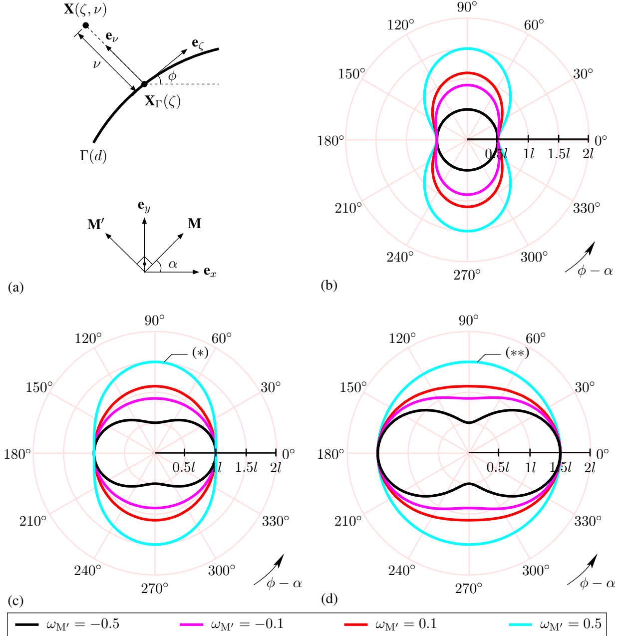
Figure 4: (a) Geometric profile of the sharp crack \Gamma \in \mathcal{B} at point \mathbf{X}_\Gamma(\zeta) together with the global and local coordinates systems (x, y) and (\zeta, \nu) , respectively. Polar plots of the effective length scale parameter l_e(\phi, \alpha) shown for an orthotropic case ( \mathbf{M} \perp \mathbf{M}' ) in (17), with the anisotropy parameter (b) \omega_M = -0.5 ; (c) \omega_M = 0.0 ; (d) \omega_M = 0.5 . The values assumed by the other anisotropy parameter \omega_{M'} are shown in color (see the legend).
