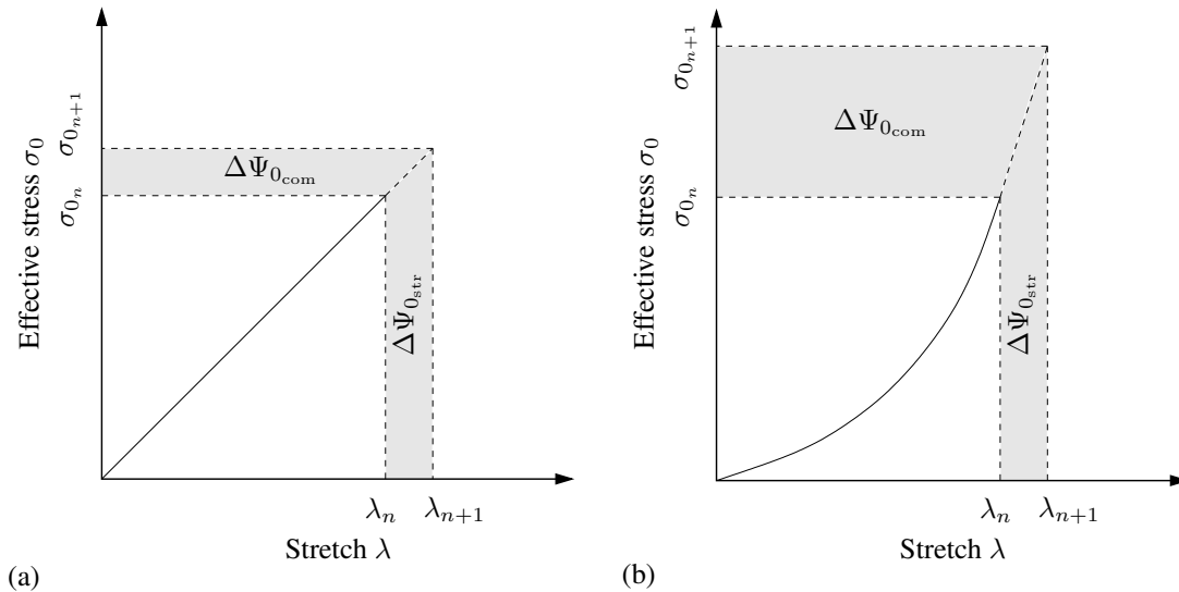
Figure 15: Qualitative sketch showing the relationship between the effective stress \sigma_0 and stretch \lambda , and the incremental change from \sigma_{0n}-\lambda_n to \sigma_{0n+1}-\lambda_{n+1} at a typical time step \Delta t = t_{n+1} - t_n : (a) linear; (b) nonlinear material behavior with the corresponding changes in the effective complementary energy \Delta\Psi_{0com} and the effective strain energy \Delta\Psi_{0str} .
