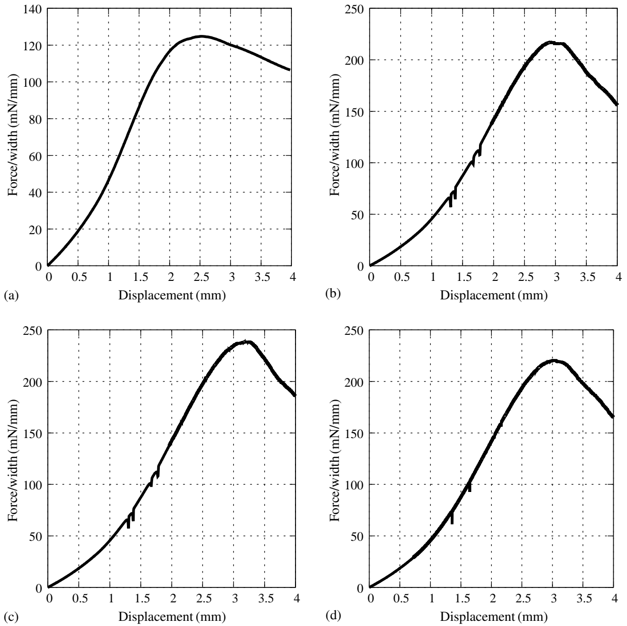
Figure 14: Plots of force per unit width for one arm against the applied displacement for (a) the energy-based; (b) the Tsai-Wu; (c) the principal stress criterion; (d) the Hill criterion.
