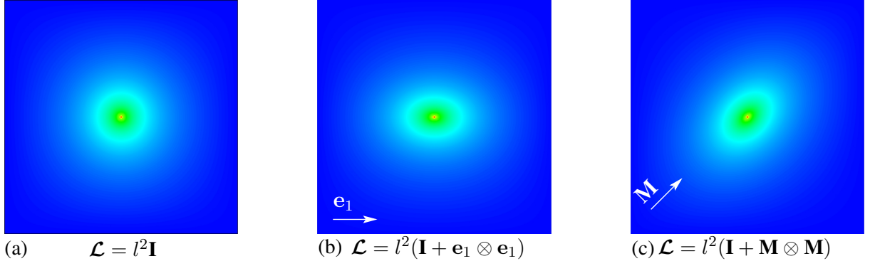
Figure 3: (a) Isotropic damage field; (b) anisotropic damage field with fiber angle \alpha = 0^\circ ; (c) anisotropic damage field with \alpha = 45^\circ .
