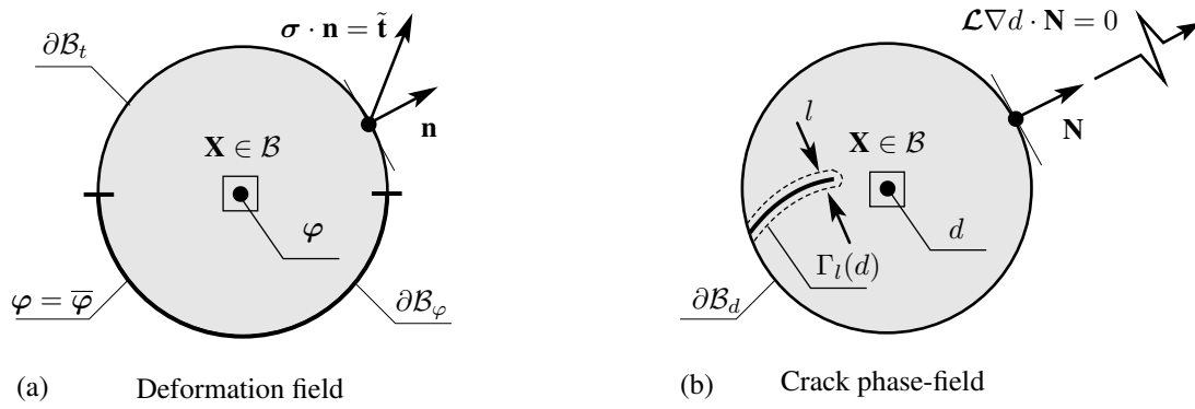
Figure 2: Multi-field problem: (a) mechanical problem of deformation along with Dirichlet and Neumann-type boundary conditions actualized by \varphi = \bar{\varphi} and the Cauchy theorem \boldsymbol{\sigma} \cdot \mathbf{n} = \tilde{\mathbf{t}} , respectively; (b) evolution of the crack phase-field problem with the Neumann-type boundary condition \mathcal{L}\nabla d \cdot \mathbf{N} = 0 .
