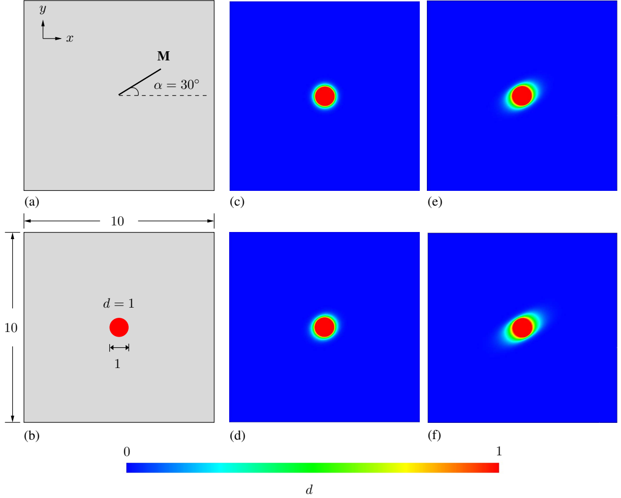
Figure 6: (a) 2-D square domain with one family of fibers oriented with an angle of \alpha = 30^\circ with respect to the x -axis; (b) geometry of the domain and boundary condition delineating a disc, where d = 1 . Evolution of the phase-field parameter d for a varying anisotropy parameter \omega_M : (c) 0; (d) 1; (e) 5, (f) 10. Dimensions are provided in millimeters.
