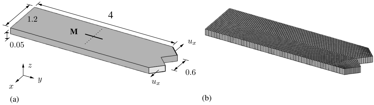
Figure 12: (a) Geometry of the strip with a single family of fibers with orientation \mathbf{M} in the y -direction, corresponding to the collagenous component of the material. The strip is torn apart by means of a displacement u_x applied at the two arms in the positive and negative x -direction; (b) finite element mesh of the corresponding geometry. Dimensions are provided in millimeters.
