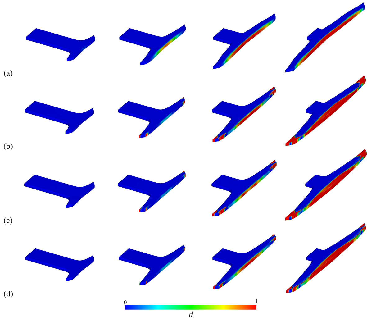
Figure 13: Evolution of the crack phase-field d for (a) the energy-based; (b) the Tsai-Wu; (c) the principal stress criterion; (d) the Hill criterion, as the arterial tissue with an initial tear is being pulled in two opposite directions.
