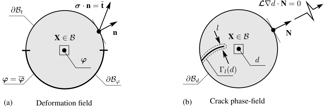
Figure 2: Multi-field problem: (a) mechanical problem of deformation along with Dirichlet and Neumann-type boundary conditions actualized by \varphi = \bar{\varphi} and the Cauchy theorem \boldsymbol{\sigma} \cdot \mathbf{n} = \tilde{\mathbf{t}} , respectively; (b) evolution of the crack phase-field problem with the Neumann-type boundary condition \mathcal{L}\nabla d \cdot \mathbf{N} = 0 .
