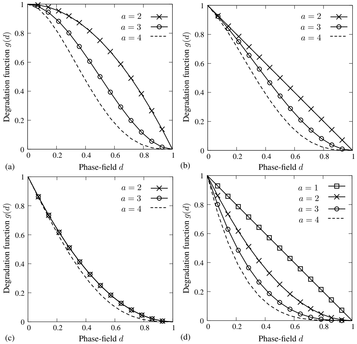
Figure 5: Qualitative behavior of the degradation function g(d) vs d : (a) b = 0 ; (b) b = 1 ; (c) b = 2 , according to (R2.1), while for (R2.2) g(d) is stated in (d).
