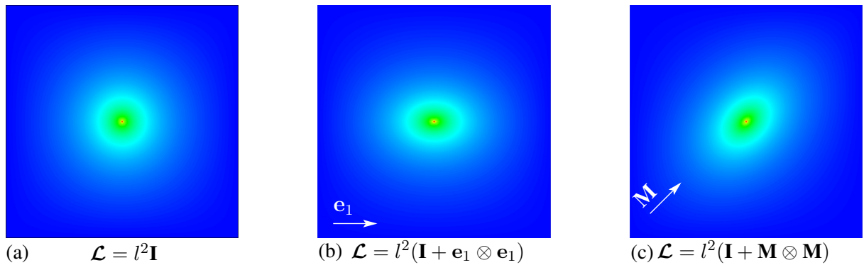
Figure 3: (a) Isotropic damage field; (b) anisotropic damage field with fiber angle \alpha = 0^\circ ; (c) anisotropic damage field with \alpha = 45^\circ .
