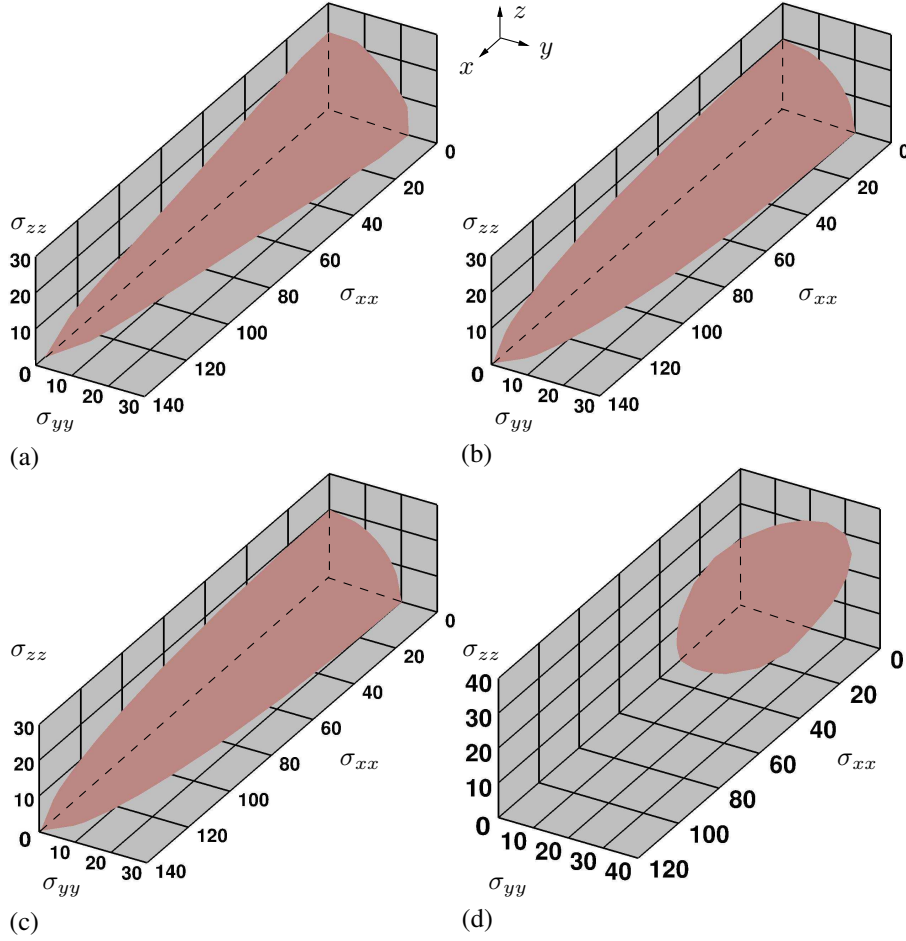
Figure 8: Failure surfaces in regard to Cauchy stresses \sigma_{xx} , \sigma_{yy} and \sigma_{zz} in kPa at which the failure conditions are satisfied, leading to d > 0 for (a) the energy-based; (b) the Tsai-Wu; (c) the maximum principal stress and (d) the Hill criterion.
