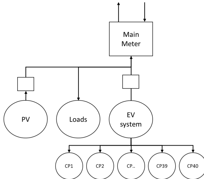
Figure 50. Illustration of pilot 2a in the Dutch pilot
