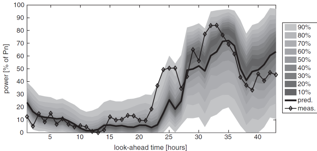
Figure 61. Forecasting of wind power production
