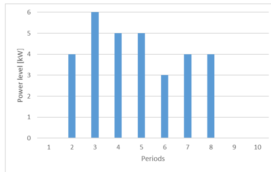
Figure 17. Consumption in case with shifting and shaping
