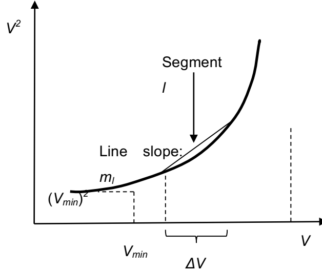
Figure 12. The piecewise linearization method [18]
