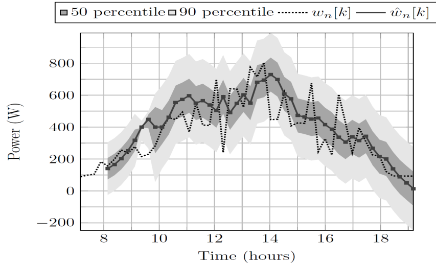
Figure 62. PV forecasting on a cloudy day
