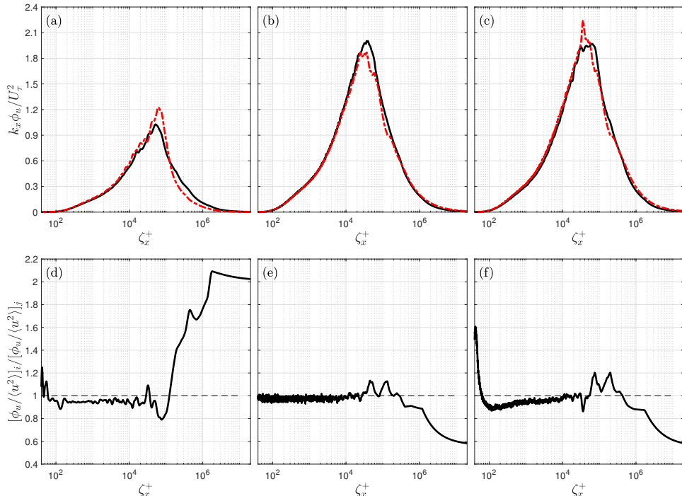
FIGURE 2. Pre-multiplied velocity spectra in the free-stream for cases (a) G and H, (b) K and M, and (c) N and O. (—) cases G, K, and N; (---) cases H, M, and O. The bottom panes (d), (e), and (f) show the ratio of the two curves presented in (a), (b) and (c), respectively; i represents the solid line and j represents the dashed line.
