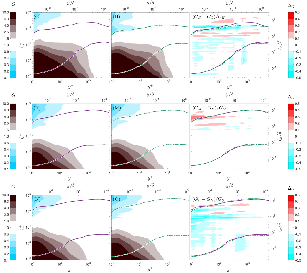
FIGURE 9. Contour plots of the gain of the pre-multiplied velocity spectra relative to the free-stream spectrum and the difference between the illustrated cases. Additional contour lines are drawn at a threshold of \phi^+ = 0.6 to identify the area in the plot that represents the most energy.
