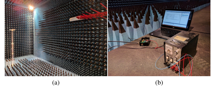
Fig. 4. Anechoic chamber test
