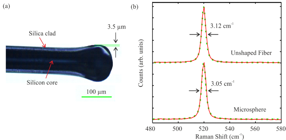
Fig. 1. (a) Microscope image of the hybrid microspherical resonator. (b) Raman spectrum of the polysilicon microspherical resonator core compared to that of the unshaped fiber core; solid lines are measured data, dotted curves are Voigt fits (Lorentzian linewidths as indicated).
