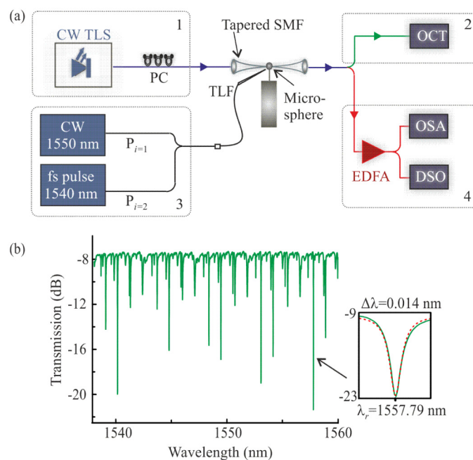
Fig. 2. (a) Set-up for characterizing the hybrid spherical resonators. Box 1 and 2 are used for the transmission measurements. Box 3 and 4 convert the set-up for the pump-probe experiments used to determine the nonlinear wavelength shifting for either a CW or pulsed pump. Polarization controller (PC), fiber amplifier (EDFA), tapered lens fiber (TLF), digital sampling oscilloscope (DSO), optical component tester (OCT). (b) Transmission spectrum. Inset: Lorentzian fit to determine Q_l .
