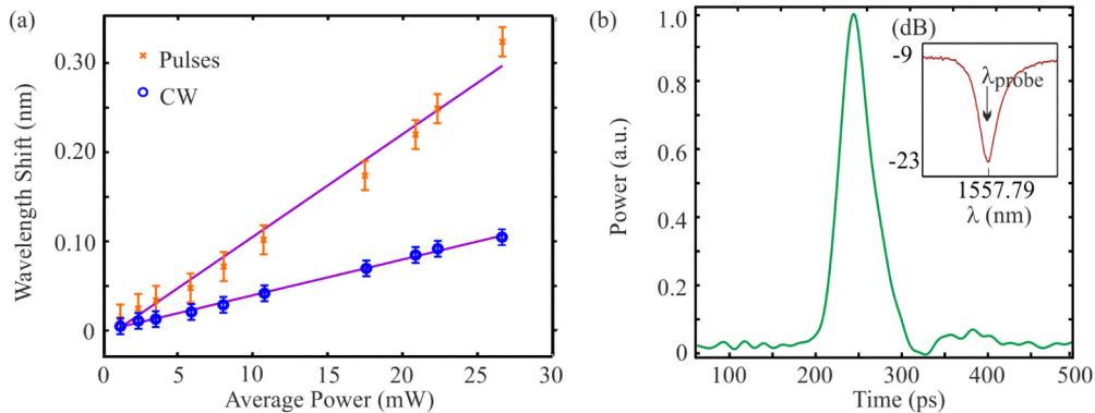
Fig. 3. (a) Wavelength shifting as a function of average power coupled into the TLF for CW and pulsed pumping. (b) All-optical switching of a CW probe induced by the pulsed pump. Inset: the CW probe position with respect to cold cavity resonance dip.
