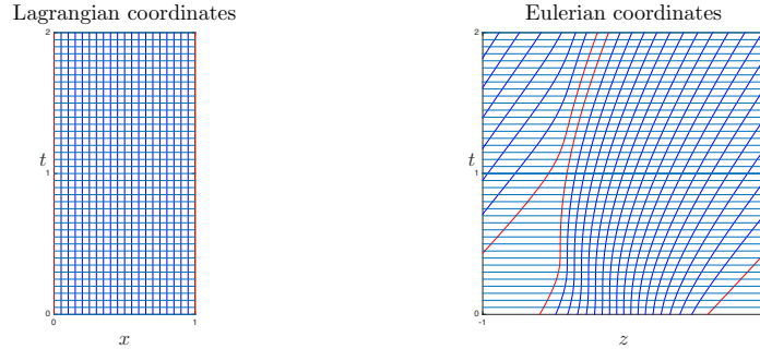
FIGURE 1. Left: the Lagrangian grid \{(t^n, x_{i-1/2})\}_{i=1}^N . Right: the Eulerian grid \{(t^n, z_{i-1/2}^n)\}_{i=1}^N . In both cases n = 0, \dots, 40 .
