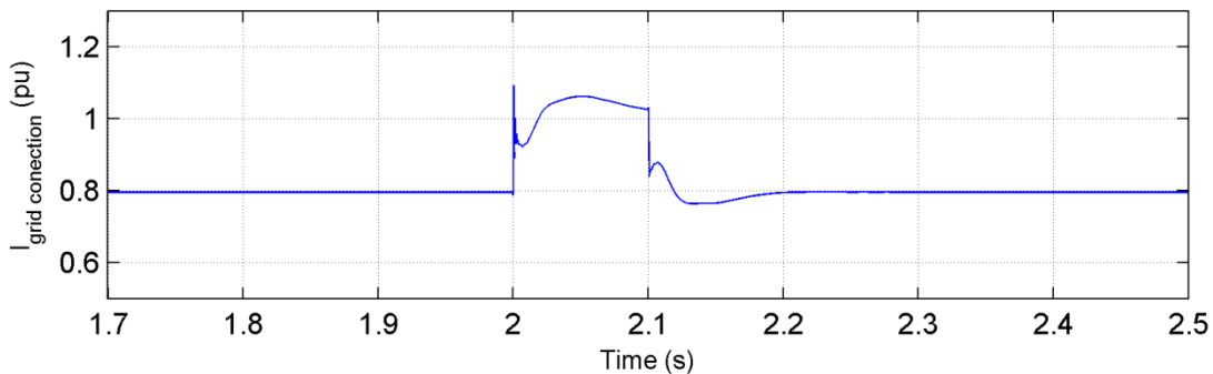
Fig. 5.19 RMS current from the onshore power grid to the onshore converter during a sag in the onshore voltage.
