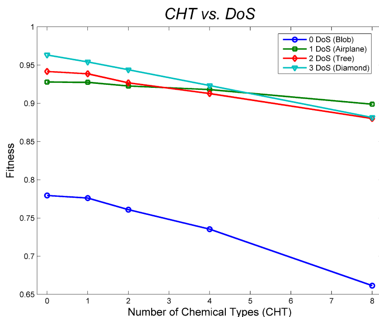
Figure 11.33: Fitness achieved using various numbers of chemical types (CHT) and degrees of symmetry (DoS)
