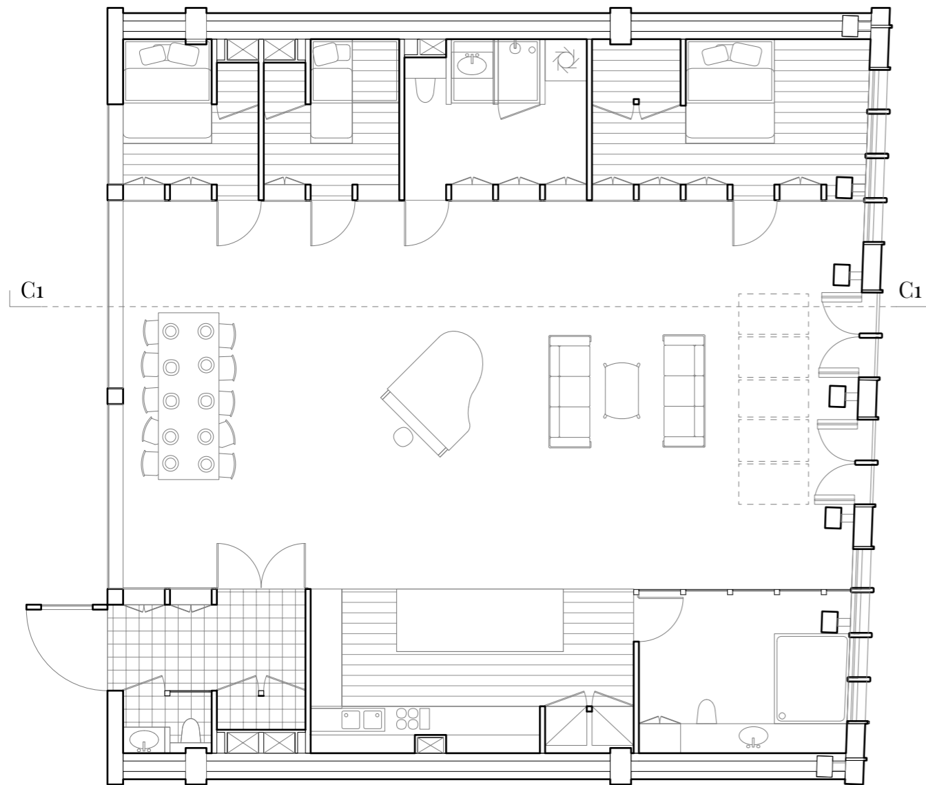
Plan 8, Leilighetstype 3
