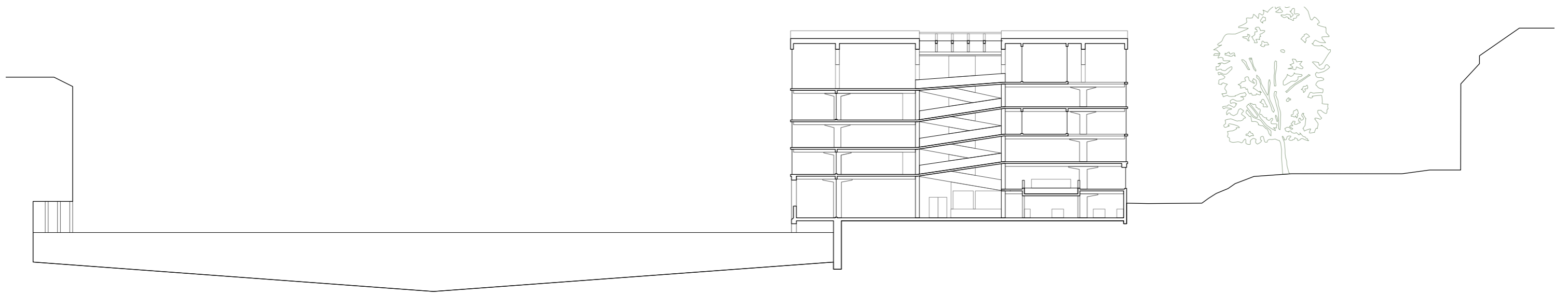
Snitt D - D, Restaurant brygge
