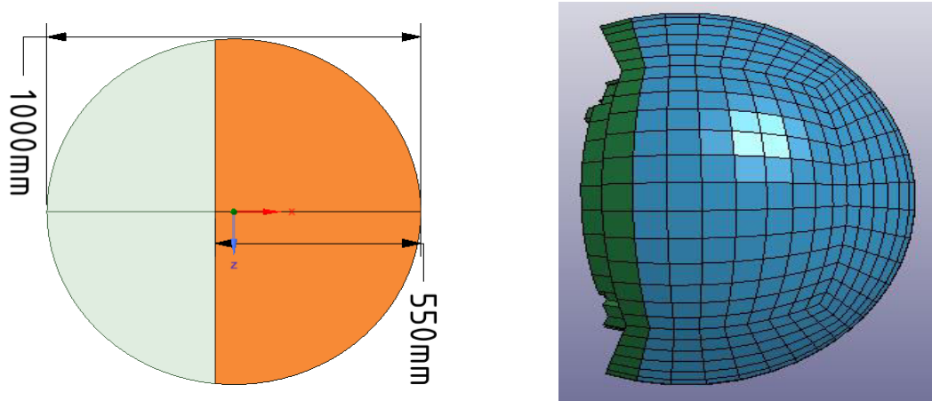
Figure 41 (a) sketch of the ice growler (b) ice model used in the crushing analysis in LS DYNA
