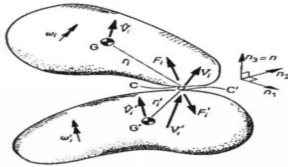
Figure 19 Free Body Diagram of two impacting bodies (21) (Liu 2011)
