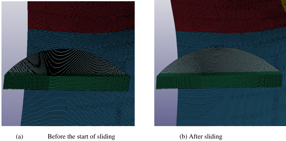
Figure 88 (a,b) presents two animation pictures before sliding starts and after the sliding for case 2
