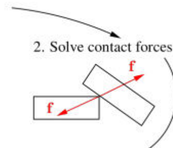
Figure 110 shows the second step in DEM where the forces that arise due to the contact between the particles are solved
