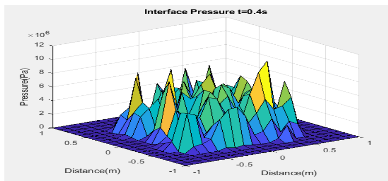
Figure 58 Local pressure pattern with visible peaks for rigid structure-ice floe interaction
