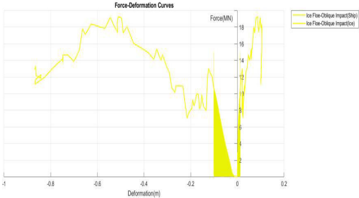
(c) Limited F-D curves based on EM output for the ice floe-oblique impact case
