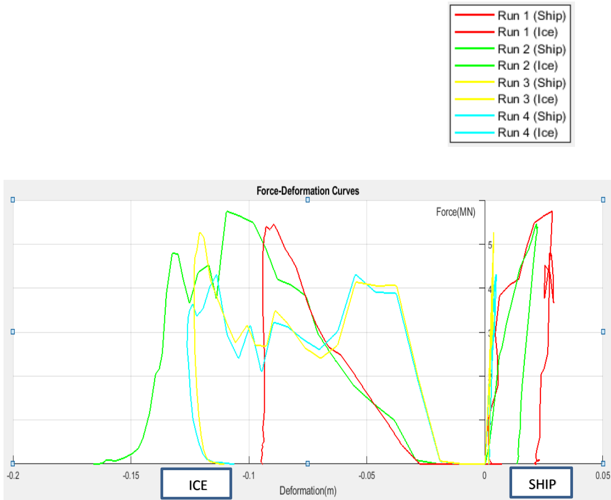
Figure 85 Force-deformation curves for different impact angles and frictional coefficient
