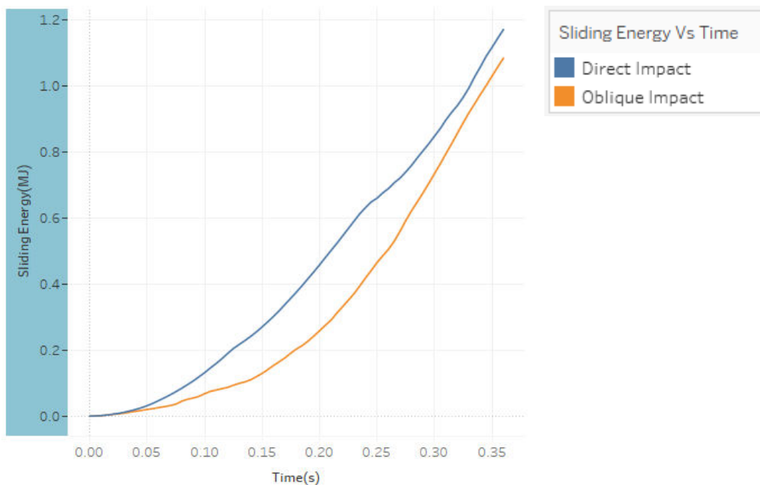
Figure 77 Plot showing the sliding energy as a function of time for direct and oblique ice floe impacts
