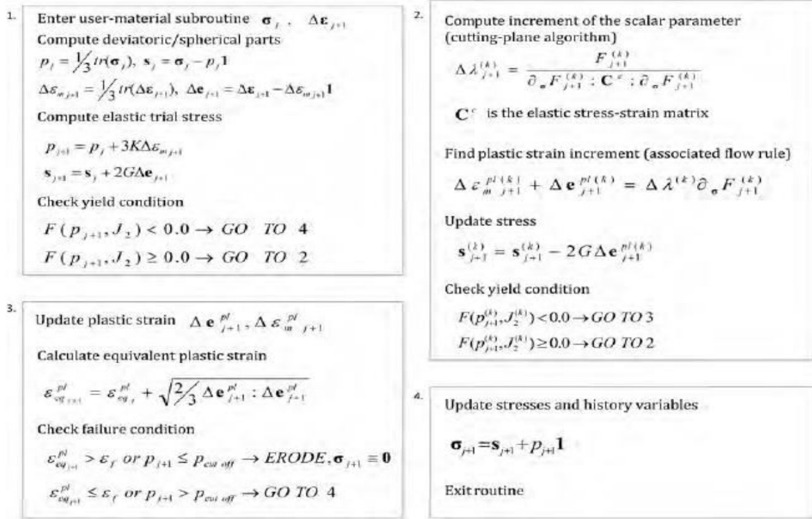
Figure 32 Flowchart showing the user defined algorithms for ice material model
