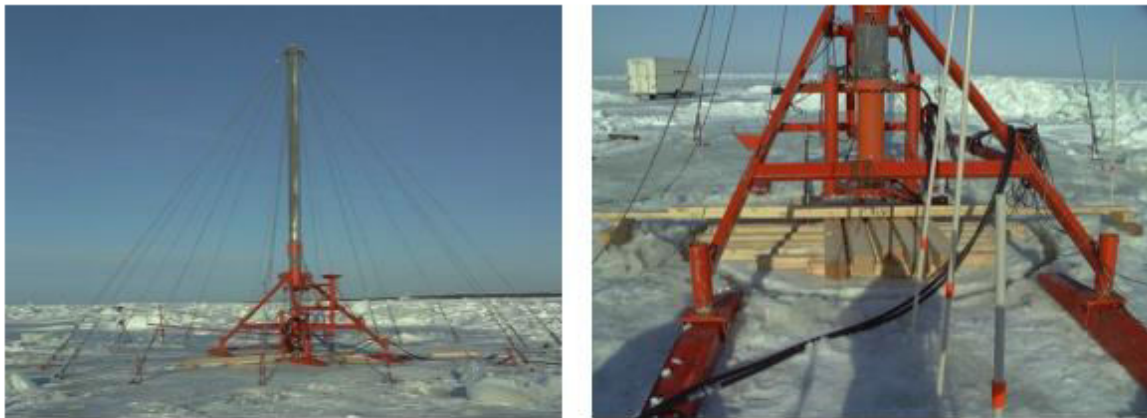
Figure 14 Picture showing the full scale tests on a ridge in Baltic sea (Tukhuri, Ice Mechanics-Ridges and Rubble piles 2016)
