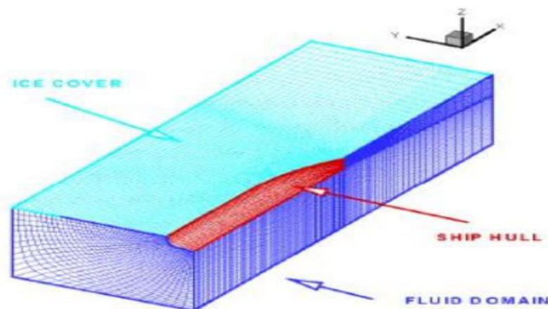
Figure 12 CFD simulation of ship in ice (Kujala, Winter Navigation-Ship resistance in ice 2016)
