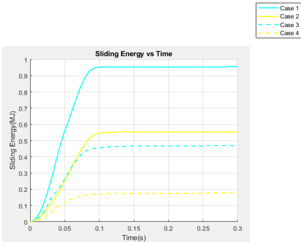
Figure 89 Plots showing sliding energy curves for all simulated cases as a function of time
