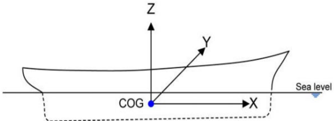
Figure 20 Global coordinate system axis of the ship (21) (Liu 2011)
