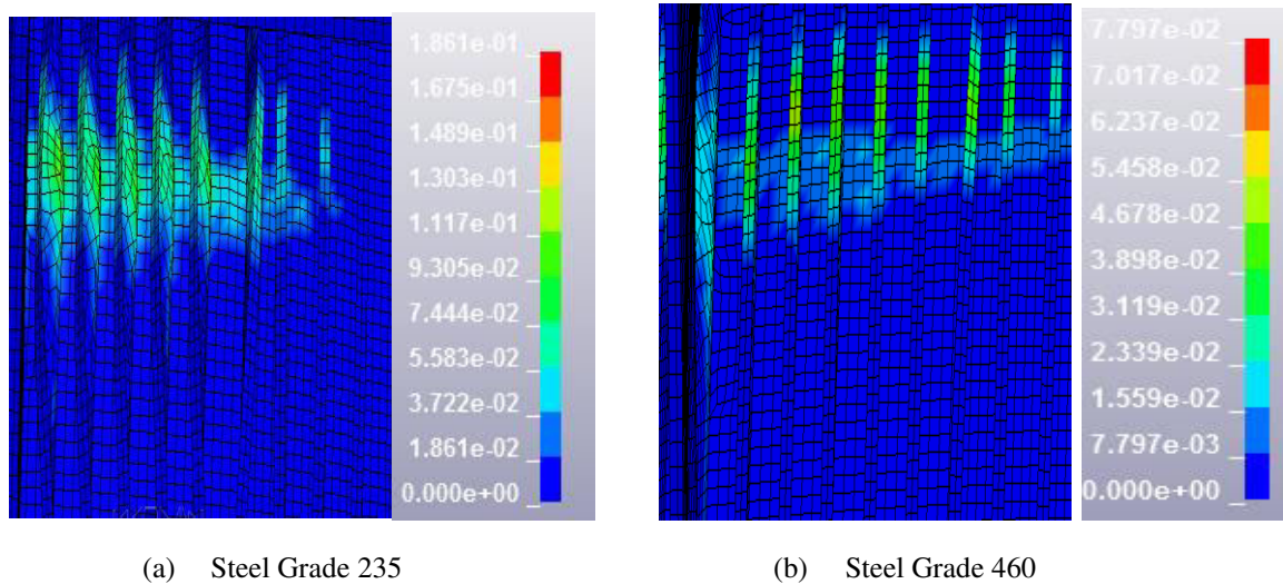
Figure 97 (a,b) shows effective plastic strain distribution for two steel grades S23 and S460
