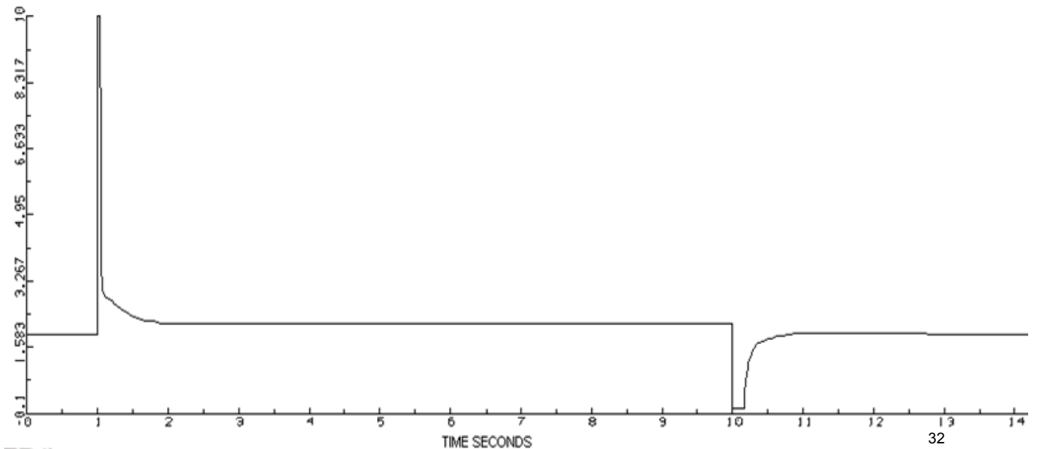
Figur 3: Tidsrespons for VR, feltspenning i feltgenerator opprinnelige PID innstillinger
