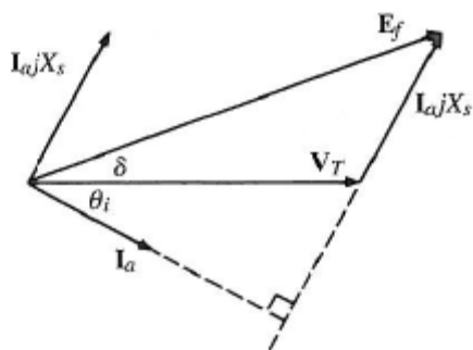
Figur 9: Viserdiagram for en synkrogenerator [12]
