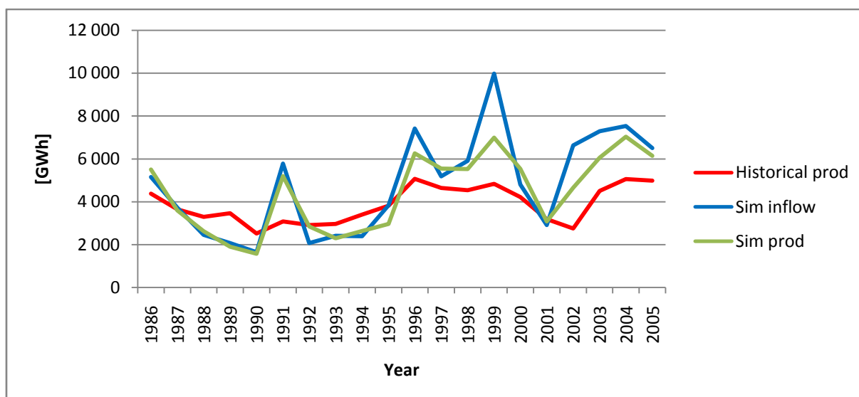
Figure 22 Comparing historical production with simulated production and inflow
