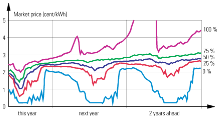
Figure 2 Example of price forecast from the EMPS model (SINTEF, EMPS, 2008)
