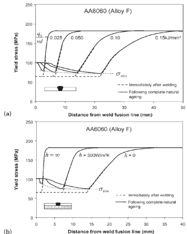
a effect of applied heat input q_0/vd on HAZ yield strength distribution for h=0 (adiabatic surfaces – no heat loss to surroundings); b effect of heat transfer coefficient h on HAZ yield strength distribution for q_0/vd=0.1 kJ mm -2
