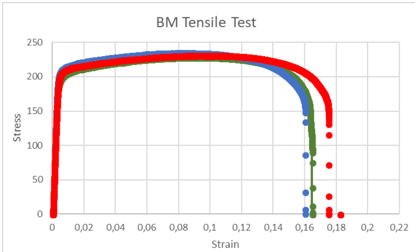
Fig.67 Stress-Strain curve of the BM
