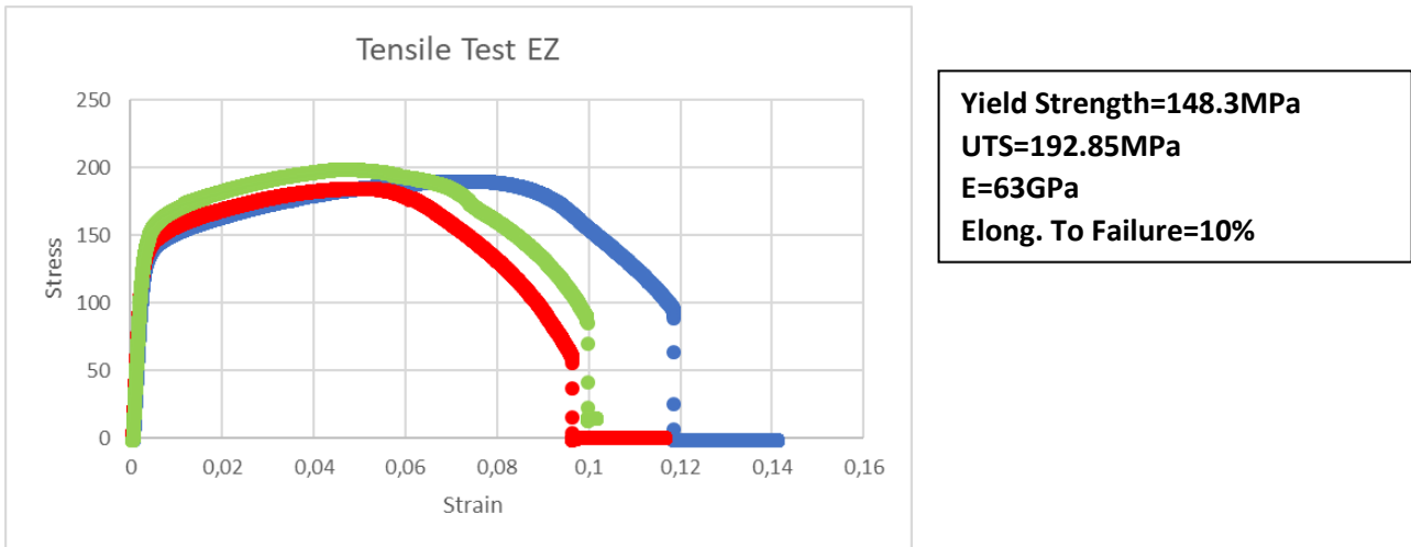
Fig.69 stress-strain extrusion zone EZ
