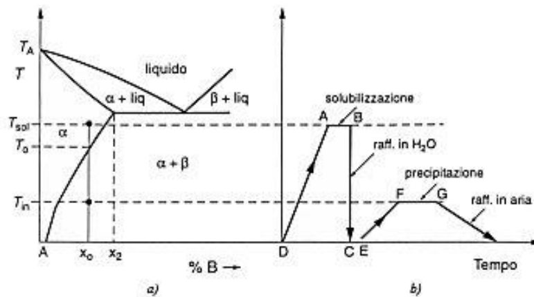
Fig.15 Heat treatment T6
