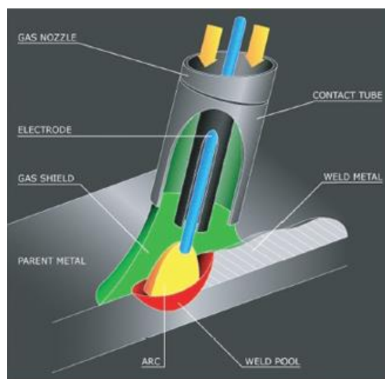
Fig.14 Gas metal arc welding
