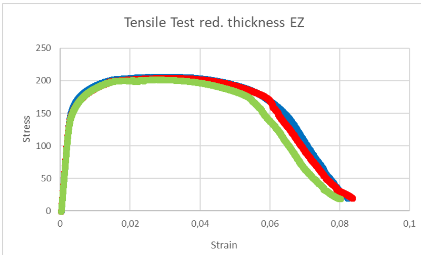
Fig.71 tensile test reduce thickness EZ
