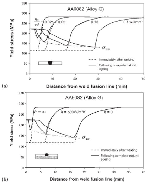
a effect of applied heat input q_0/vd on HAZ yield strength distribution for h=0 (adiabatic surfaces – no heat loss to surroundings); b effect of heat transfer coefficient h on HAZ yield strength distribution for q_0/vd=0.1 kJ mm -2 .
