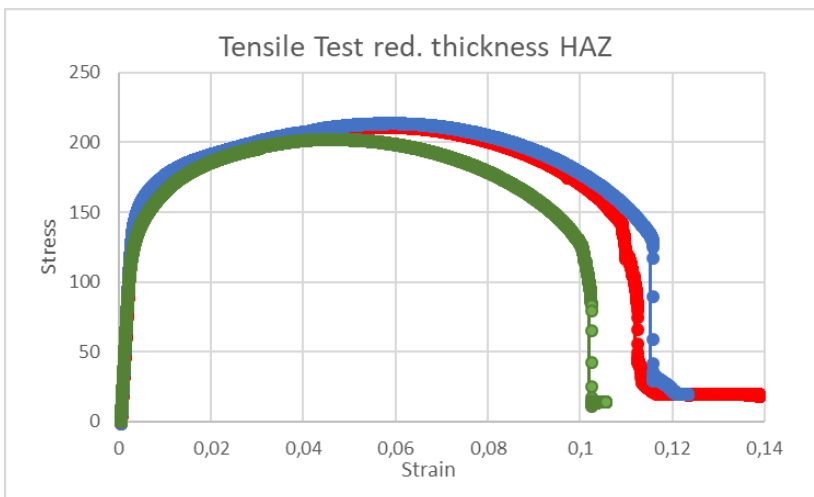
Fig.72 Tensile test reduce thickness HAZ
