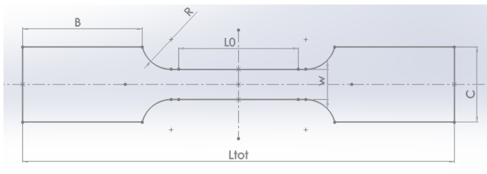
Fig.34 dogbone specimen
