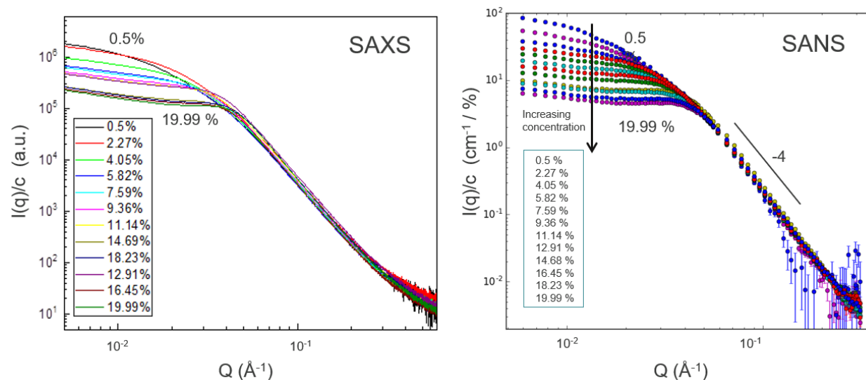
Fig.8. SAXS and SANS intensities normalized to concentration of MNPs ( \text{Fe}_3\text{O}_4/\text{CA} ) with varying concentration. The SANS data have been background-subtracted for the \text{H}_2\text{O} contribution.
