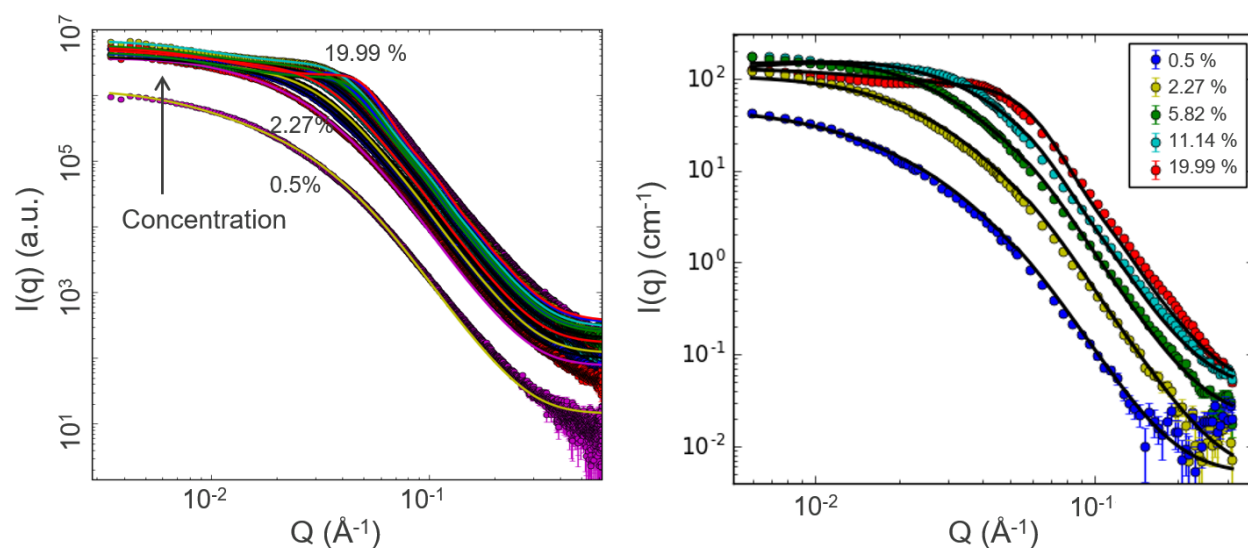
Fig. 9. SAXS (left) and SANS data (right) of \text{Fe}_3\text{O}_4/\text{CA} magnetic fluids with fits (continuous lines) using a core-shell ellipsoidal model and a screened Coulomb interaction potential. Only selected concentrations are shown for the SANS data in order to better appreciate the difference between the curves with increasing concentration.
