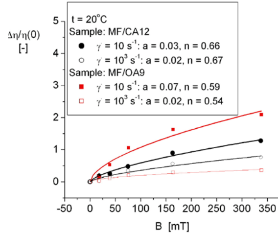
Fig.16 b. Magnetoviscous effect: dependence on magnetic induction at \dot{\gamma} = 10\text{s}^{-1} and at \dot{\gamma} = 10^3\text{s}^{-1} .
