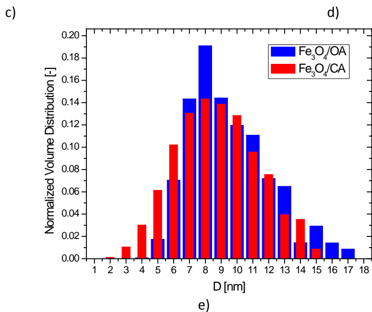
Fig.2. TEM images and nanoparticle diameter histograms for: a) and b) Fe 3 O 4 /CA; c) and d) Fe 3 O 4 /OA samples; e) normalized volume distributions.
