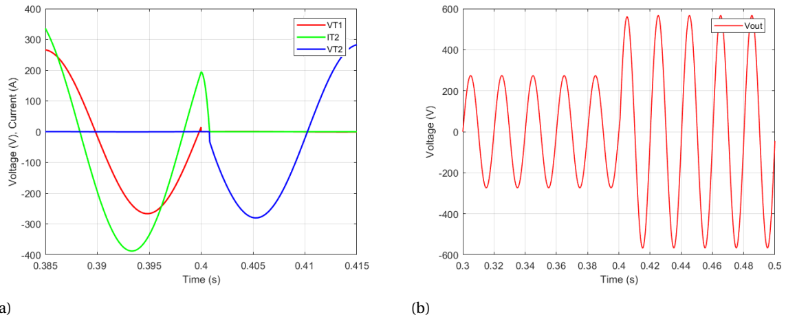
Figure 6.18: Simulation results at capacitive power factor angle of 30^\circ for switching up operation (a) Thyristor voltages V_{T1} , V_{T2} and thyristor current I_{T2} (b) Tap output voltage ( V_o )
