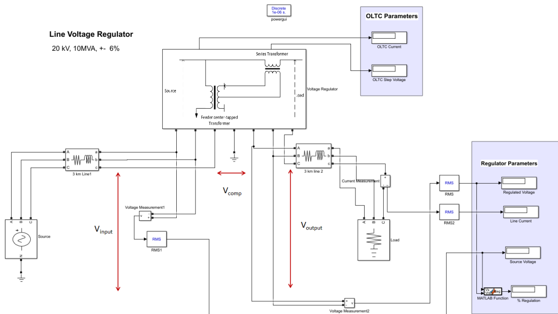
Figure 6.19: MATLAB/ Simulink model of a LVR with thyristor based OLTC in a MV distribution line
