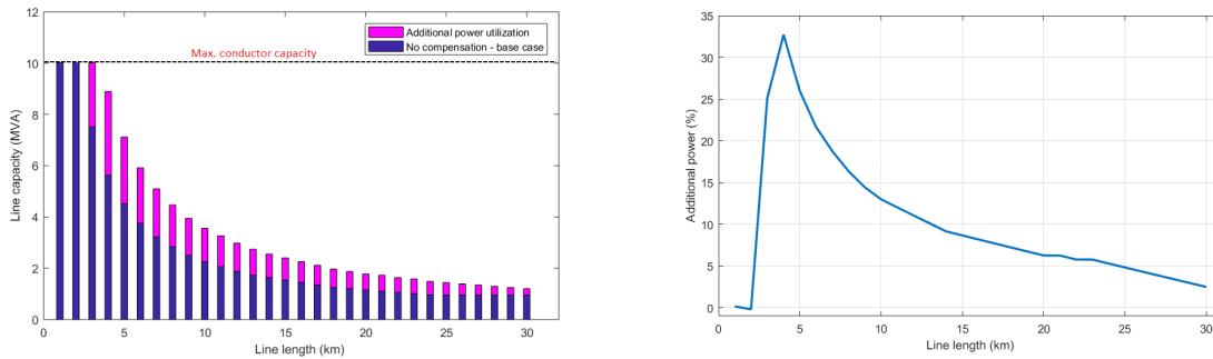
(a) (b) Figure 3.20: (a) Line capacity (MVA) vs line length (km) for the generation scenario with A1_63 conductor (b) Percentage increase in the line capacity as a function of line length for the generation scenario with A1_63 conductor
