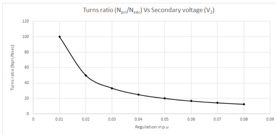
Figure 4.12: Turns ratio Vs Regulation voltage ( V_2 ) for OLTC on the primary side of the feeder transformer
