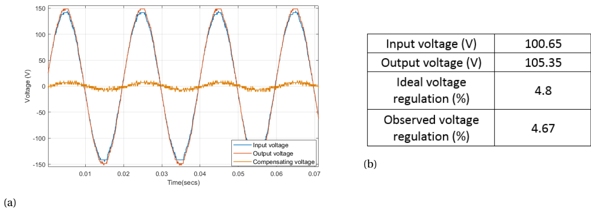
Figure 5.10: Experimental results for positive voltage regulation (a) Per-phase input, output and compensation voltage waveforms (b) Per-phase RMS input, output and compensation voltage values
