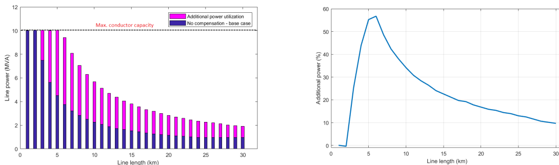
(a) (b) Figure 3.21: (a) Line capacity (MVA) vs line length (km) for the generation scenario with A1_100 conductor (b) Percentage increase in the line capacity as a function of line length for the generation scenario with A1_100 conductor
