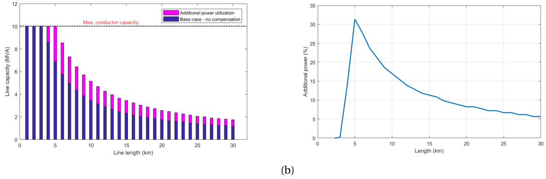
Figure 3.18: (a) Line capacity (MVA) vs line length (km) for the load scenario with A1_63 conductor (b) Percentage increase in the line capacity as a function of line length for the load scenario with A1_63 conductor
