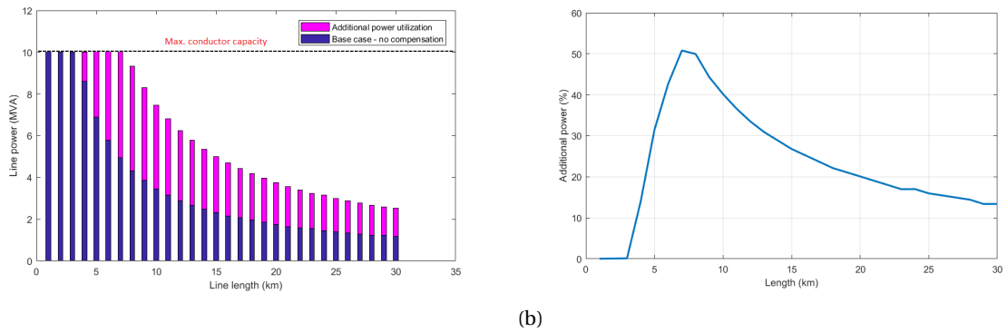
Figure 3.19: (a) Line capacity (MVA) vs line length (km) for the load scenario with A1_100 conductor (b) Percentage increase in the line capacity as a function of line length for the load scenario with A1_100 conductor
