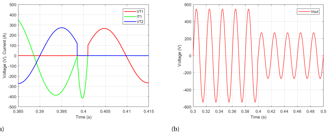
Figure 6.16: Simulation results at capacitive power factor angle of 24.8^\circ ( \phi_c ) for switching down operation (a) Thyristor voltages V_{T1} , V_{T2} and thyristor current I_{T1} (b) Tap output voltage ( V_o )
