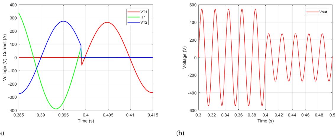
Figure 6.17: Simulation results at capacitive power factor angle of 30^\circ for switching down operation (a) Thyristor voltages V_{T1} , V_{T2} and thyristor current I_{T1} (b) Tap output voltage ( V_o )
