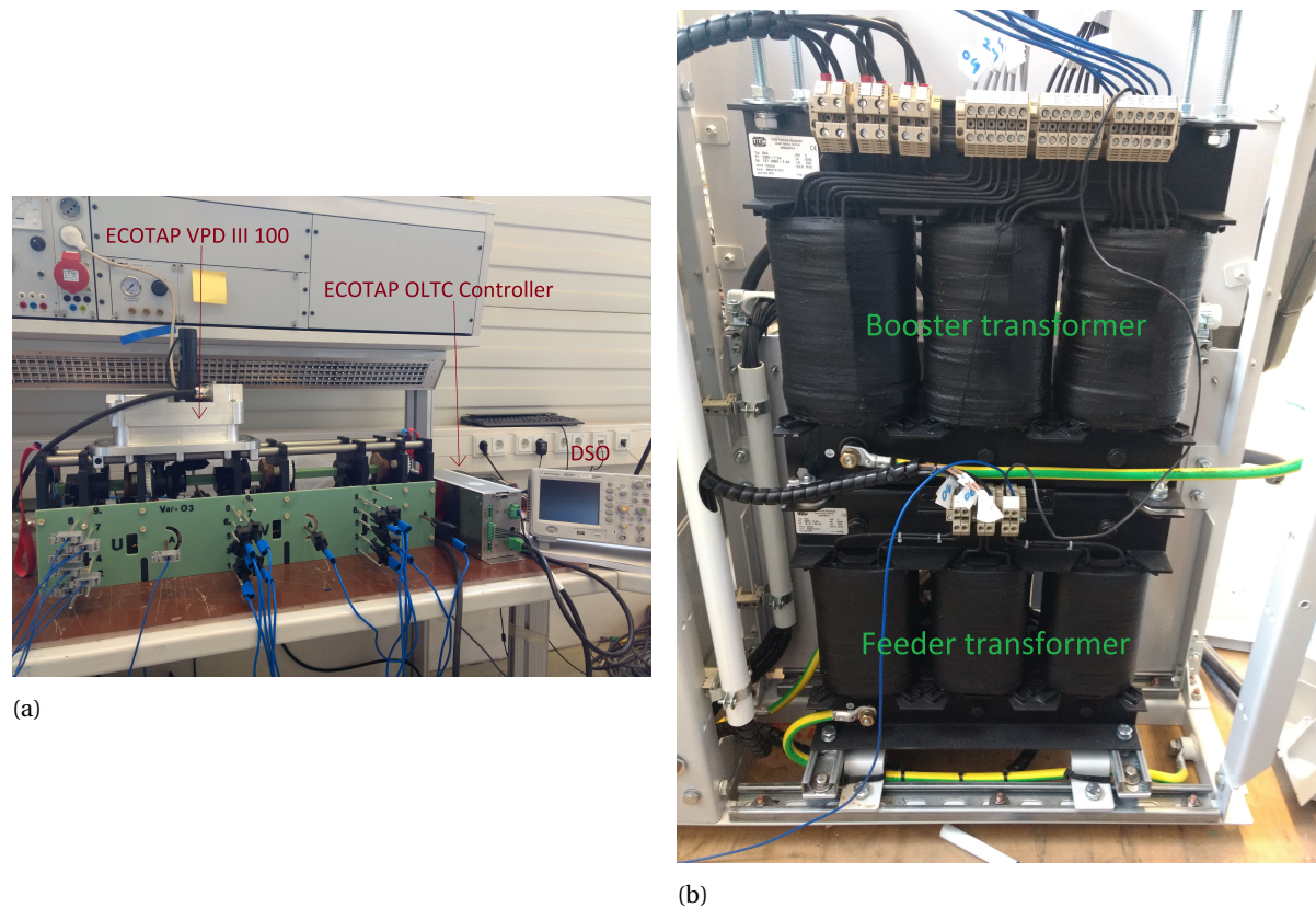
Figure 5.8: (a) MR ECOTAP OLTC(left), MR controller(center), DSO (right) (b) Feeder transformer (top), Booster transformer (bottom)
