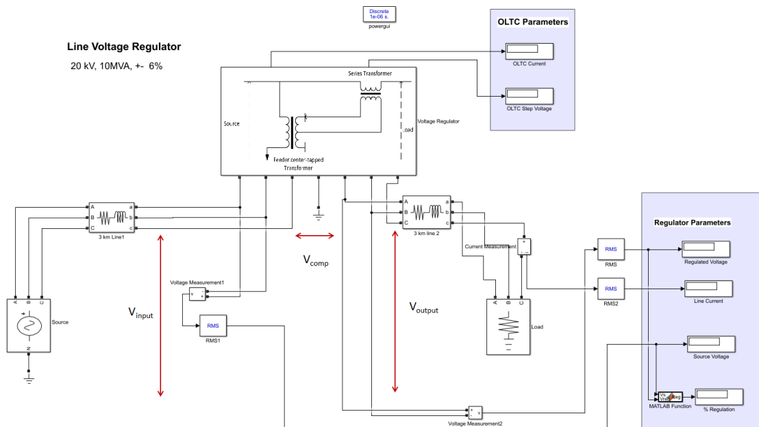
Figure 5.4: MATLAB/ Simulink model of a LVR in a MV distribution line
