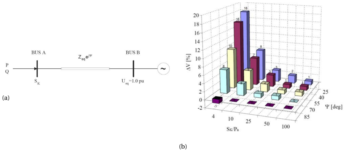
Figure 2.6: (a) A thevenin equivalent circuit for a wind farm (Bus A) connected to a grid (Bus B) (b) Voltage variation due to injected power P_n [70]
