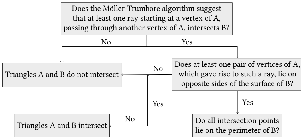
Figure 3.14: Flowchart illustrating the algorithm for detecting self-intersections. In order to ensure that no self-intersection went unnoticed, the indicated procedure was carried out by comparing each of the interpolation triangles A in the most recently computed level set, to all of the triangles B in the previously computed level sets. Provided that any of the new triangles intersected any of the old ones, the new level set as a whole was flagged as self-intersecting. How this intersection-detection approach handled a set of special cases is illustrated in figure 3.15.
