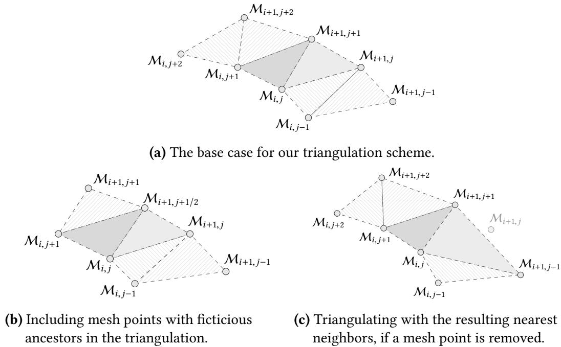
Figure 3.13: Conceptual illustrations of our triangulation algorithm. The standard approach, which applies when there is a one-to-one correspondence between the nearest neighbors of the point M_{i,j} in the level set \mathcal{M}_i , and the M_{i,j} 's nearest neighbors in the level set \mathcal{M}_{i+1} , is shown in (a). Meanwhile, (b) and (c) illustrate our handling of the special cases which arise when the one-to-one correspondence between points in subsequent level sets is broken. In particular, (b) shows how we include a mesh point inserted inbetween the points M_{i+1,j} and M_{i+1,j+1} in the triangulation, while (c) demonstrates how the removal of mesh point M_{i+1,j} affects the triangulation. Both of these kinds of adjustments were made in order to maintain the density of mesh points (cf. section 3.8.1). In all of the illustrations, the pair of triangles which arise when triangulating outwards from M_{i,j} , are shaded. The remaining triangles (patterned) originate from the triangulation of other points in level set \mathcal{M}_i . Note that the removal of bundles of mesh points in order to dampen the effect of numerical noise (which introduces bulges, as described in section 3.8.2) is treated analogously to the case of single missing points.
