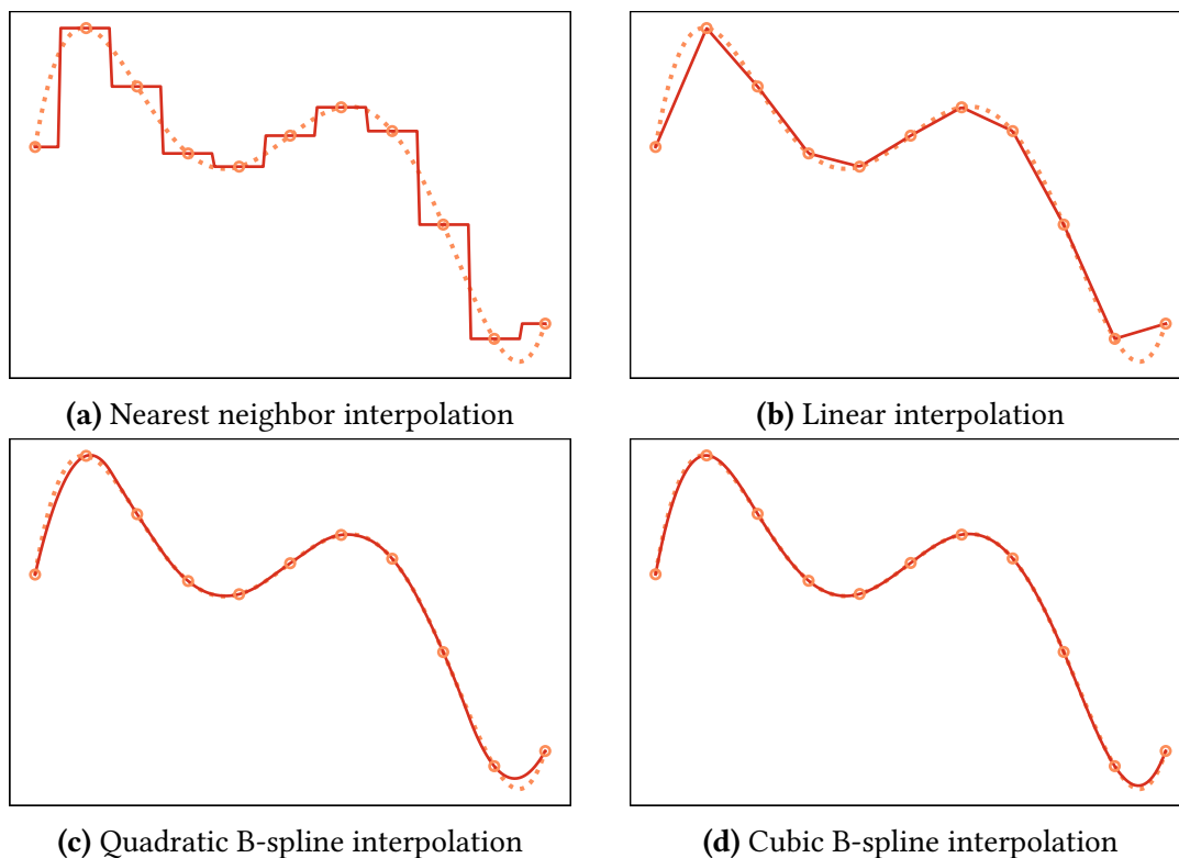
Figure 2.1: A selection of commonly used interpolation methods applied to a discretely sampled, high degree polynomial (dashed). The sampling points (knots) are shown as hollow circles. The splines in (c) and (d) are of second and third order, respectively (see definition 3). Observe how higher order splines yield increasingly accurate and smooth interpolations.
