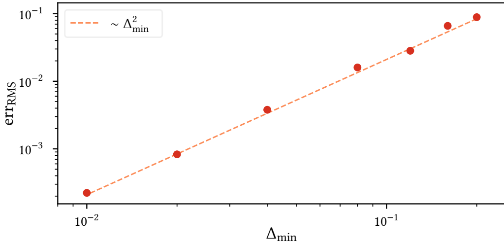
Figure 4.2: RMS error of geodesic level set approximations to an analytically known three-dimensional surface, as a function of mesh point density. Using seven different mesh point densities (here referred to by their \Delta_{\min} ), we computed approximations of the sinusoidal surface defined by equations (4.1) and (4.3) — four of which are shown in figure 4.1 — whose RMS error (as defined in equation (4.4)) are shown as solid dots. Note how the RMS error appears to increase quadratically as a function of \Delta_{\min} .
