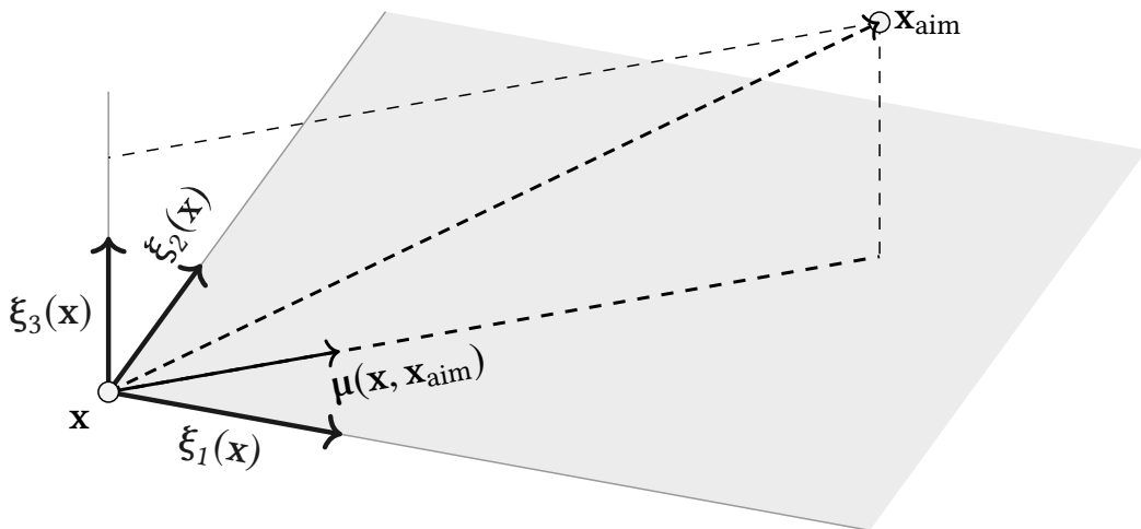
Figure 3.5: Visualization of the direction field used to compute trajectories within a manifold, using the legacy approach. The direction \boldsymbol{\mu}(\mathbf{x}, \mathbf{x}_{\text{aim}}) (see equation (3.17)) is found by normalizing the projection of \mathbf{x}_{\text{aim}} - \mathbf{x} into the plane spanned by the local \boldsymbol{\xi}_1 - and \boldsymbol{\xi}_2 vectors (shaded).
