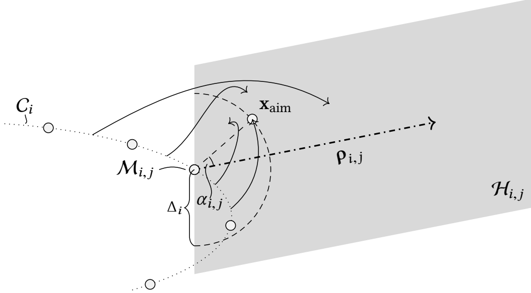
Figure 3.6: Visualization of typical trajectories used to compute a new mesh point, using the legacy approach. The aim point \mathbf{x}_{\text{aim}} is used to guide trajectories which are locally orthogonal to the \xi_3 direction field (cf. equation (3.17)) towards the intersection between the manifold \mathcal{M} and the half-plane \mathcal{H}_{i,j} (shaded), in order to find a new mesh point \mathcal{M}_{i+1,j} located a distance \Delta_i from \mathcal{M}_{i,j} . \mathcal{H}_{i,j} is defined by the point \mathbf{x}_{i,j} (that is, the coordinates corresponding to the mesh point \mathcal{M}_{i,j} ), its unit normal \mathbf{t}_{i,j} (not shown), and the (quasi-)radial unit vector \boldsymbol{\rho}_{i,j} (dashdotted). The half-circle of radius \Delta_i , centered in \mathbf{x}_{i,j} and laying within \mathcal{H}_{i,j} , on which we seek to find a new mesh point, is dashed. All permitted trajectory initial positions lie along the smooth parametrized curve C_i (dotted), and are given by equation (3.18). A select few trajectories are shown, where the arrowheads indicate the first intersection with \mathcal{H}_{i,j} (as per equation (3.19)), at which point the integration was terminated.
