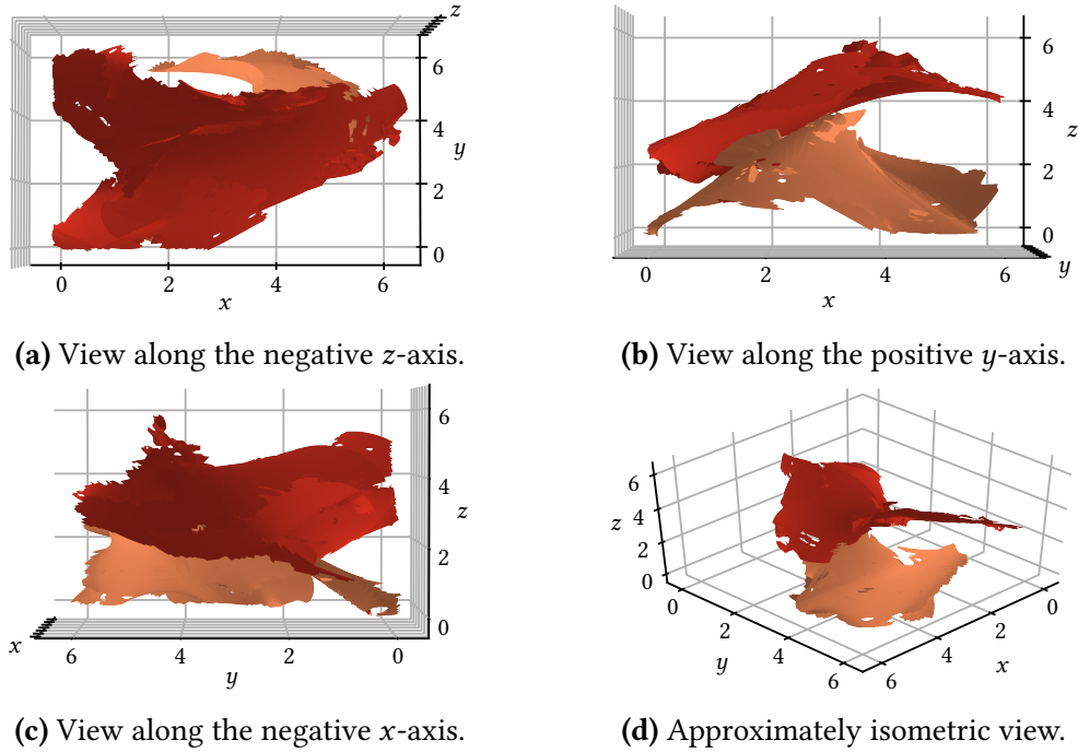
Figure 4.10: Four views of the repelling LCSs obtained for transport in the steady ABC flow, for the time interval \mathcal{I} = [0, 5] (see section 3.1.1). A total of 22 surfaces constitute two distinct, fairly smooth and coherent structures, which are shown in different colors. We provide four different viewing angles (the same as the ones used in figure 4.8, which shows the computed \mathcal{U}_0 domain), chosen in order convey the three-dimensional structures in as great detail as possible.
