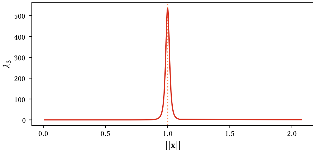
Figure 4.5: Arithmetic average of \lambda_3 across all solid angles, for the purely radial velocity field given by equation (4.5), using r = 1 . Note in particular the sharp repulsion peak at \|\mathbf{x}\| = 1 , which is a strong indicator for the presence of a repelling LCS.
