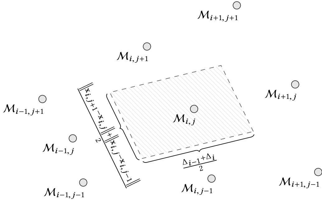
Figure 3.17: Our way of assigning weights to mesh points in computed LCSs. To a given LCS point \mathcal{L}_k , we assigned a weight given by a rectangular approximation of the surface area closer to the corresponding manifold mesh point \mathcal{M}_{i,j} than all other points in the parametrization of the manifold \mathcal{M} (patterned). Here, \Delta_i corresponds to the interstep length used to create level set \mathcal{M}_{i+1} , based on level set \mathcal{M}_i , (see section 3.7), while \mathbf{x}_{i,j} denotes the coordinates of mesh point \mathcal{M}_{i,j} .
