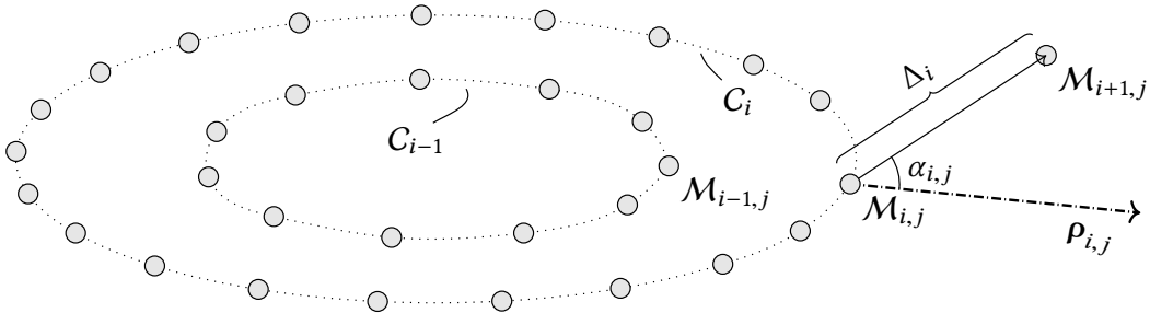
Figure 3.12: The principles of curvature-guided interset step length adjustment. For each of the mesh points \{\mathcal{M}_{i+1,j}\} constituting the level set \mathcal{M}_{i+1} which were computed from the mesh points constituting the most recently completed level set \mathcal{M}_i (i.e., all but the mesh points which were computed from fictitious ancestors, cf. section 3.8.1), the angular offsets \alpha_{i,j} between the guidance vectors \rho_{i,j} (dashdotted) and \rho_{i+1,j} (not shown, but parallel to the vector separating \mathcal{M}_{i,j} and \mathcal{M}_{i+1,j} , shown in solid) were computed. These were used in conjunction with \Delta_i , the interset step used to compute the new mesh points, in order to determine whether or not the suggested level set would have to be discarded due to the local curvature along at least one point strand being too large, according to criterion (3.28). If the level set was deemed acceptable, local curvature estimates \{\alpha_{i,j}\} and \{\Delta_i \cdot \alpha_{i,j}\} were then used to determine if the subsequent level set \mathcal{M}_{i+2} could be computed using \Delta_{i+1} > \Delta_i ; namely, if criterion (3.29) was satisfied.
