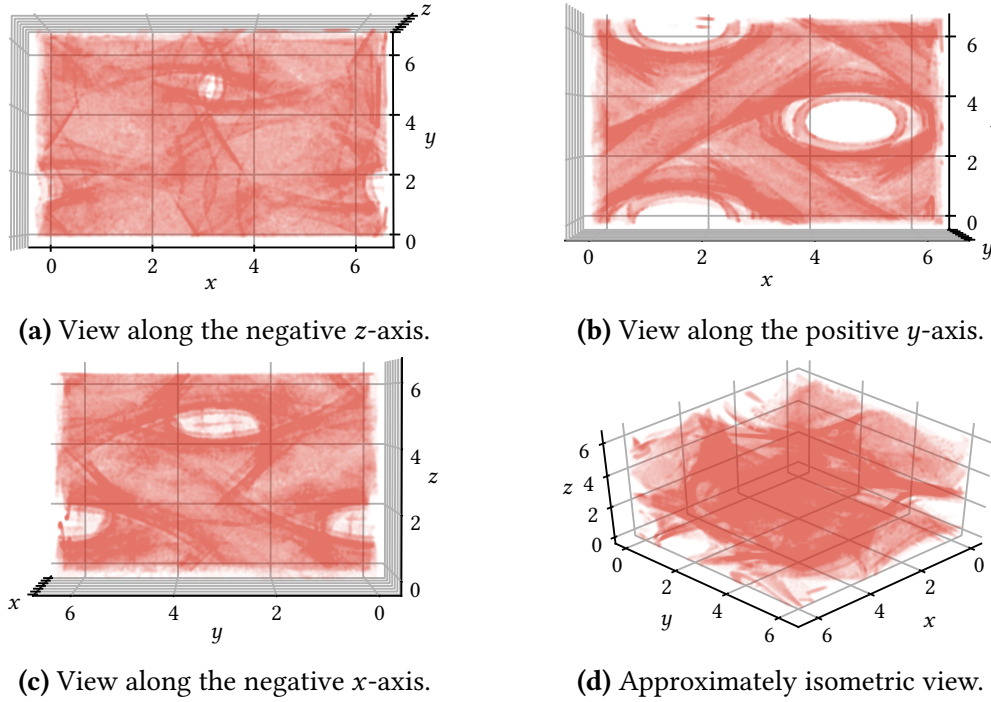
Figure 4.8: Four views of the \mathcal{U}_0 domain obtained for transport in the steady ABC flow, for the time interval \mathcal{I} = [0, 5] , identified as the grid points which satisfy the LCS criteria (2.28a), (2.28b) and (2.28d) (details on the implementation are available in section 3.5.1). In total, the domain consists of 340 951 different points (cf. table 3.2).
