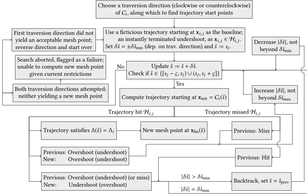
Figure 3.7: Flowchart illustrating the algorithm for iteratively choosing new trajectory start points based on the termination status of the preceding trajectories, using the legacy approach. All possible trajectory start points are contained within a subset of C_i , per equation (3.18). Whether or not a given trajectory intersected with the half-plane \mathcal{H}_{i,j} , and satisfied \Delta(\tilde{s}) = \Delta_i , was determined using equations (3.19) and (3.20).
