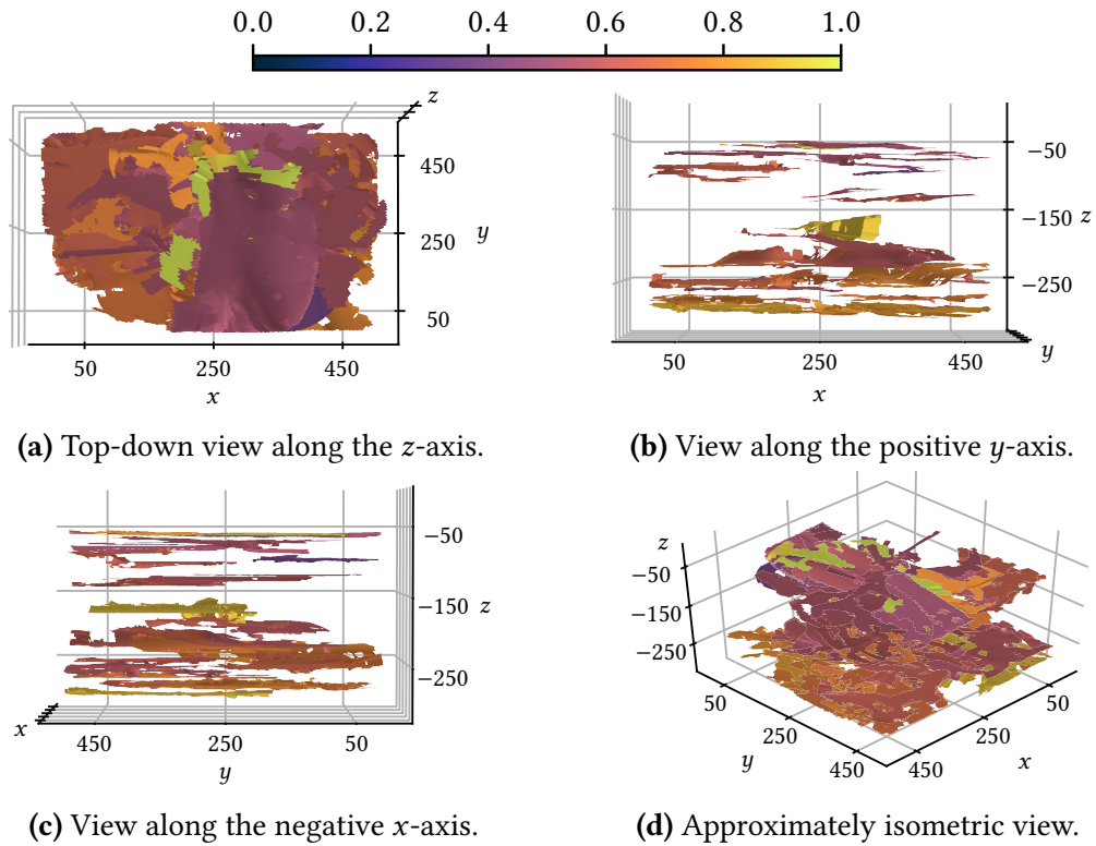
Figure 4.13: Four views of the repelling LCSs obtained for transport in the Førde fjord, over a time interval of 12 hours (see section 3.2). A total of 110 distinct surfaces are shown, which are colored according to their relative repulsion averages (per equation (4.6)) using the perceptually uniform colormap shown at the top. We provide four different viewing angles (the same as the ones used in figure 4.12, which shows the computed \mathcal{U}_0 domain), chosen in order to convey the three-dimensional structures in as great detail as possible.
