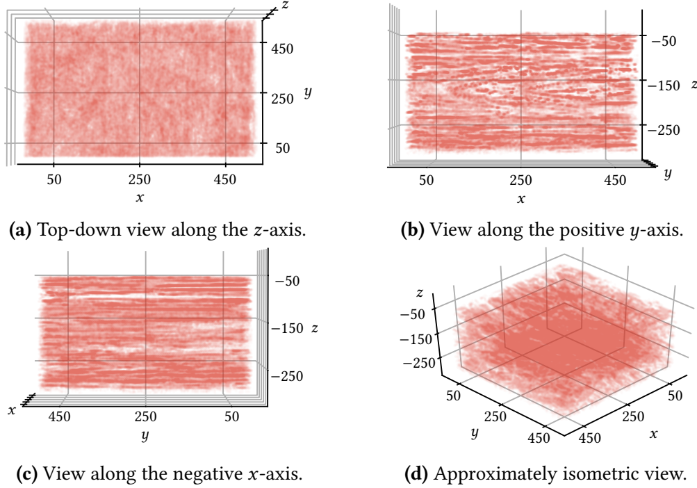
Figure 4.12: Four views of the \mathcal{U}_0 domain obtained for transport in the Førde fjord, over a time interval of 12 hours (see section 3.2), identified as the grid points which satisfy the LCS criteria (2.28a), (2.28b) and (2.28d) (details on the implementation are available in section 3.5.1). Note that the axes are given in metres, where z = 0 corresponds to the surface level, increasing downwards. In total, the domain consists of 1 631 points (cf. table 3.2).
