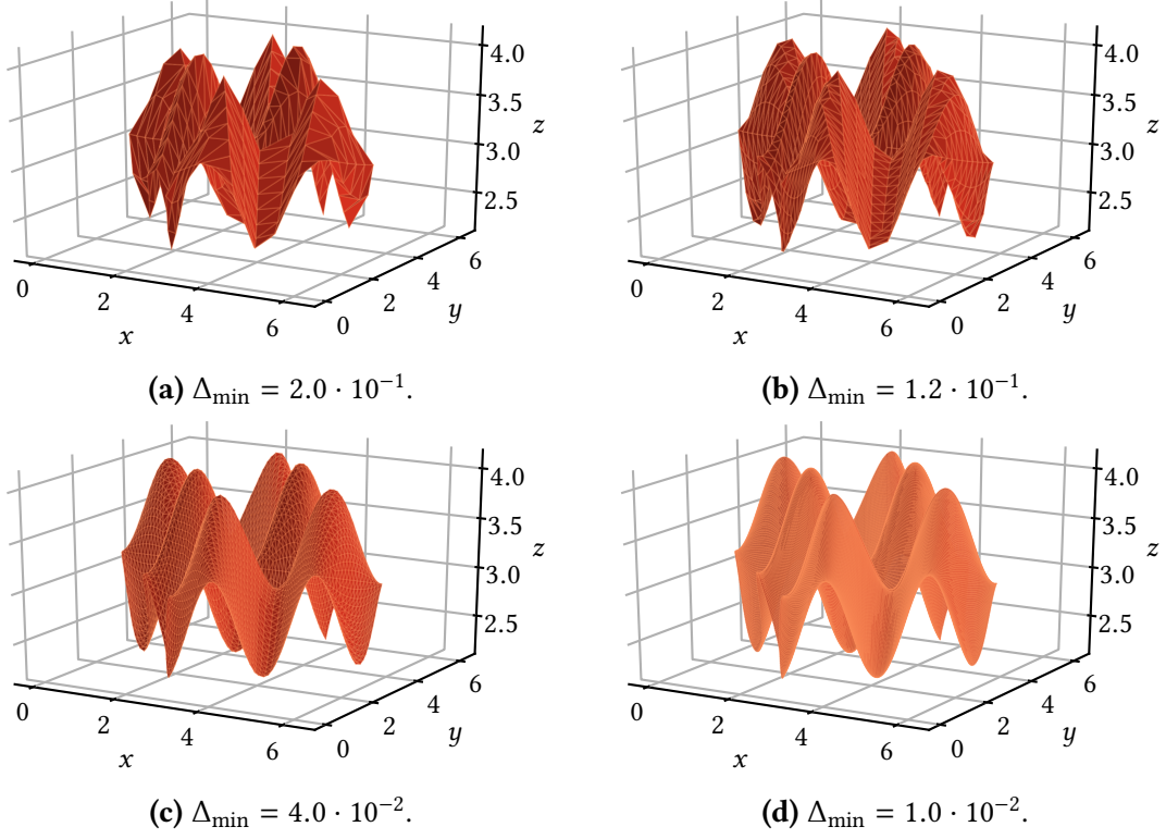
Figure 4.1: Geodesic level set approximation to an analytically known three-dimensional surface. The underlying sinusoidal surface is given by equations (4.1) and (4.3). The manifolds were all computed using the parameters given in table 4.1, with varying mesh point densities (given by the value of \Delta_{\min} ), where the mesh outlines are shown explicitly for clarity. Each of the approximations were grown from the initial position \mathbf{x}_0 = (\pi, \pi, \pi) . Note how all of the manifolds are able to capture the macroscale behaviour of the underlying surface, although the microscale behaviour is increasingly well-resolved when the mesh point density increases.
