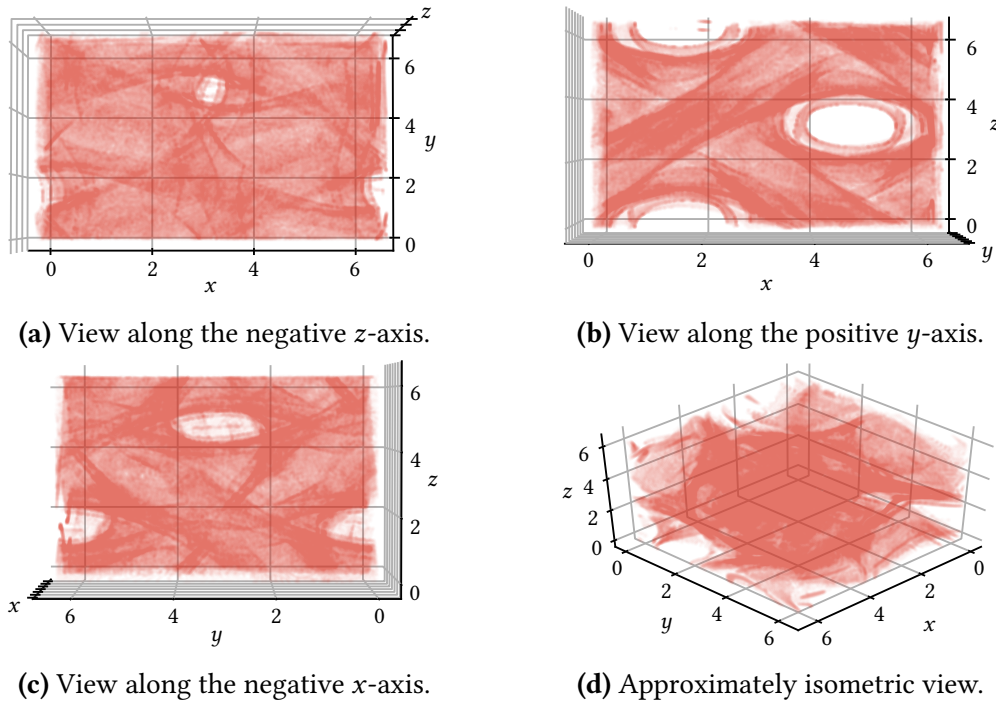
Figure 4.9: Four views of the \mathcal{U}_0 domain obtained for transport in the unsteady ABC flow, for the time interval \mathcal{I} = [0, 5] , identified as the grid points which satisfy the LCS criteria (2.28a), (2.28b) and (2.28d) (details on the implementation are available in section 3.5.1). In total, the domain consists of 361 461 different points (cf. table 3.2).
