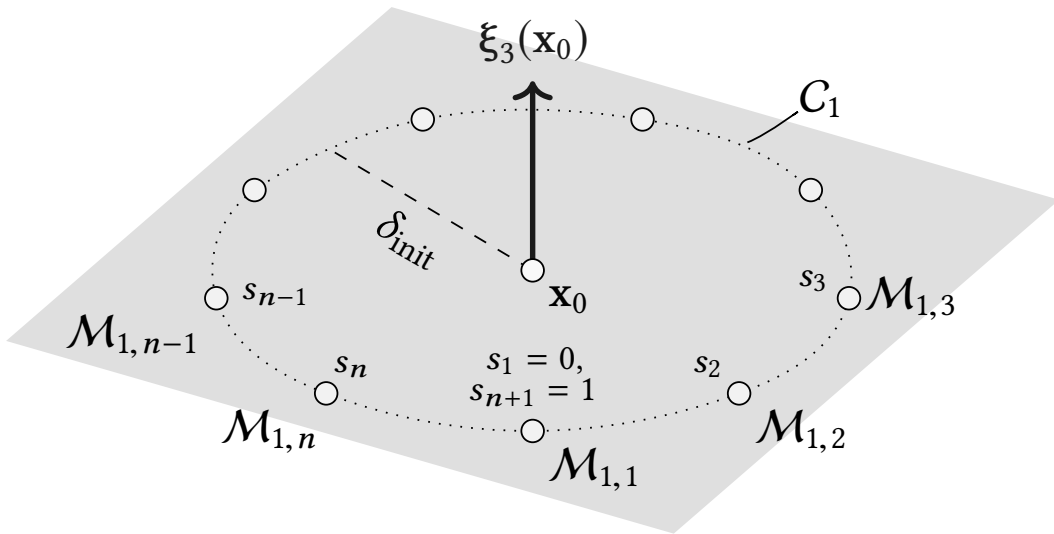
Figure 3.4: The construction of the innermost geodesic level set. An initial condition \mathbf{x}_0 is found by means of the method outlined in section 3.5.1. A set of n mesh points \{\mathcal{M}_{1,j}\}_{j=1}^n is then evenly distributed within the plane defined by the point \mathbf{x}_0 and the unit normal \xi_3(\mathbf{x}_0) , which is shaded. Each mesh point is separated from \mathbf{x}_0 by a small distance \delta_{\text{init}} (dashed). Using a normalized pseudo-arclength parameter s , the mesh point coordinates are interpolated using cubic B-splines, forming the smooth curve C_1 (dotted).
