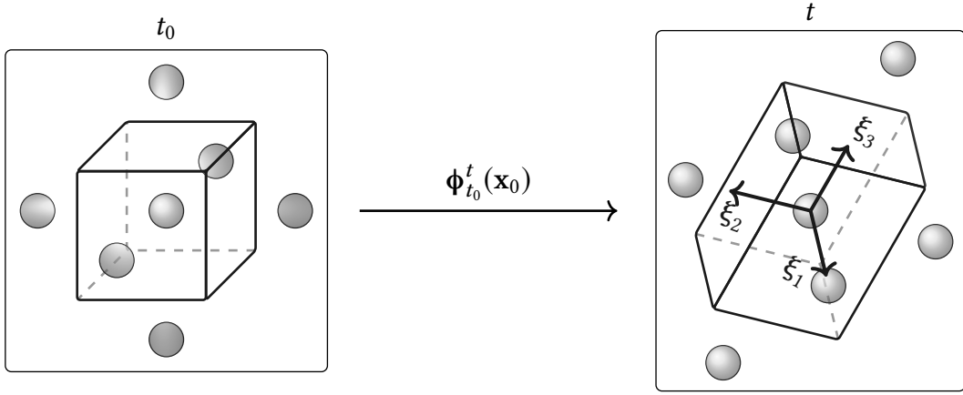
Figure 2.2: Geometric interpretation of the eigenvectors of the Cauchy-Green strain tensor. The central unit cell is stretched and deformed under the flow map \phi_{t_0}^t(\mathbf{x}_0) . The local stretching is largest in the direction of \xi_3 , the eigenvector which corresponds to the largest eigenvalue, \lambda_3 , of the Cauchy-Green strain tensor, defined in equation (2.25). Along the \xi_i axes, the stretch factors are given by \sqrt{\lambda_i} , respectively.
