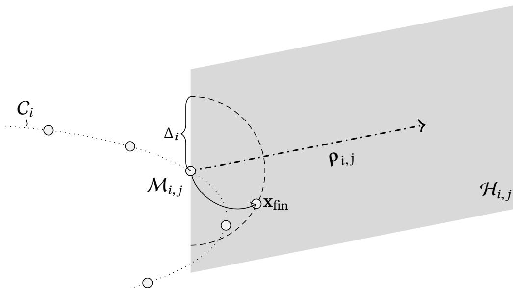
Figure 3.8: Visualization of a typical trajectory used to compute a new mesh point, using the revised approach. A trajectory is computed, starting at \mathbf{x}_{i,j} (that is, the coordinates corresponding to the mesh point \mathcal{M}_{i,j} ) and moving in the direction field given by equation (3.24), in order to find a new mesh point at the intersection between the manifold \mathcal{M} and the half-plane \mathcal{H}_{i,j} (shaded), located a distance \Delta_i from \mathcal{M}_{i,j} . \mathcal{H}_{i,j} is defined by the point \mathbf{x}_{i,j} , its unit normal \mathbf{t}_{i,j} (not shown), and the (quasi-)radial unit vector \boldsymbol{\rho}_{i,j} (dashdotted). The half-circle of radius \Delta_i , centered in \mathbf{x}_{i,j} and laying within \mathcal{H}_{i,j} , on which we seek to find a new mesh point, is dashed. As soon as a trajectory reaches a point separated from \mathcal{M}_{i,j} by a distance \Delta_i (per equation (3.26)), the integration is stopped, and a new mesh point \mathcal{M}_{i+1,j} (not shown) is placed at the trajectory end point \mathbf{x}_{\text{fin}} .
