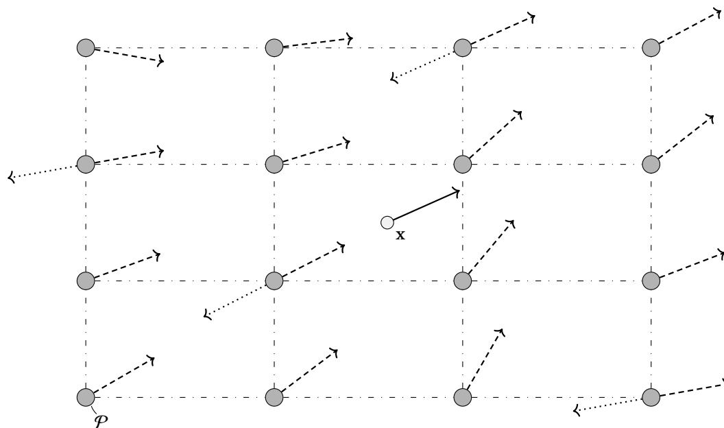
Figure 3.3: Conceptual illustration of the special-purpose cubic interpolation routine for the Cauchy-Green strain eigenvectors. The 64 nearest grid points (16 in two dimensions; here shown in gray) to any given coordinate \mathbf{x} are identified. As the local stretch is equal in magnitude along the negative \xi_i axis as that of its positive counterpart, we are free to reverse any \xi_i vector which is rotated more than 90^\circ with regards to the chosen pivot vector (at the grid point denoted by \mathcal{P} ) prior to interpolating the components of \xi_i , making use of cubic B-splines. The vectors used in the local cubic interpolation are dashed, whereas the vectors which had to be reversed are dotted.
