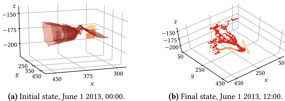
Figure 4.14: Advection of tracers in order to verify the repelling nature of the computed LCSs in the Førde fjord. At midnight June 1, 2013, two blobs of initial conditions are placed at opposite sides of the most strongly repulsive LCS identified for flow in the Førde fjord (see figure 4.13) as shown in (a). The two blobs, and the mesh points in the parametrization of the LCS, are then advected in the model data for the oceanic currents briefly described in section 3.2.1, using the Dormand-Prince 8(7) ODE solver, for the 12 hour time interval of interest, where the final state is shown in (b). Note that, although the LCS triangulation breaks down under the advection, the two blobs of particles remain on fairly compact, and remain on the opposite sides of the LCS, never crossing the LCS surface. This indicates that the local centre of strongest repulsion remains located inbetween the two blobs of particles throughout – which is the exact behaviour we expect for a repelling LCS.
