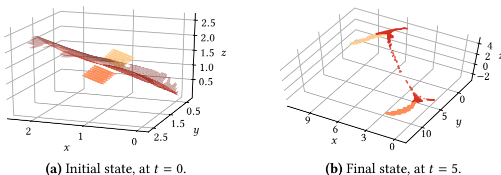
Figure 4.7: Advection of tracers in order to verify the repelling nature of the computed LCSs. At t = 0 , two blobs of initial conditions are placed at opposite sides of a repelling LCS identified in the steady ABC flow — more on which to follow in section 4.3 — as shown in (a). The two blobs, and the mesh points in the parametrization of the LCS, are then advected by the velocity field given by equations (3.1) and (3.2) using the Dormand-Prince 8(7) ODE solver, until t = 5 , for which the corresponding state is shown in (b). Note that, although the LCS triangulation breaks down under the advection, the two blobs of particles remain on fairly compact, and remain on the opposite sides of the LCS, never crossing the LCS surface. This indicates that the local centre of strongest repulsion remains located inbetween the two blobs of particles throughout — which is the exact behaviour we expect for a repelling LCS.
