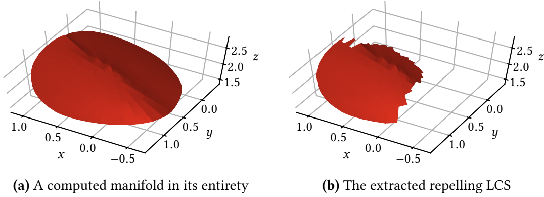
Figure 3.16: An example of a repelling LCS extracted as a subset of a computed manifold. In (a), a sample manifold for the steady ABC flow is shown, whereas (b) shows the subset of the manifold which satisfies the LCS existence criteria given in equation (2.28) (or is sufficiently close to any point satisfying these criteria, meaning that their inclusion facilitates triangulations which provide an overall enhanced visual representation).
