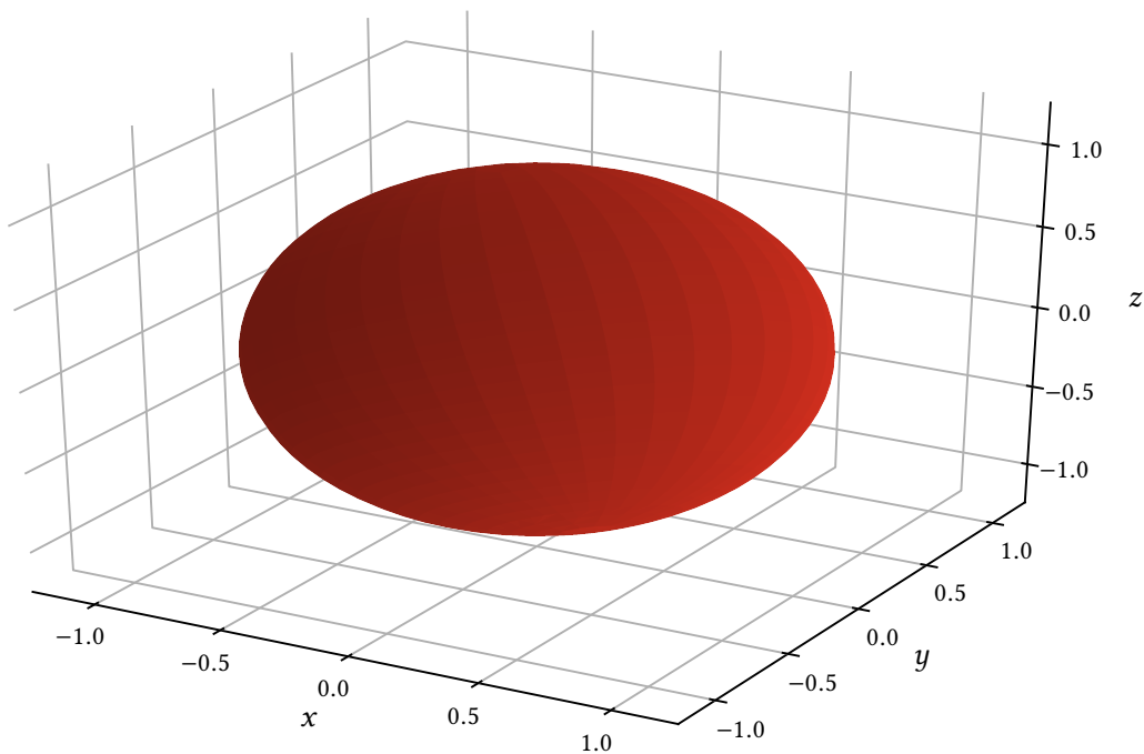
Figure 4.6: The single repelling LCS present in the purely radial velocity field given by equation (4.5) with r = 1 . In computing the underlying manifolds, we used the filtering parameters \varepsilon = 5 \cdot 10^{-3} and \nu = 20 (cf. section 3.5.1 and table 3.2), and otherwise the same parameter values as given in table 4.2. To extract LCSs, we used the tolerance parameter \gamma_{\blacktriangleright} = 1.2 , keeping only the LCSs whose (pseudo-)surface area was greater than or equal to \mathcal{W}_{\min} = 1 (see section 3.11). This resulted in 3 identical (to numerical precision) copies of a single, spherical, repelling LCS of unit radius – which is exactly as expected, given the sharp repulsion maximum at \|\mathbf{x}\| = 1 , as shown in figure 4.5.
