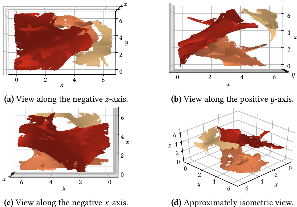
Figure 4.11: Four views of the repelling LCSs obtained for transport in the unsteady ABC flow, for the time interval \mathcal{I} = [0, 5] (see section 3.1.2). A total of 31 surfaces constitute three distinct, reasonably smooth and coherent structures, which are shown in different colors. We provide four different viewing angles (the same as the ones used in figure 4.9, which shows the computed \mathcal{U}_0 domain), chosen in order convey the three-dimensional structures in as great detail as possible.
