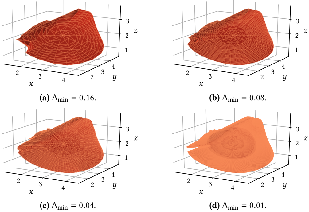
Figure 4.3: Geodesic level set approximations with varying mesh point densities, for a manifold in the steady ABC flow (see section 3.1). The manifolds were all computed using the parameters given in table 4.1, with varying mesh point densities (here noted by their \Delta_{\min} ), where the mesh outlines are shown explicitly for clarity. Each of the approximations were grown from the same initial position \mathbf{x}_0 . Note how, although the microscale behaviour generally is more well-resolved as the mesh point density increases, there appears to be a threshold above which undesired numerical artefacts – perhaps most notably near the left edge of the manifold shown in (d) – manifest.
