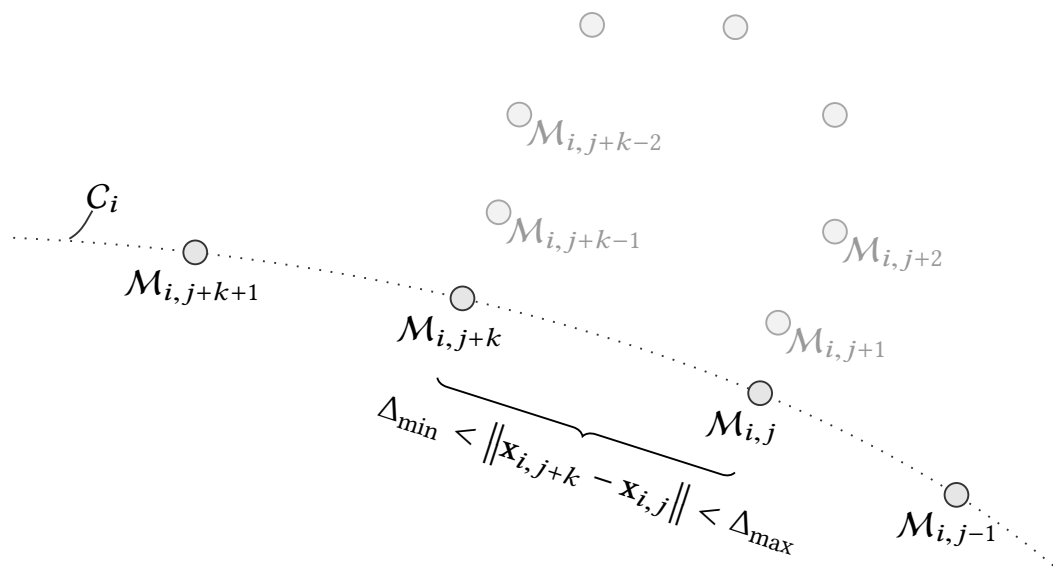
Figure 3.11: Our approach to limit the compound numerical error, by continuously removing unwanted loops in the computed level sets. As the separation between the mesh points \mathcal{M}_{i,j} and \mathcal{M}_{i,j+k} satisfies the restrictions regarding mesh point density (cf. section 3.8.1), the mesh points \{\mathcal{M}_{i,j+\kappa}\}_{\kappa=1}^{k-1} (shown in a lighter shade of gray) are removed, provided that the cumulative neighbor separation around the bulge is sufficiently large (per the conditions presented in equation (3.27)) – which is the case in the above. The resulting interpolation curve C_i becomes significantly more well-behaved without the superfluous mesh points.
