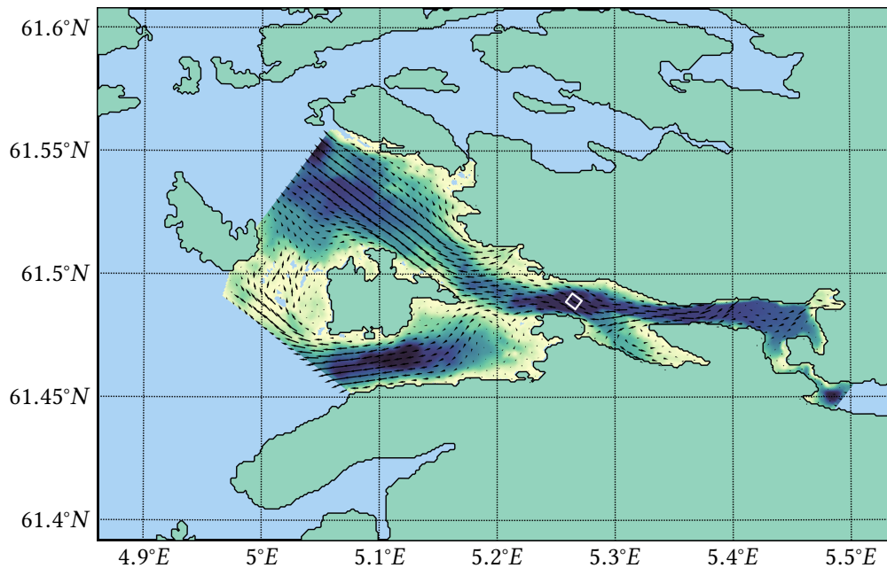
Figure 3.2: Stereographical map projection of the Fårde fjord and its surroundings. The local fjord depths are indicated by a varying background color. A subset of the gridded velocity vectors indicates the macroscopic trends of the oceanic currents at a depth of 3 m below the surface. Outlined in white is a bird’s-eye view of the main region of interest; namely, a region of water which was neither particularly close to the oceanic surface, nor struck the coastline when transported by the currents for the duration of the 12 hour time interval of interest.
