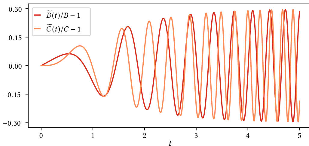
Figure 3.1: Time dependence of the coefficient functions for unsteady ABC flow, defined in equations (3.2)–(3.4).
