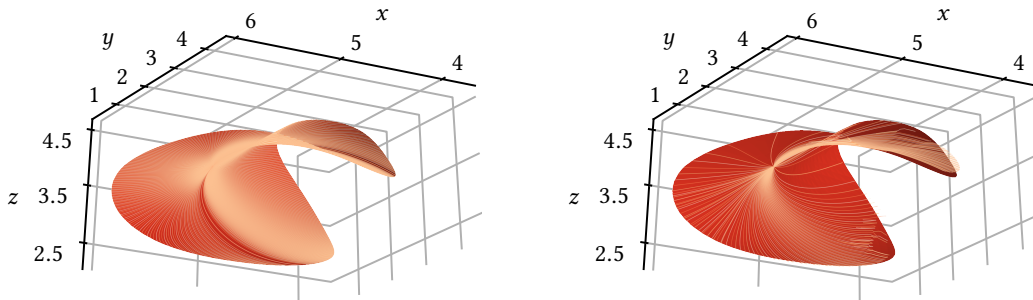
(a) Trajectories computed in the direction field given by equation (3.24). (b) Trajectories of the direction field given by equation (2.31), for various weights (a, b) .
