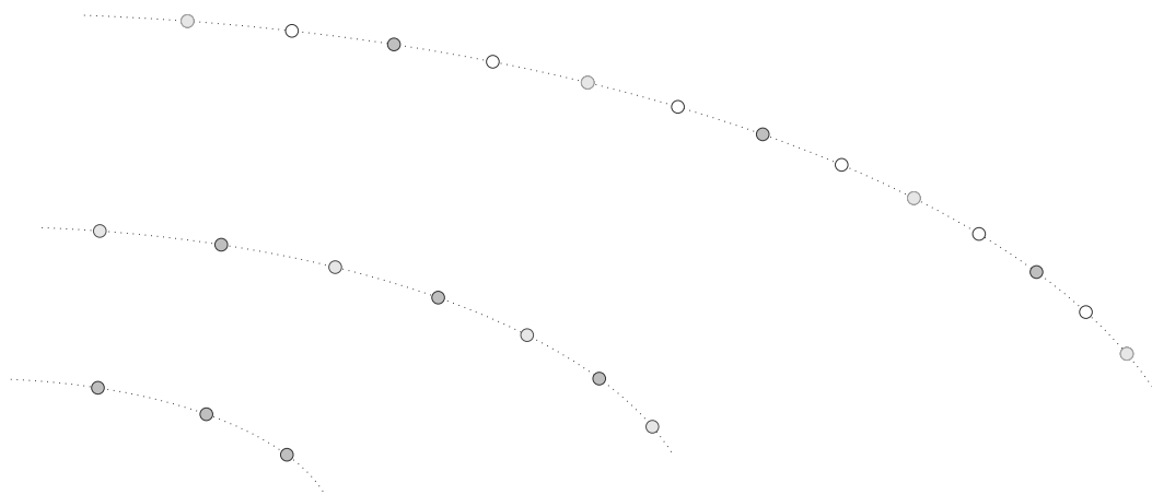
Figure 3.9: Conceptual illustration of the rationale behind the insertion of new mesh points as the geodesic level sets expand. The shown subset of the innermost topological circle is parametrized by three mesh points, shown as dark gray circles. As the topological circle is expanded, an increasing amount of mesh points must be inserted in order to maintain the (approximate) mesh point density. In the intermediate-sized circle shown in the figure, the mesh points with no direct analogue in the smallest circle are shown in a lighter shade of gray. Similarly, in the largest circle shown, the mesh points with no direct analogue in the intermediate-sized circle are drawn without fill.
