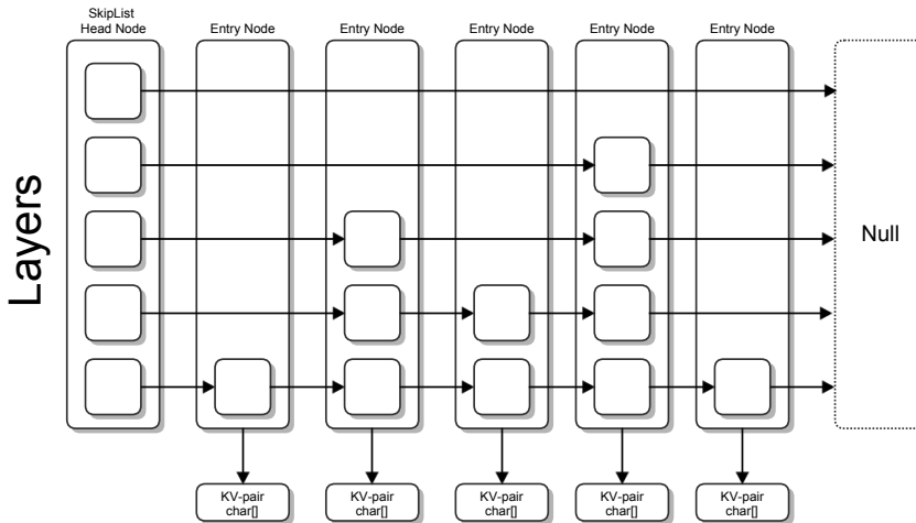
Figure 2.7: Memtable Skip-list
