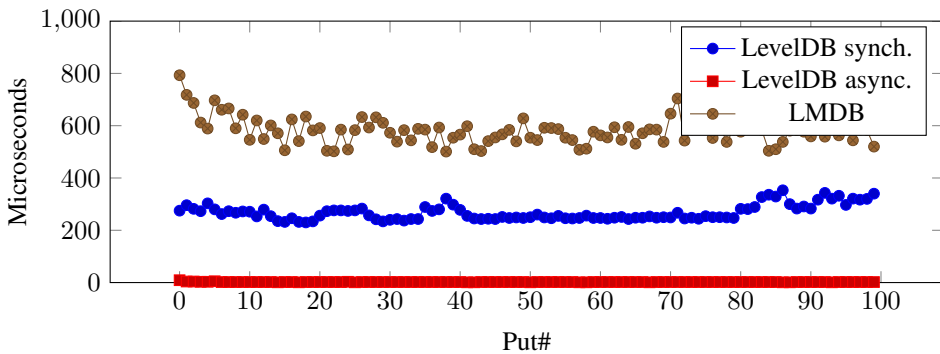
Figure 4.1: The duration of Put -operations with a 4-byte key and 1 byte value. No compactions were running or started for the duration.
