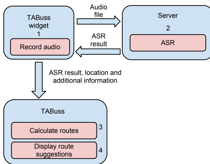
Figure 6.5: The TABuss widget architecture
