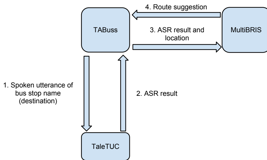
Figure 6.4: TABuss' query based on ASR results
