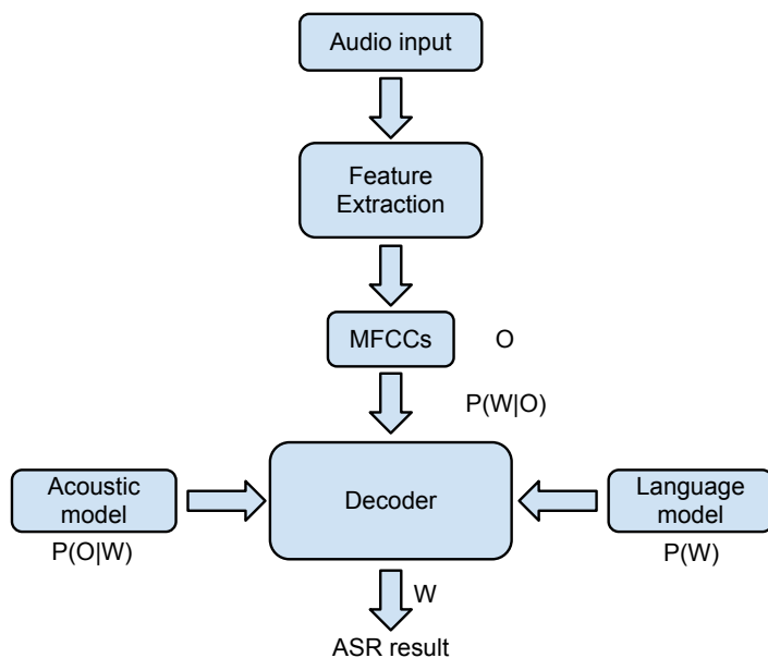
Figure 2.1: ASR architecture
