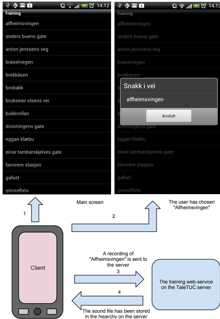
Figure 7.1: The recording application that collects data for the acoustic model
