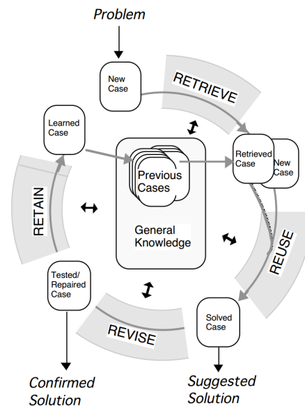
Figure 3.1: The classical representation of the CBR cycle by Aamodt and Plaza (1994)
