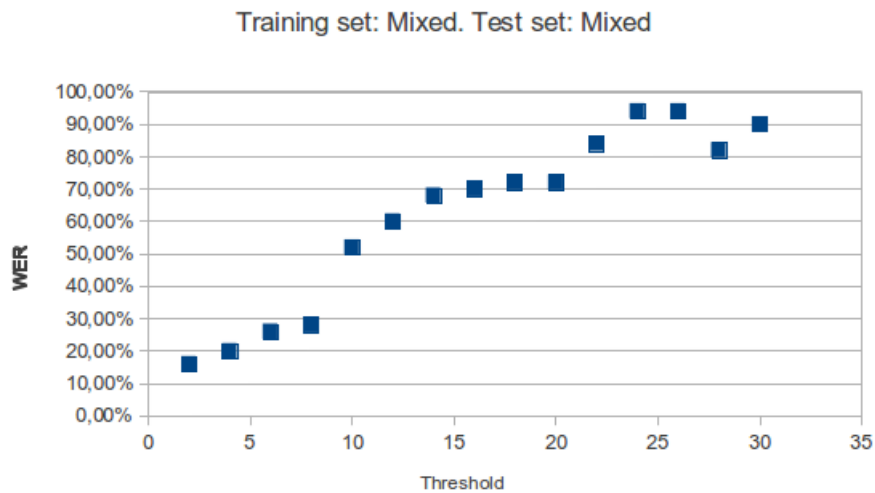
Figure 7.4: VAD threshold test 3
