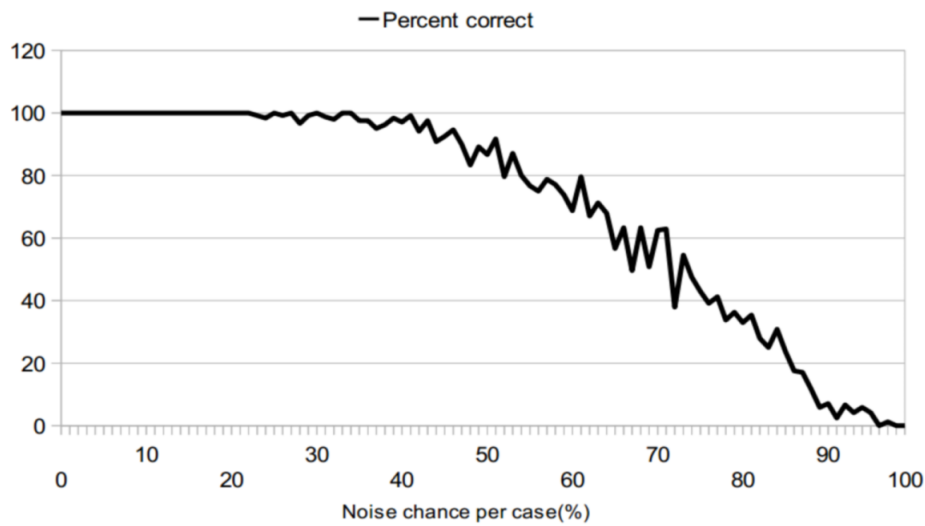
Figure 7.13: Correct guesses with noise amount (noise excluded from the test data), when using 2x10-fold cross-validation. Case-base includes 200 cases
