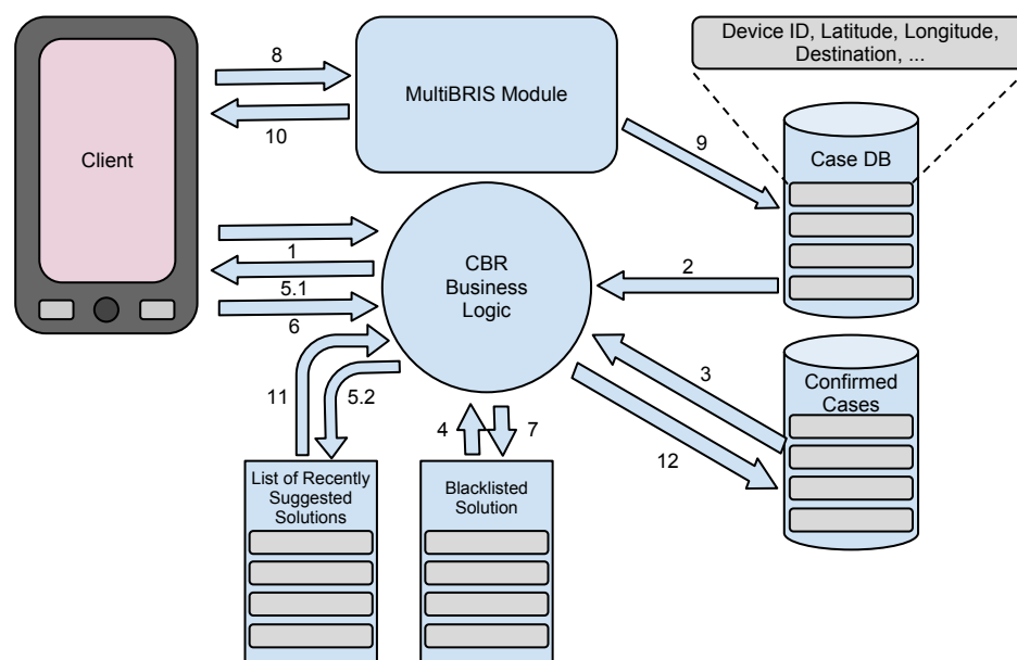
Figure 6.3: CBR Module
