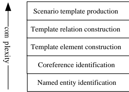
Figure 2.3: Five tasks of information extraction
