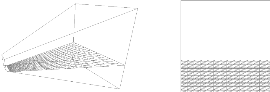
(a) seen from outside the frustum (b) seen from the projecting camera Figure 14: A projected grid. (a) tessellation seen from a second camera. Notice the increased vertex spacing in the far end of the viewing frustum. (b) tessellation seen from the projecting camera. Notice the uniform spacing of vertices.
