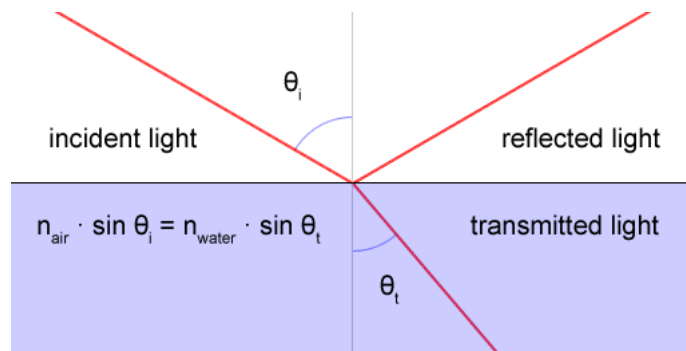
Figure 24: An illustration of Snell's law. Here, the upper medium is air, and the lower medium (shaded) is water. The interface between the two media is the center horizontal line. The angle of incidence is \theta_i , and the angle of refraction is \theta_t .
