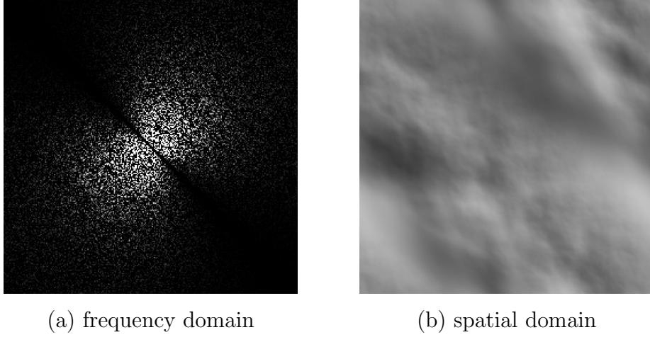
Figure 6: Ocean synthesis. (a) shows the magnitudes of a sampled frequency spectrum, and (b) shows the spatial height map synthesized from this spectrum.
