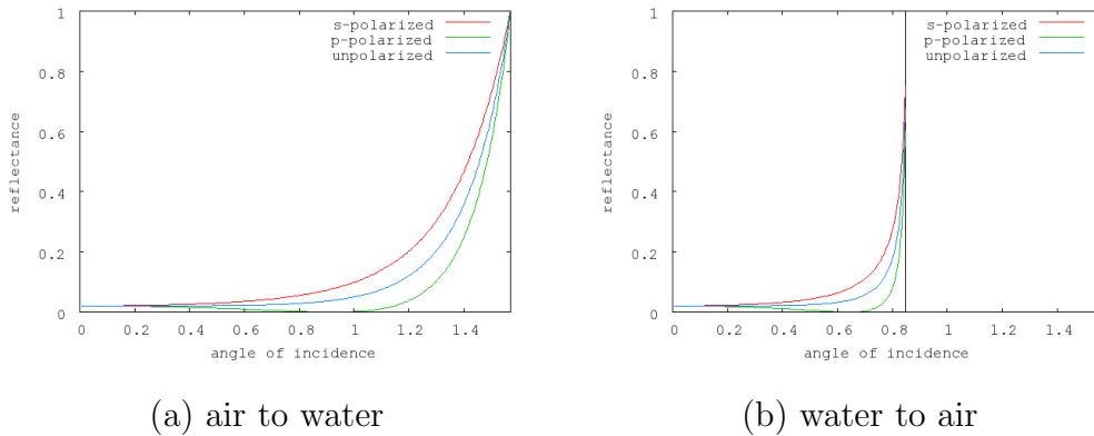
Figure 25: Fresnel reflectance at the air-water boundary. (a) and (b) show the reflectance for light transmitted by air and water, respectively. The vertical line in (b) marks the critical angle, beyond which total internal reflection occurs. The middle curve, in both diagrams, is the average of the reflectance for s -polarized and p -polarized radiation.
