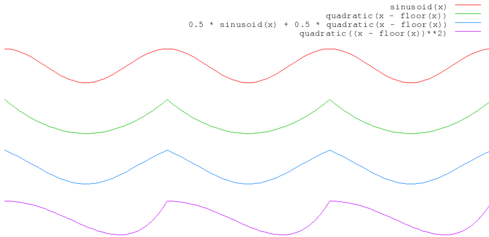
Figure 1: Various wave profiles. From top to bottom: sinusoid wave, piecewise quadratic wave, blended wave, quadratic wave with exponentiated argument. The functions used here are: \text{sinusoid}(x) = \cos(2\pi x) and \text{quadratic}(x) = 8(x - 0.5)^2 - 1 .
