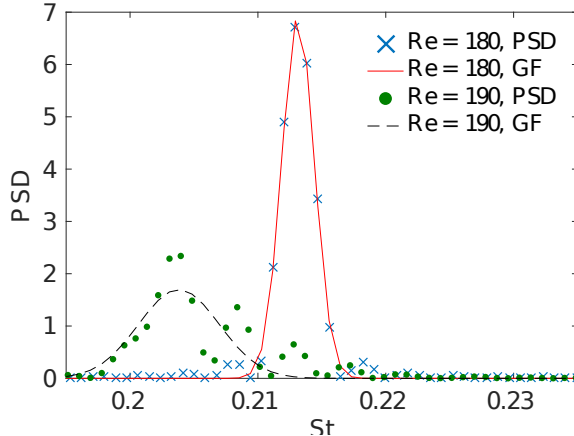
Figure 5. Power spectral density (PSD) as a function of Strouhal number with curve fitted Gaussian distribution (GF), for flow LFS flow at Re = 180 (PSD: \times , GF: —) and Re = 190 (PSD: \bullet , GF: - -).
