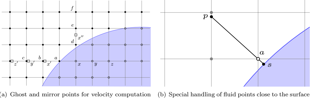
Figure 1. Immersed boundary method. (a) Ghost points (x,y,z; \circ) used in the central-difference stencils of fluid points (a-c; \bullet) are set by mirror points (x',y',z'; \square) . The mirror points are interpolated along grid lines. When (x; \circ) is used to compute vertical velocity components of fluid points (d-f; \bullet) the corresponding mirror point is (x''; \square) . (b) For a fluid point (a; \circ) very close to the cylinder surface, interpolation between a surface point (s; \bullet) and the intersection between the surface normal and the first grid line at (p; \bullet) is used.
