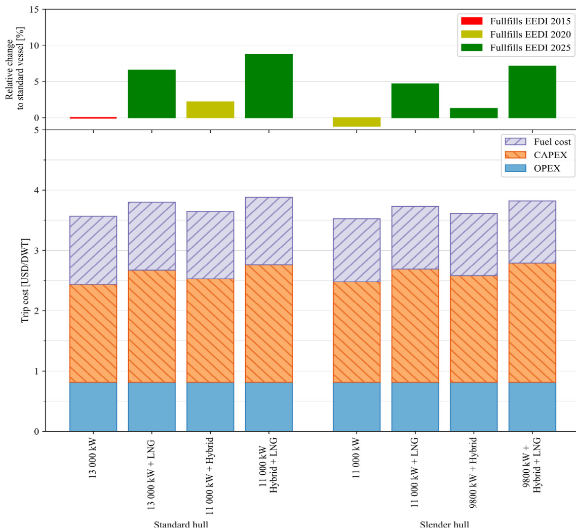
Fig. 9. Roundtrip voyage cost for vessels sailing at medium speed.
