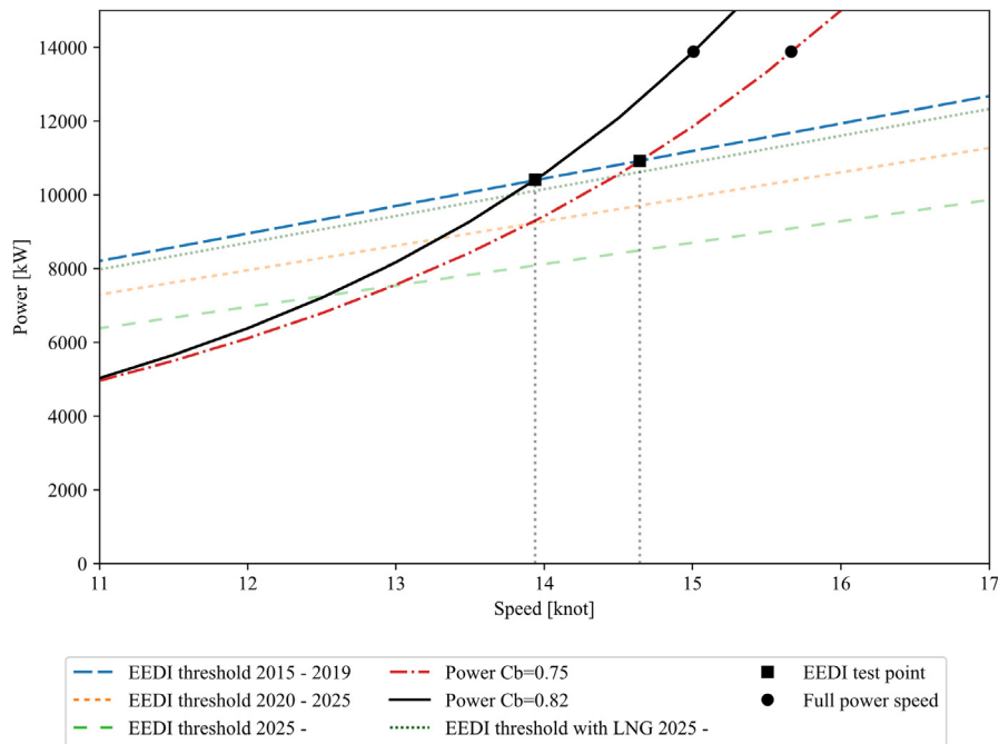
Fig. 5. Graphic representation of the EEDI score.
