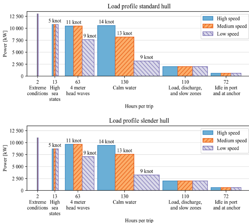
Fig. 7. Power demand and duration of the different sailing modes.
