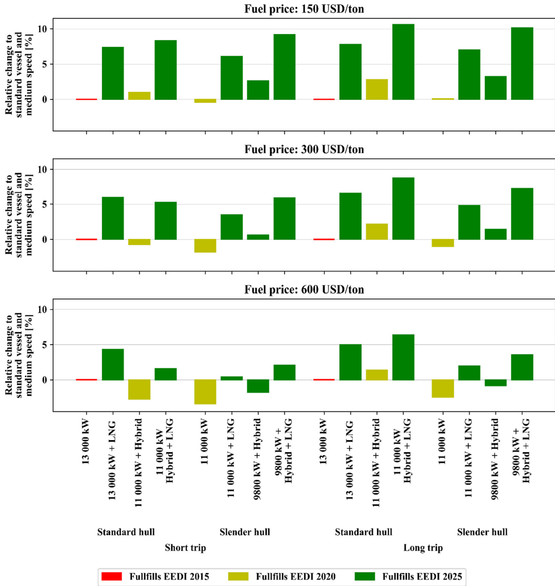
Fig. 12. Relative voyage costs of round-trip of 7500 NM.
