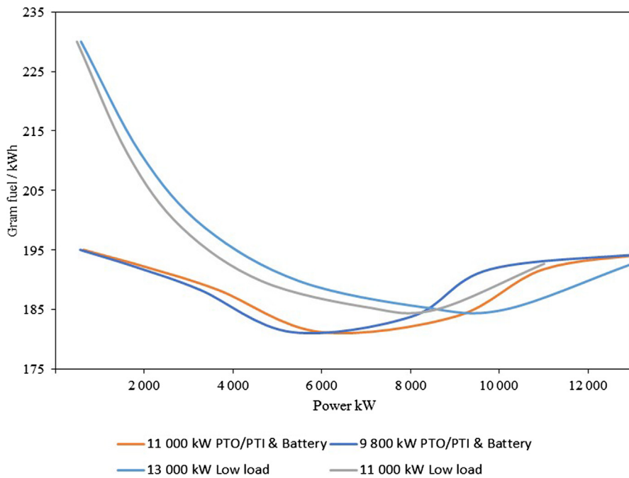
Fig. 4. Specific fuel oil consumption (SFOC) as a function of power option.
