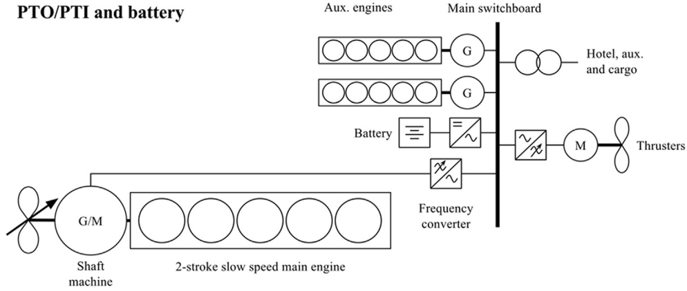
Fig. 3. Configuration of a hybrid power system with PTO/PTI and batteries.
