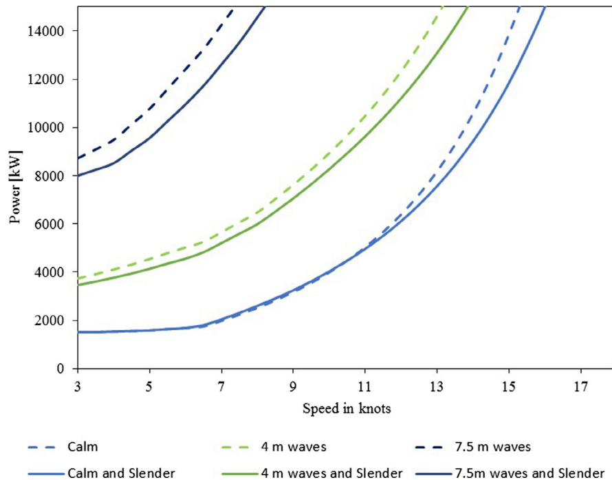
Fig. 2. Power requirements for conventional and slender hulls.
