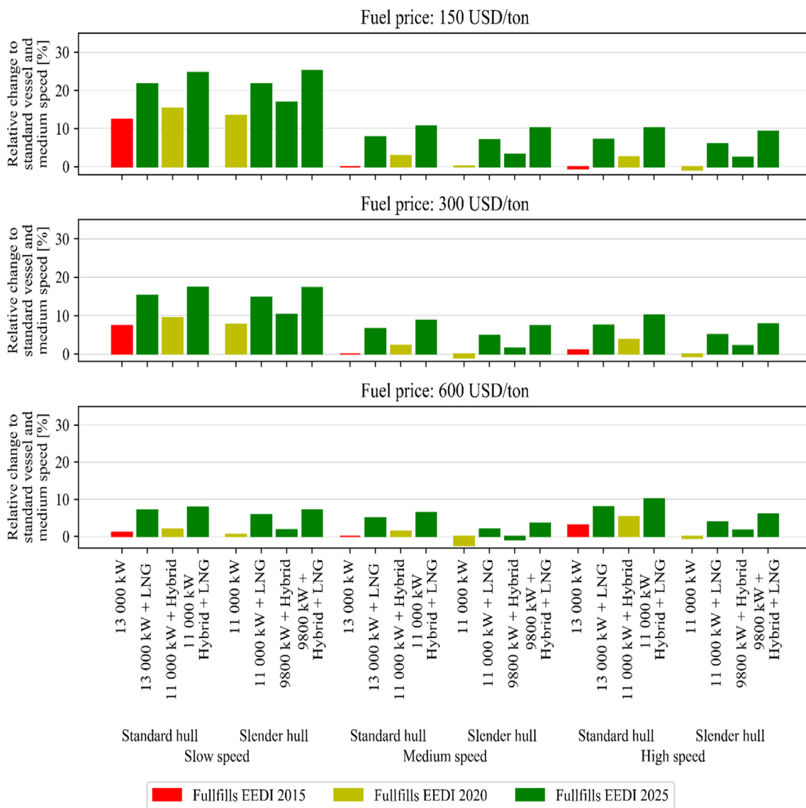
Fig. 11. Cost differences as a function of speed and fuel price.
