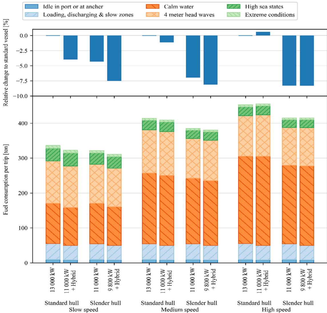
Fig. 8. Fuel consumption.
