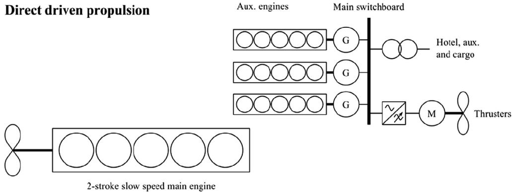
Fig. 1. Power and propulsion machinery setup for direct-driven propulsion.
