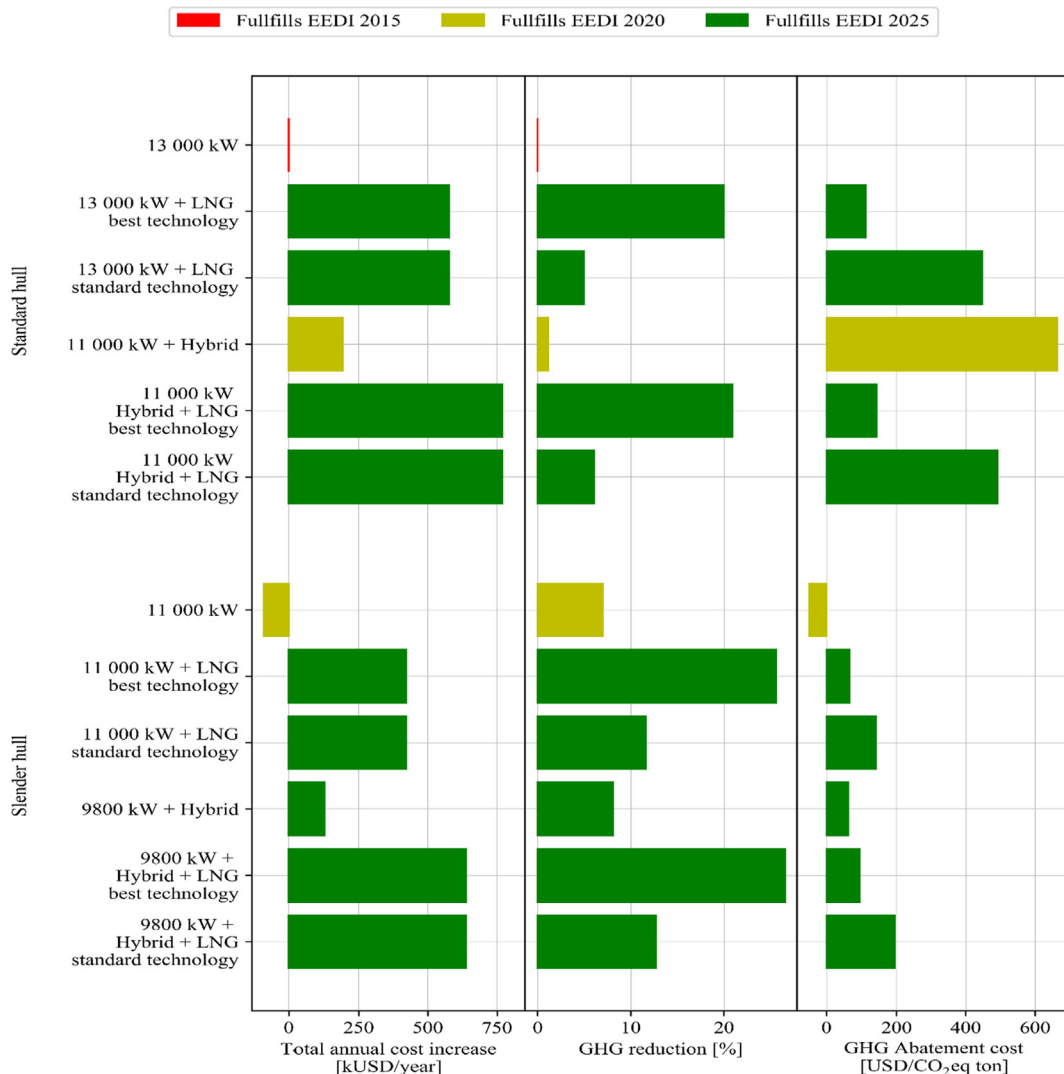
Fig. 10. Abatement cost of the various options.
