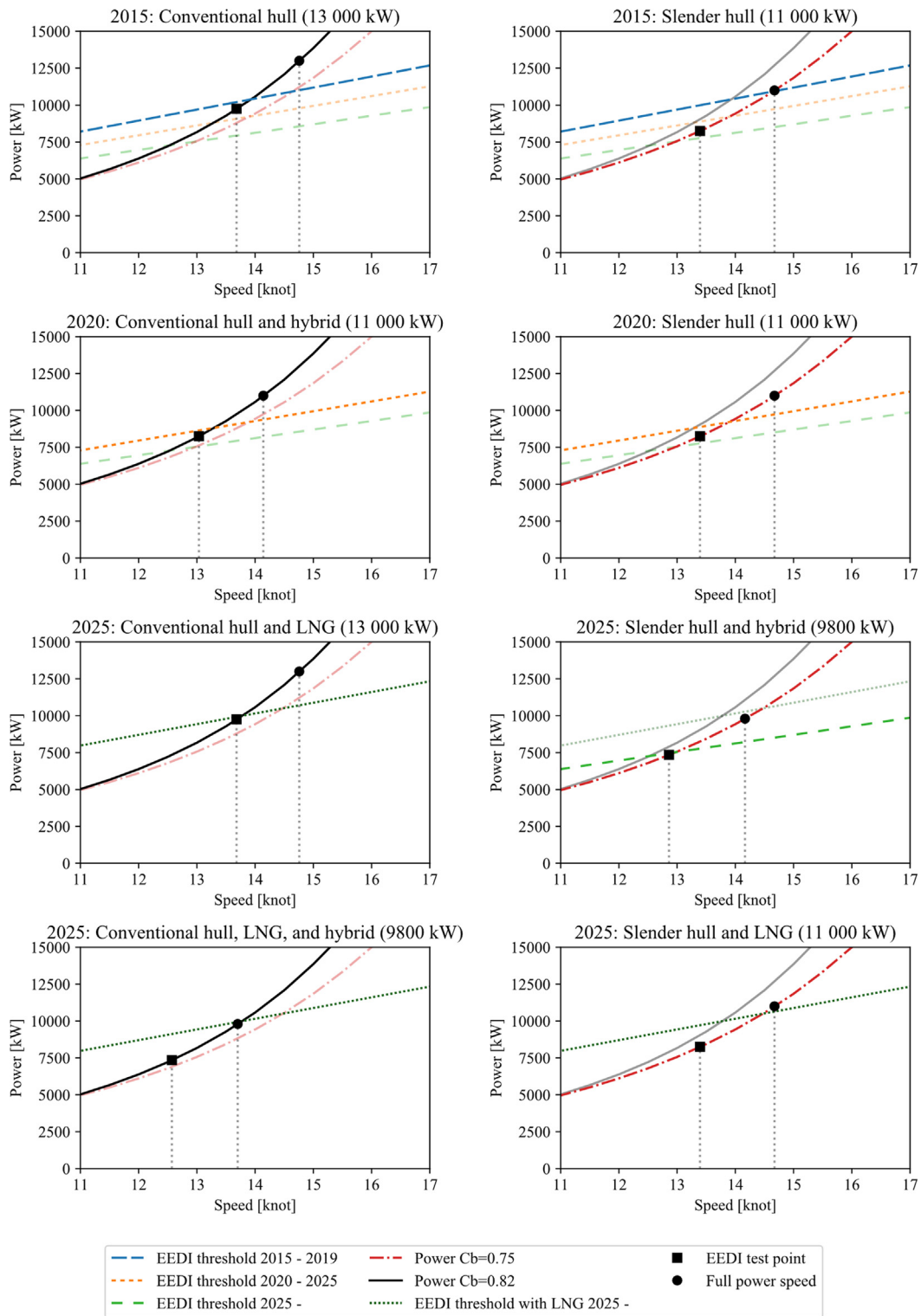
Fig. 6. Power and EEDI thresholds in 2015, 2020 and 2025 for a 110,000-dwt tanker.
