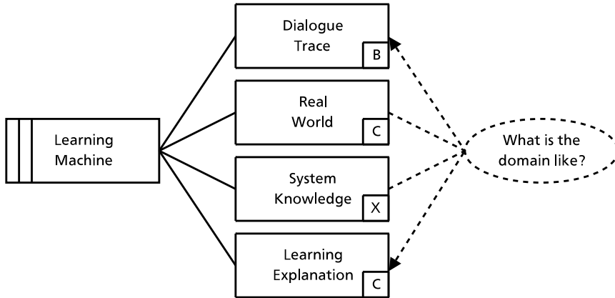
Figure H.5.: Learning Explanation. This goal is special, since it focuses on the user's interest in the application domain (hence the real world), and not on some particular behaviour of the system.
