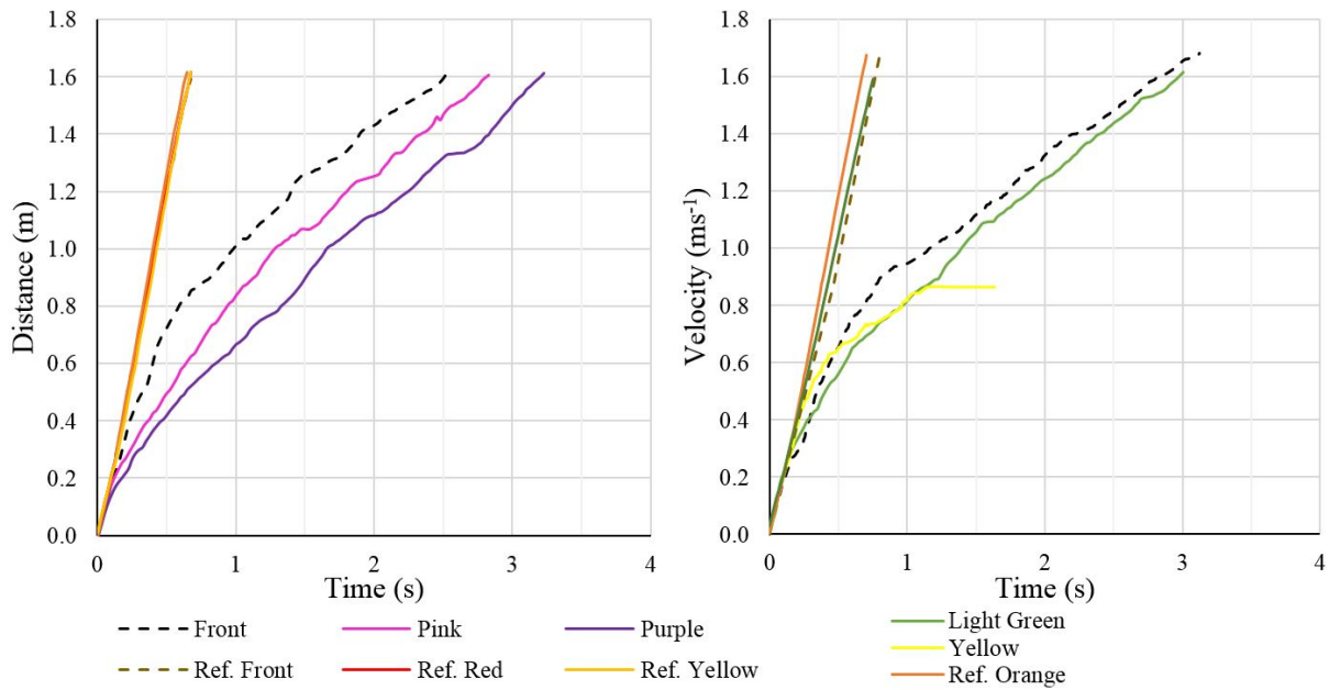
Figure 5.9: Diagram of ballotini flowing through 25% forest at 50% relative humidity showing the change in surface/front velocity between forested and unforsted terrain.
