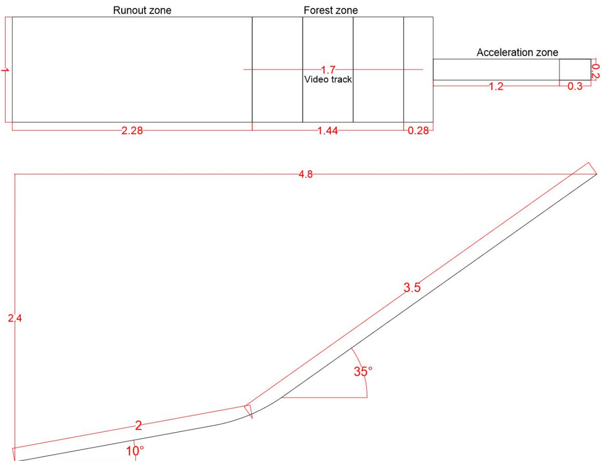
Figure 4.1: Chute design
