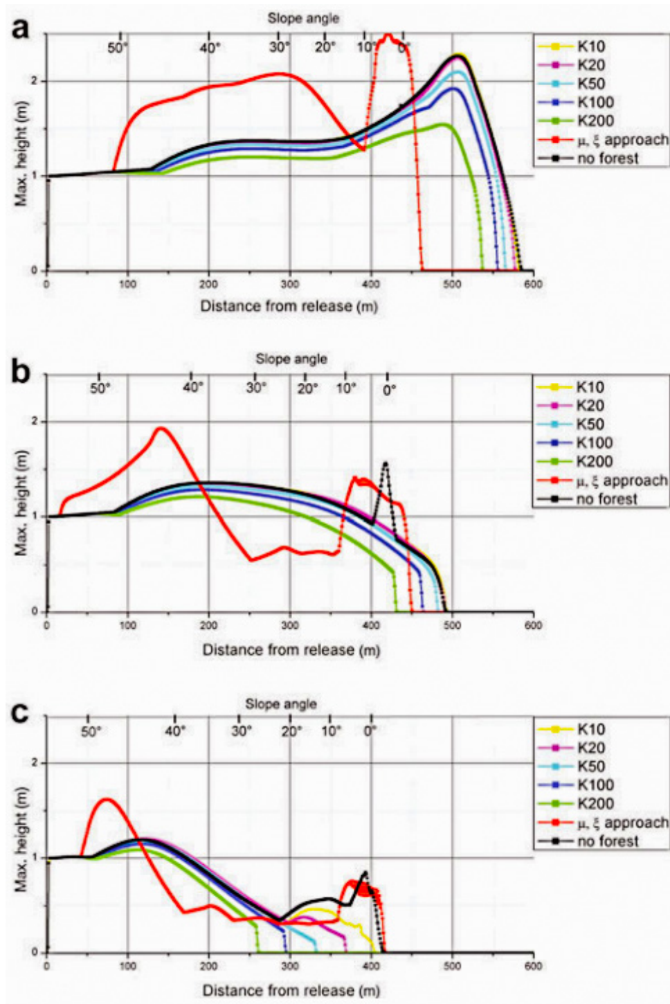
Figure 3.9: Fig 9. Maximum flow height profiles for simulations of snow avalanches with dissimilar release volumes: (a) 20\,000\ m^3 ; (b) 5\,000\ m^3 ; (c) 1\,000\ m^3 and calculated via VS model of RAMMS on a parabolic slope using both the friction and detrainment approaches. Five different values for the detrainment coefficient, K (Pa), were tested (K10, K20, K50, K100, K200). (Feistl et al., 2014)
