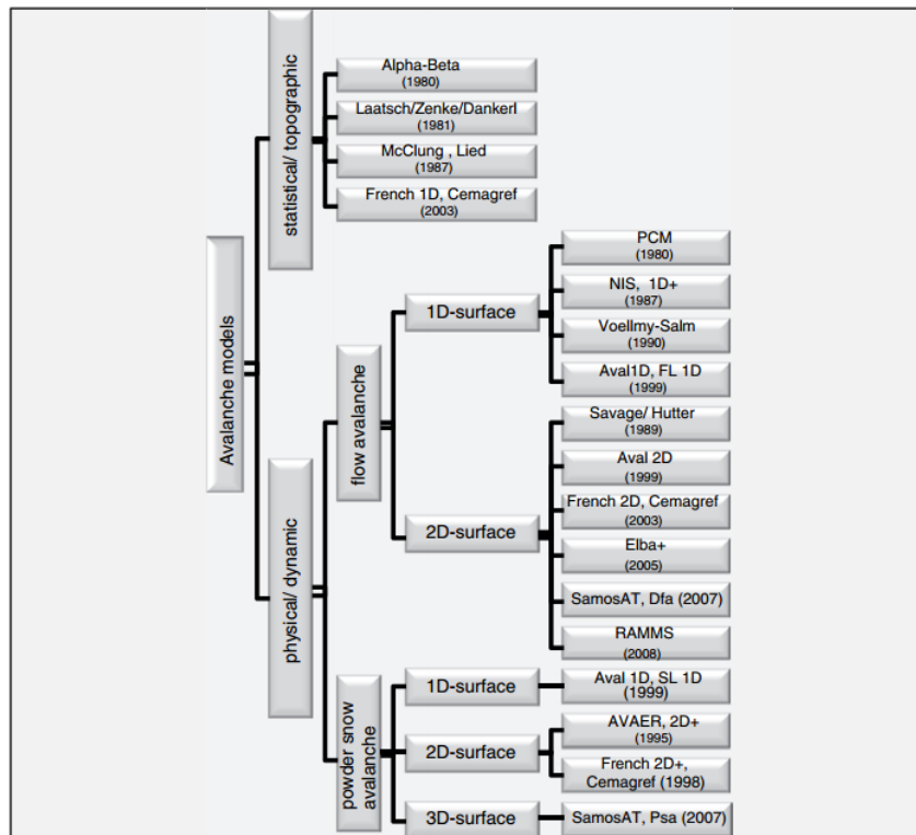
Figure 3.3: Overview and classification of common avalanche models (classification and dimensioning relative to the corresponding calculation platform)(From: Granig, Margreth)(Rudolf-Miklau et al., 2015)
