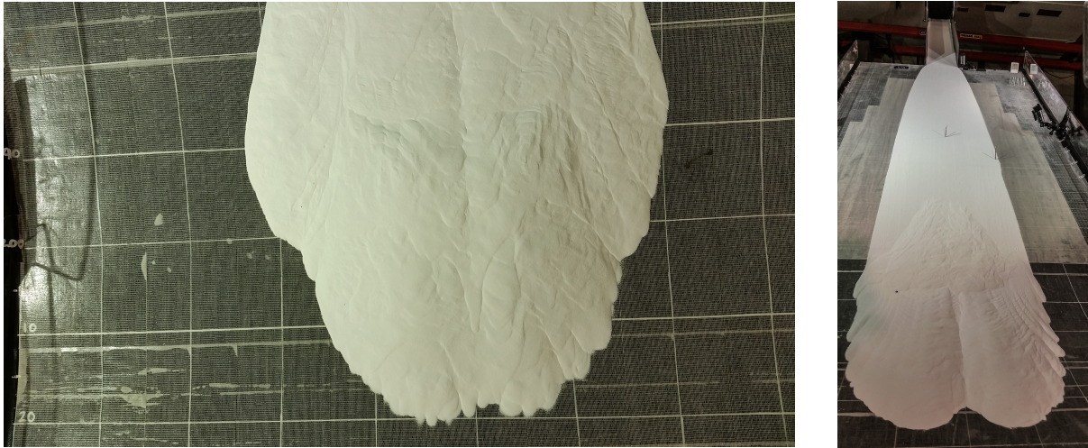
Figure 4.6: Alumina reference trials showing blown-up runout distance alongside the chute view.
