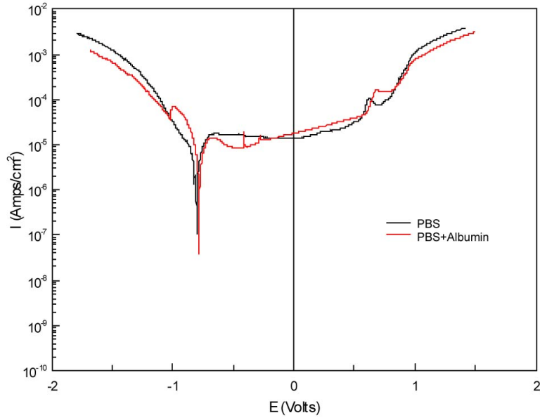
Figure 4.44: Effect of presence of 2 g/L Albumin on the polarization curves of surgical grade Co-Cr-Mo grade F75. Experimental conditions: T=37°C; pH=7.4; PBS without and with albumin addition.
