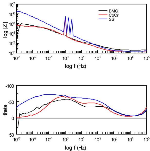
Figure 4.83: Bode plots of EIS data for SS, CoCr and BMG in PBS solution, T=20\text{ }^{\circ}\text{C} , \text{pH } 7.4 .
