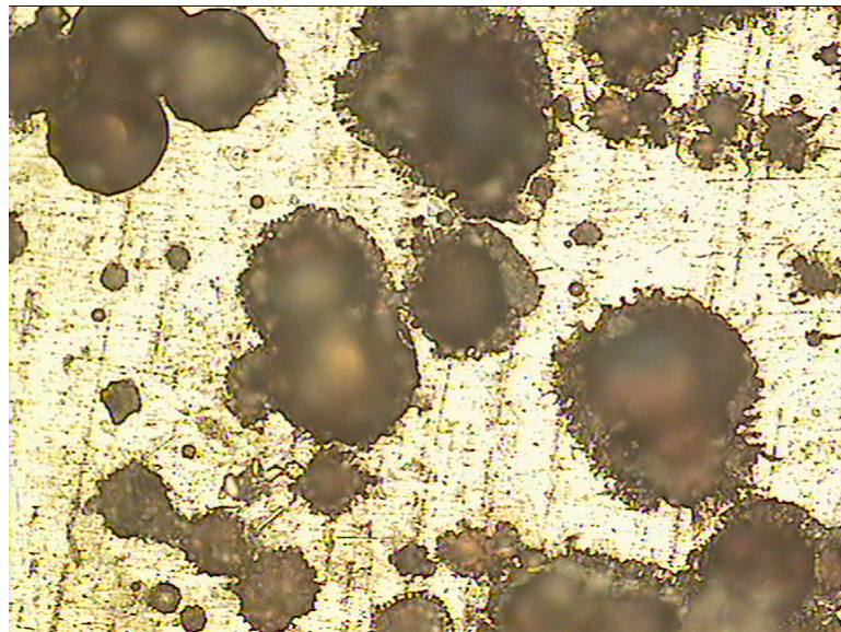
Figure 6.68: Pitting corrosion on the surface of the zirconium based bulk metallic glass in PBS solution. T=37°C; pH=7.4; Magnification 400X.
