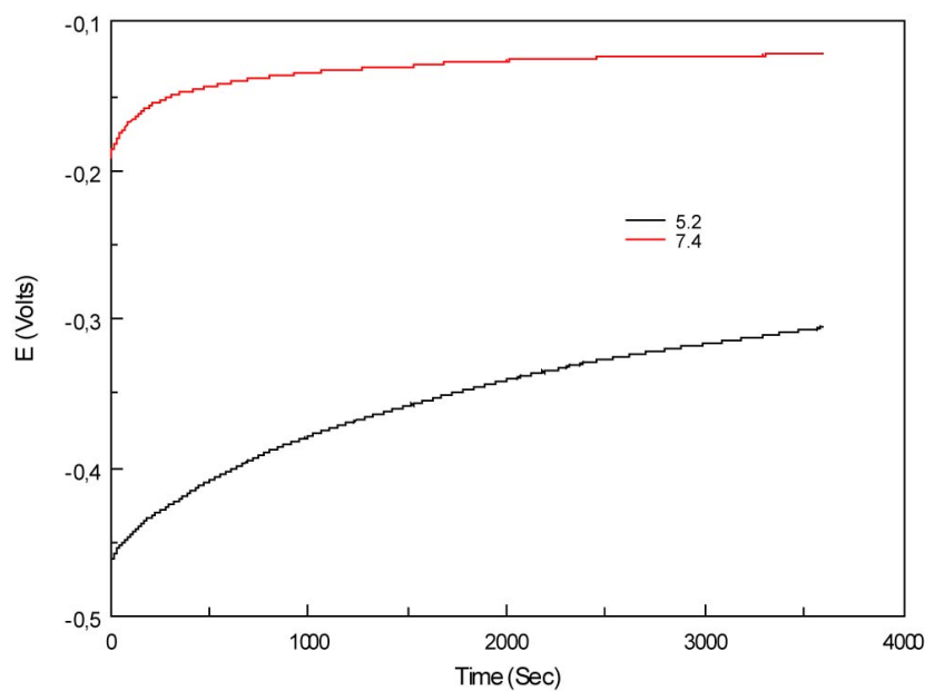
Figure 4.39: Effect of pH on OCP value of stainless steel 316. Experimental conditions: T=37°C; PBS with 2 g/L albumin; pH= 7.4 and 5.2.
