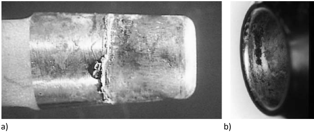
Figure 2.7: (a) Modular junction taper connection of a total hip arthroplasty showing corrosion of the taper connections. (b) Macrograph of deposits of \text{CrPO}_4 corrosion particle products on the rim of a modular cobalt–chrome femoral head [9].
