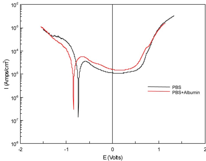
Figure 4.45: Effect of presence of 2 g/L Albumin on the polarization curves of surgical grade Co-Cr-Mo grade F75. Experimental conditions: T=37°C; pH=5.2; PBS without and with albumin addition.
