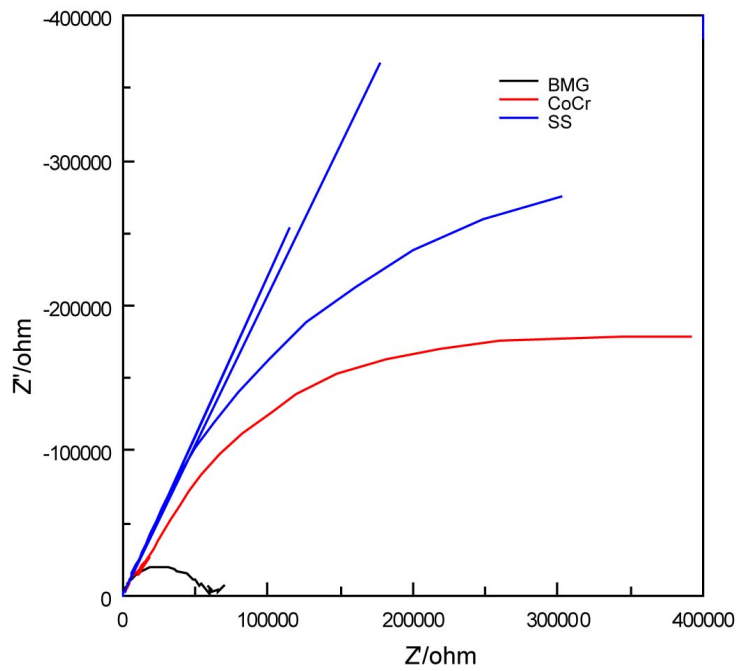
Figure 4.88: Experimental Nyquist plot in PBS with 2g/L albumin, T=37 °C, pH 7.4, after holding the samples at open circuit potential for 1 h.
