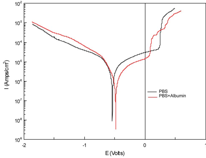
Figure 4.48: Effect of presence of 2 g/L Albumin on the polarization curves of zirconium based bulk metallic glass. Experimental conditions: T=37°C; pH=7.4; PBS without and with albumin addition.
