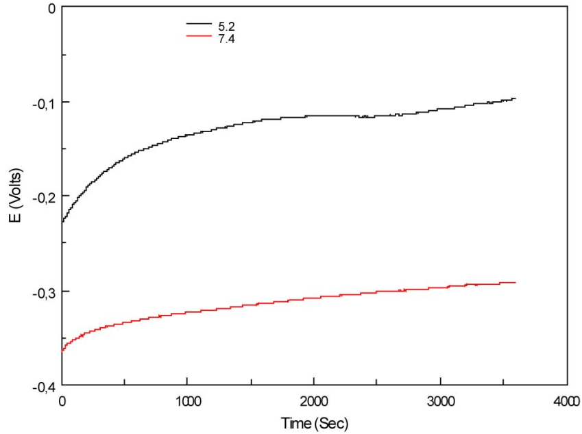
Figure 4.26: Effect of pH on OCP value of surgical grade Co-Cr-Mo grade F75. Experimental conditions: T=37°C; PBS; pH= 7.4 and 5.2.
