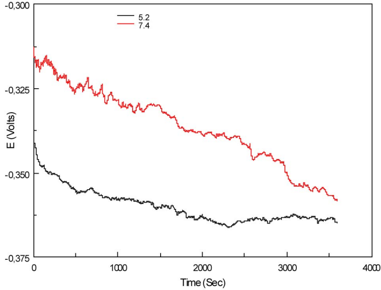
Figure 4.34: Effect of pH on OCP value of crystalline bulk metallic glass. Experimental conditions: Experimental conditions: T=37°C; PBS; pH=7.4 and 5.2.
