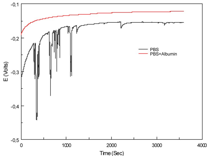
Figure 4.54: Effect of presence of 2 g/L Albumin on OCP value of stainless steel 316. Experimental conditions: T=37°C; pH=7.4; PBS with and without albumin addition.
