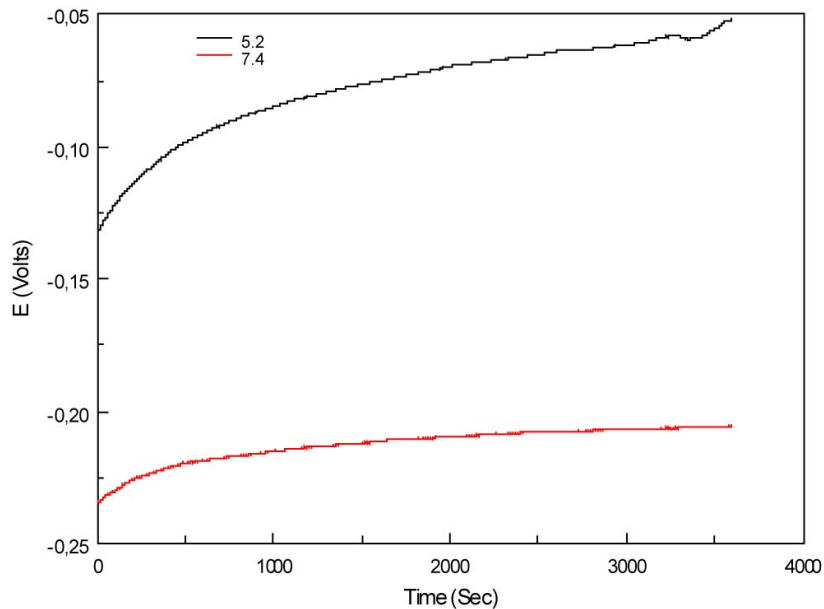
Figure 4.27: Effect of pH on OCP value of surgical grade Co-Cr-Mo grade F75. Experimental conditions: T=37°C; PBS with 2 g/L albumin; pH= 7.4 and 5.2.
