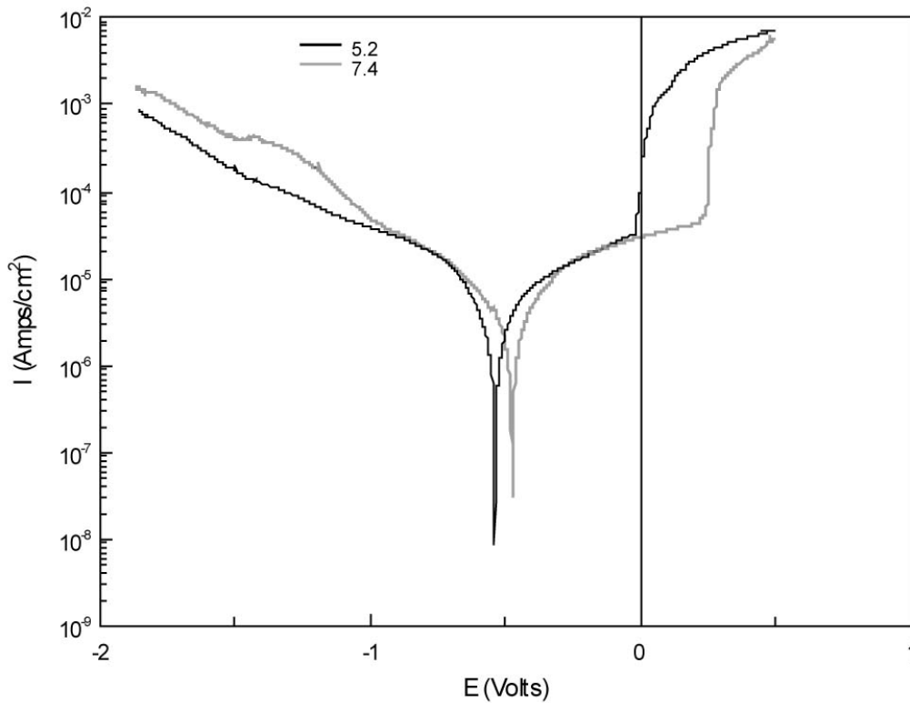
Figure 4.32: Effect of pH on the polarization curve of bulk metallic glass. Experimental conditions: T=37°C; PBS; pH=7.4 and 5.2.
