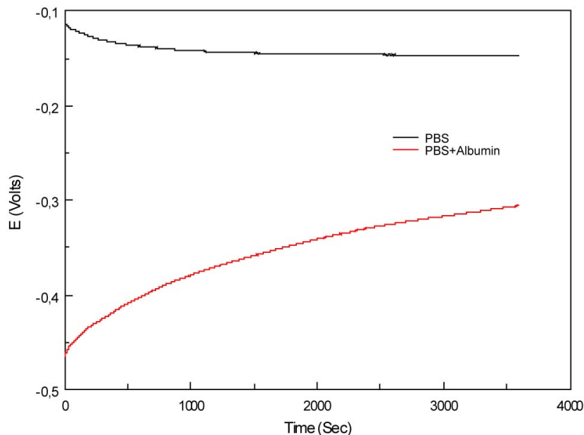
Figure 4.55: Effect of presence of 2 g/L Albumin on OCP value of stainless steel 316. Experimental conditions: T=37°C; pH=5.2; PBS with and without albumin addition.
