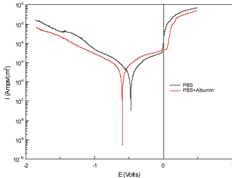
Figure 4.49: Effect of presence of 2 g/L Albumin on the polarization curves of zirconium based bulk metallic glass. Experimental conditions: T=37°C; pH=5.2; PBS without and with albumin addition.
