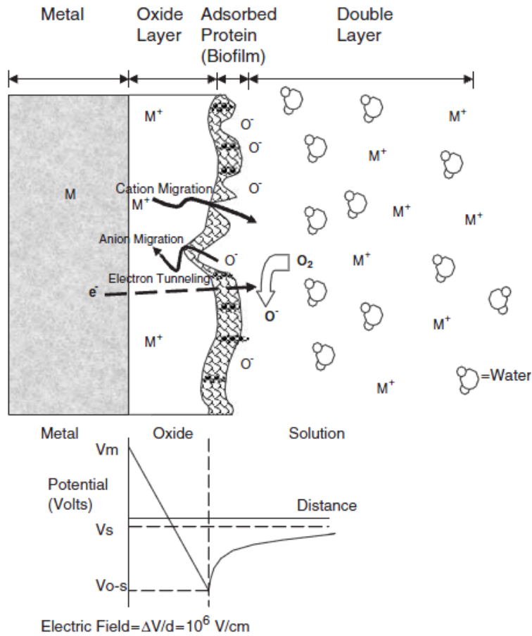
Figure 2.8: Schematic of the interface of a passivating alloy surface in contact with a biological environment [9].
