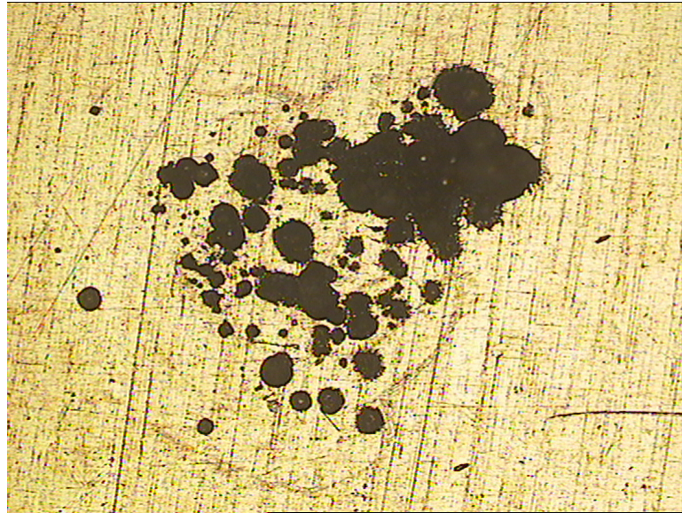
Figure 6.67: Pitting corrosion on the surface of the zirconium based bulk metallic glass in PBS solution. T=37°C; pH=7.4; Magnification 100X.
