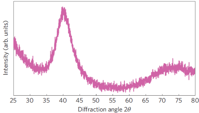
Figure 2.2: Amorphous structure of the Pd 79 Ag 3.5 P 6 Si 9.5 Ge 2 glass. X-ray diffraction analysis [37].
