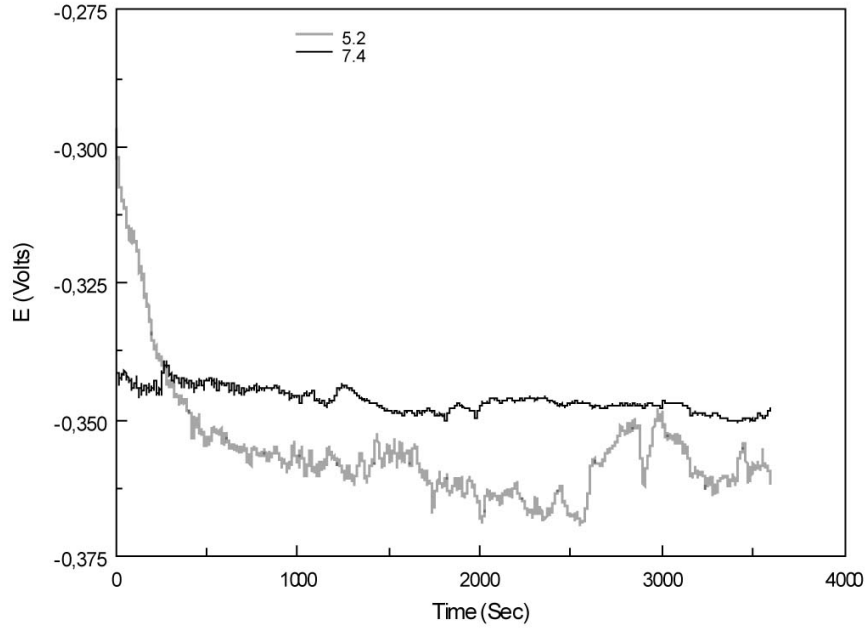
Figure 4.30: Effect of pH on OCP value of bulk metallic glass. Experimental conditions: T=37°C; PBS; pH=7.4 and 5.2.
