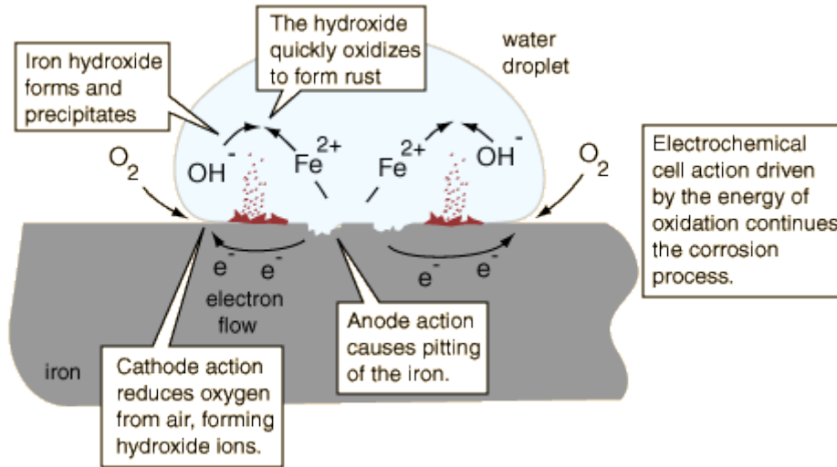
Figure 2.9: Schematic diagram of corrosion cells on iron [48].
