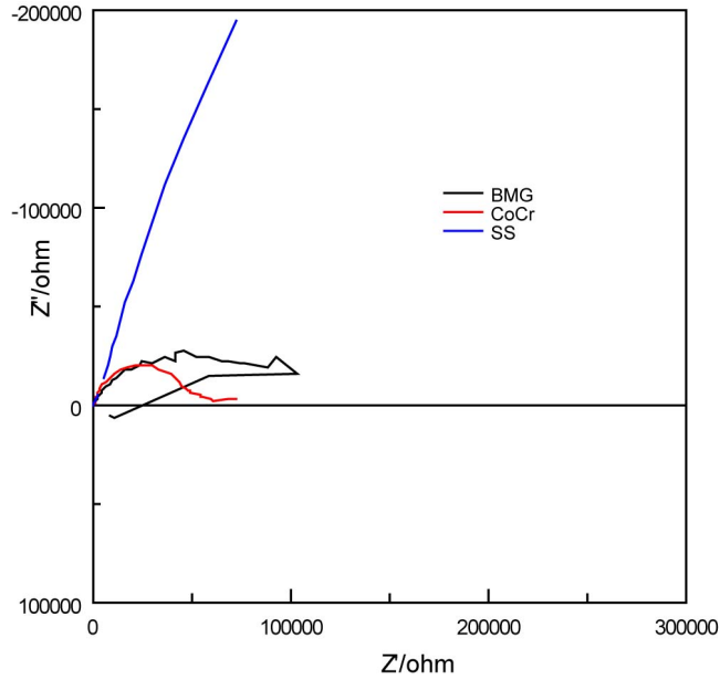
Figure 4.82: Experimental Nyquist plot in PBS, T=20\text{ }^{\circ}\text{C} , \text{pH } 7.4 , after holding the samples at open circuit potential for 1 h.
