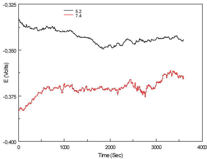
Figure 4.35: Effect of pH on OCP value of crystalline bulk metallic glass. Experimental conditions: Experimental conditions: T=37°C; PBS with 2 g/L albumin; pH=7.4 and 5.2.
