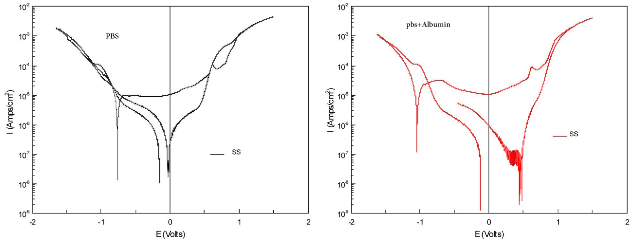
Figure 4.65: Effect of 2g/L albumin in the cyclic polarization curve for stainless steel 316. Experimental conditions: T=37°C; pH=7.4.
