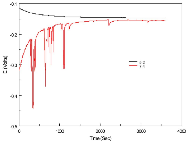
Figure 4.38: Effect of pH on OCP value of stainless steel 316. Experimental conditions: T=37°C; PBS; pH= 7.4 and 5.2.
