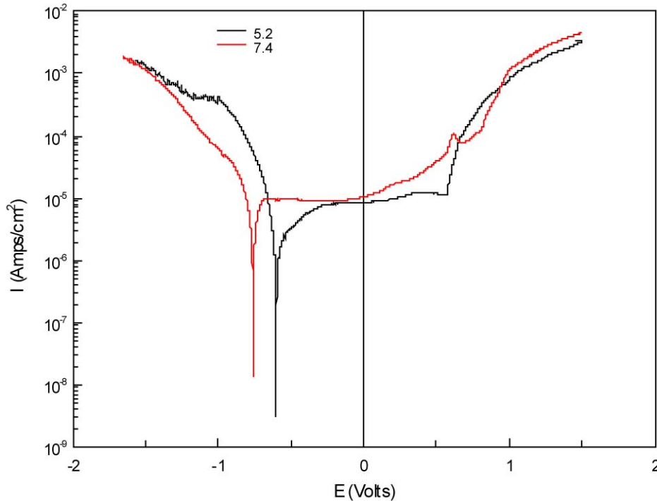
Figure 4.40: Effect of pH on the polarization curve of stainless steel 316. Experimental conditions: T=37°C; PBS; pH=7.4 and 5.2.
