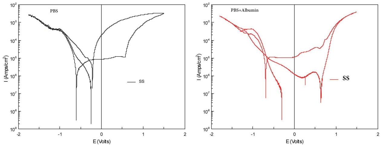
Figure 6.66: Effect of 2g/L albumin in the cyclic polarization curve for stainless steel 316. Experimental conditions: T=37°C; pH=5.2.
