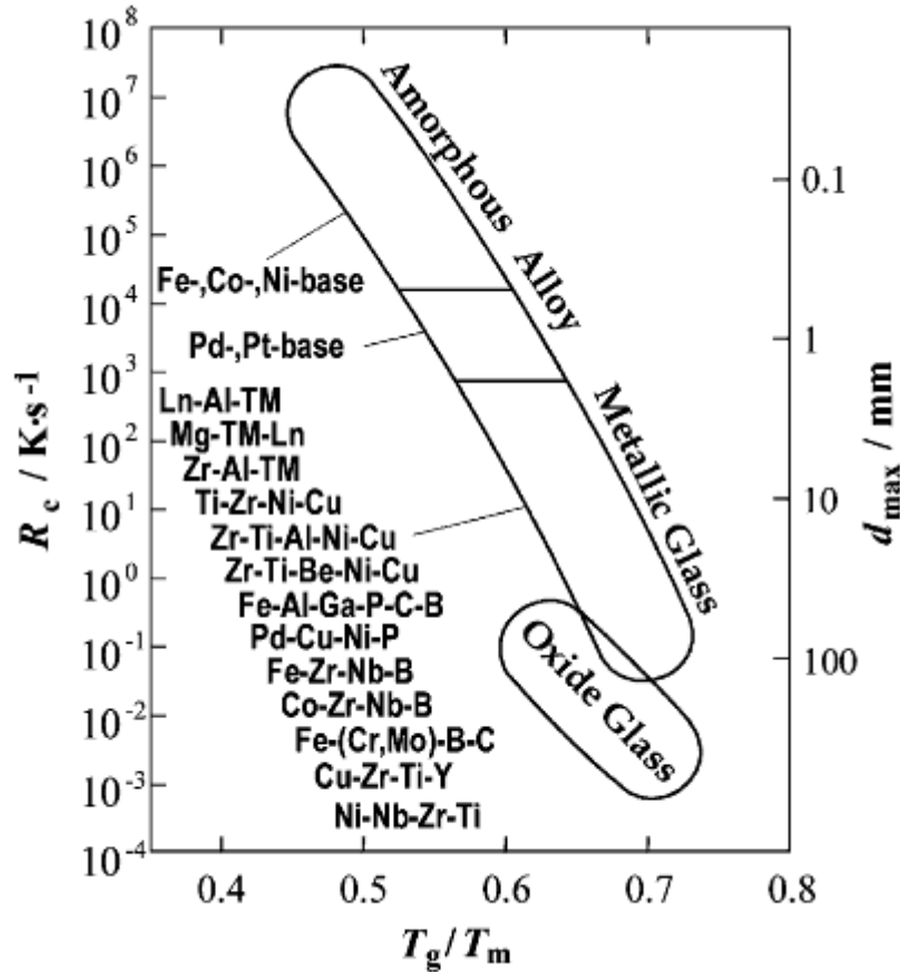
Figure 2.1: Relationship between the critical cooling rate for glass formation ( R_c ), maximum sample thickness for glass formation ( d_{max} ) and reduced glass transition temperature ( T_g/T_m ) for typical bulk glassy alloys. The data of amorphous alloys, previously reported Pd- and Pt-based glassy alloys and typical oxide glasses are also shown for comparison [35].
