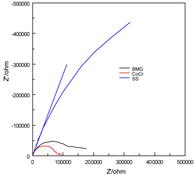
Figure 4.86: Experimental Nyquist plot in PBS with 2g/L albumin, T=20 °C, pH 7.4, after holding the samples at open circuit potential for 1 h.
