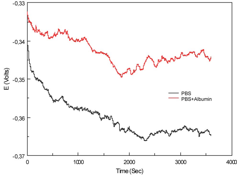
Figure 4.51: Effect of presence of 2 g/L Albumin on OCP value of crystalline zirconium based bulk metallic glass. Experimental conditions: T=37°C; pH=5.2; PBS with and without albumin addition.
