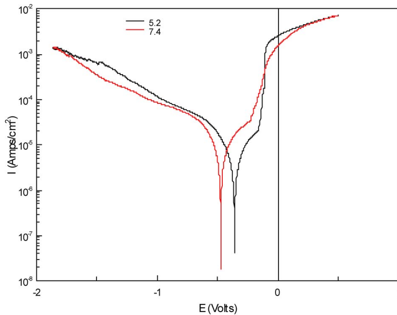
Figure 4.36: Effect of pH on the polarization curve of crystalline bulk metallic glass. Experimental conditions: T=37°C; PBS; pH=7.4 and 5.2.
