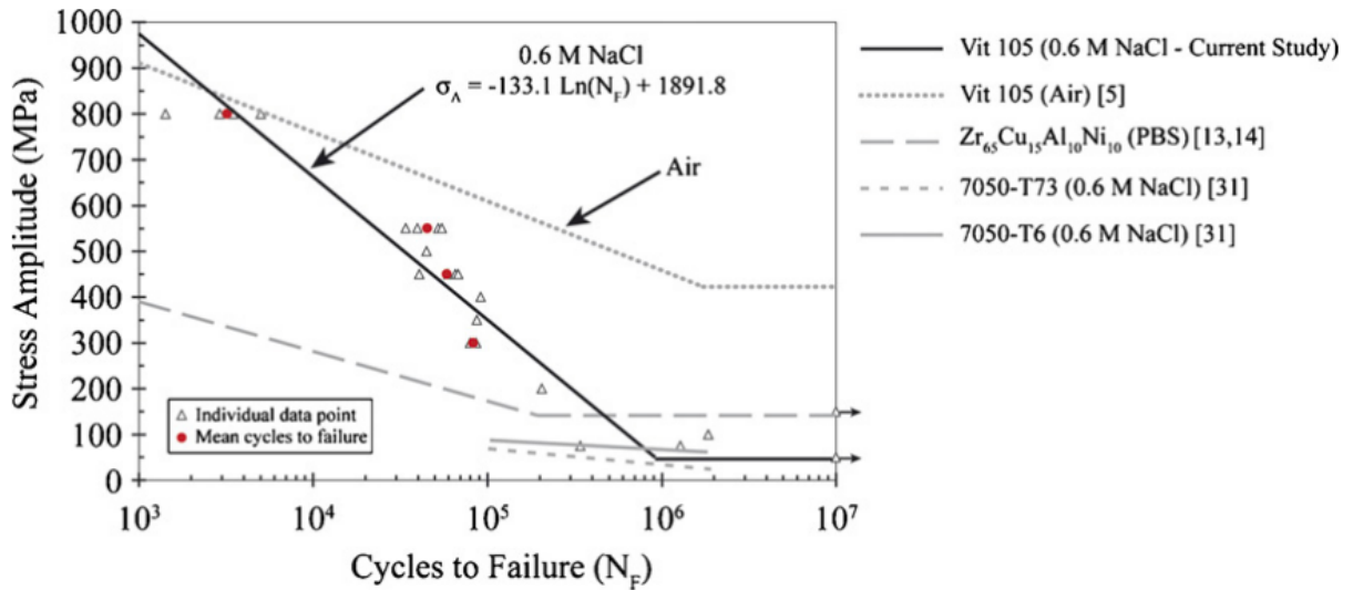
Figure 2.5: Plot of cycles to failure as a function of stress amplitude for the four-point bending of Vit 105 BMG in air and a naturally aerated, 0.6 M NaCl electrolyte at a frequency of 10 Hz and R= 0.1 [40].
