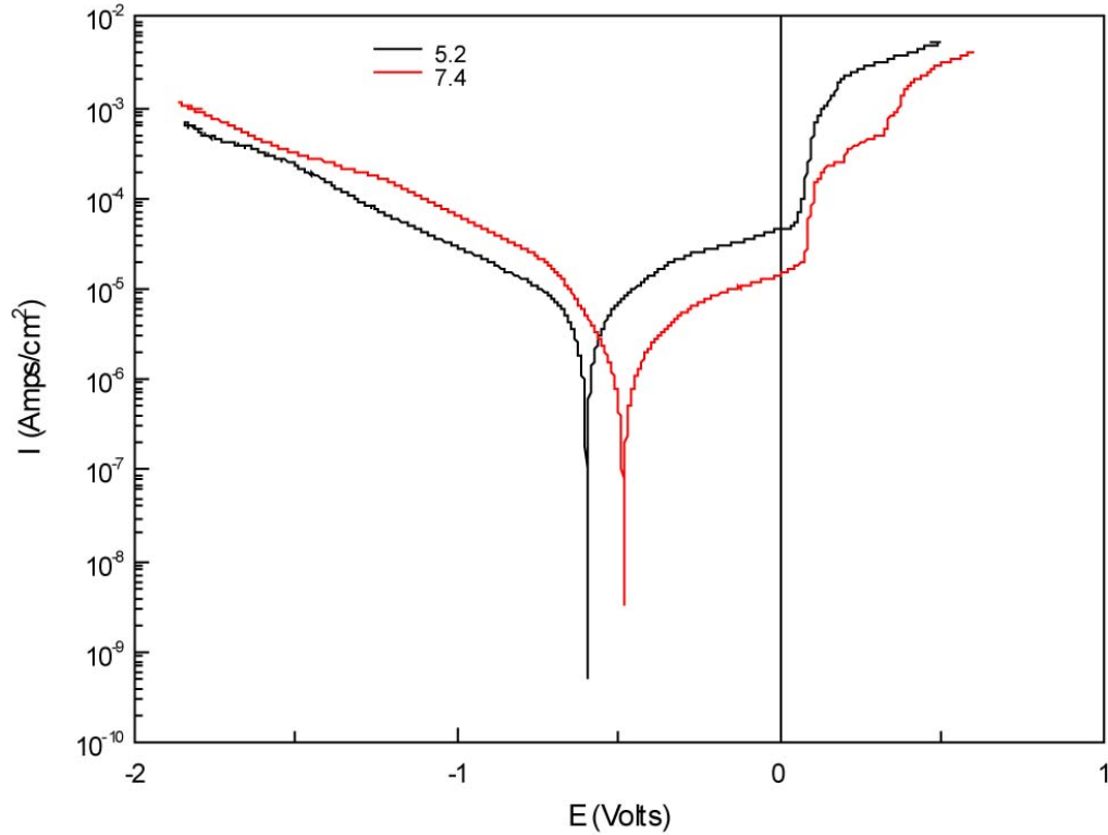
Figure 4.33: Effect of pH on the polarization curve of bulk metallic glass. Experimental conditions: T=37^{\circ}\text{C} ; PBS with 2 g/L albumin; \text{pH}=7.4 and 5.2.
