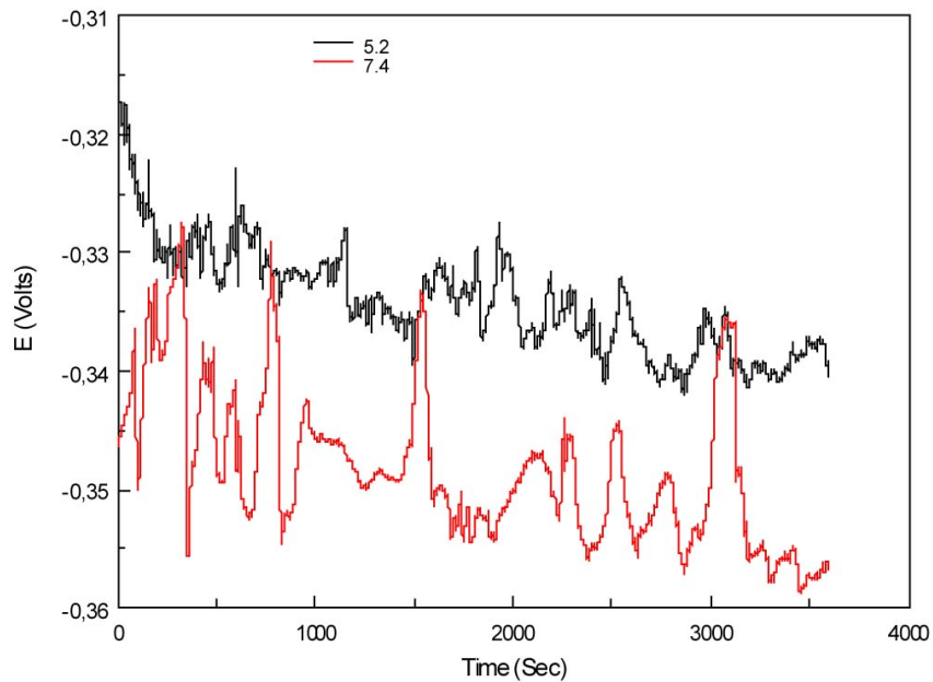
Figure 4.31: Effect of pH on OCP value of bulk metallic glass. Experimental conditions: T=37°C; PBS with 2 g/L albumin; pH=7.4 and 5.2.
