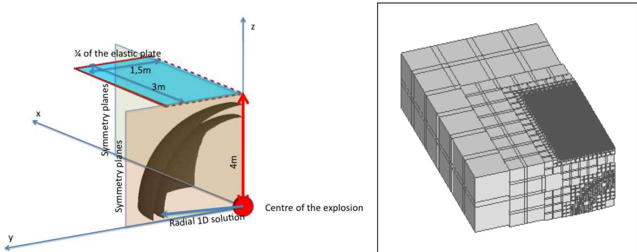
Figure 1: Left: sketch of the problem; a spherical pressure blast is generated by the explosion of a TNT charge positioned at the center of the fluid domain; the pressure wave impacts against an elastic plate. Right: example of the mesh used (the solid lines represent the block boundaries, each block is constituted by 6x6x6 cells).
