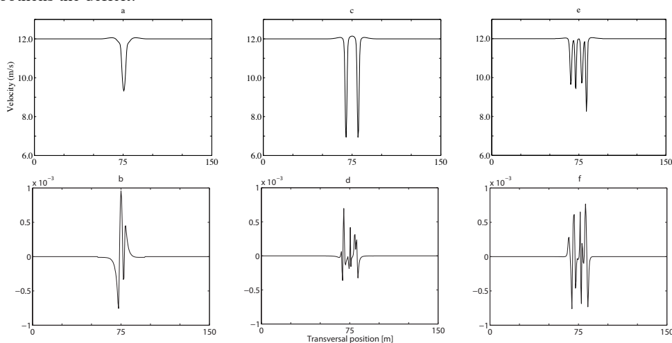
Figure 7. Mean velocity deficit (top) and time averaged unsteady motions (bottom) for monopile (left), truss 0 (middle) and truss 22.5 degrees (right).
