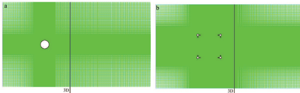
Figure 1. Grid for CFD simulations, line at 3D where rotor passes; monopile (left) and K-brace position for truss 0 degrees (right).
