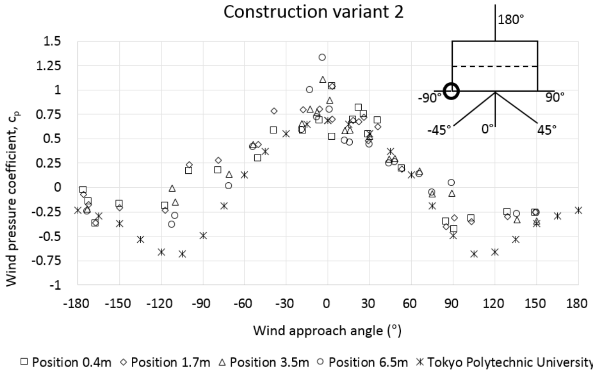
Fig. 8 Measured wind pressure coefficients, c_p , at four locations on the long wall 3.5m above the ground and different wind approach angles ( 0^\circ = perpendicular to the wall) for construction variant 2. Black circle in the upper-right corner of the diagram shows the corner from which the positions are measured.
