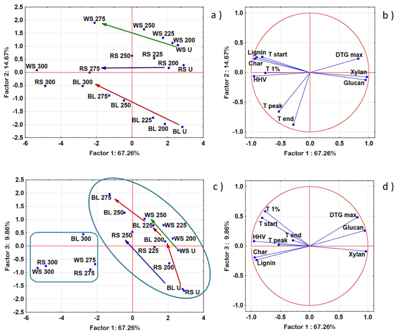
Figure 3. PCA score (a, c) and loading (b, d) plots based on the calorific values, thermogravimetric and chemical composition data. The arrows show the direction of the variation of the samples with increasing torrefaction temperatures. WS: wheat straw, RS: rape straw, BL: Black locust wood
