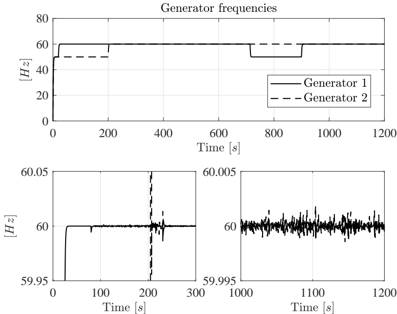
Figure 6.16: Generator frequencies
