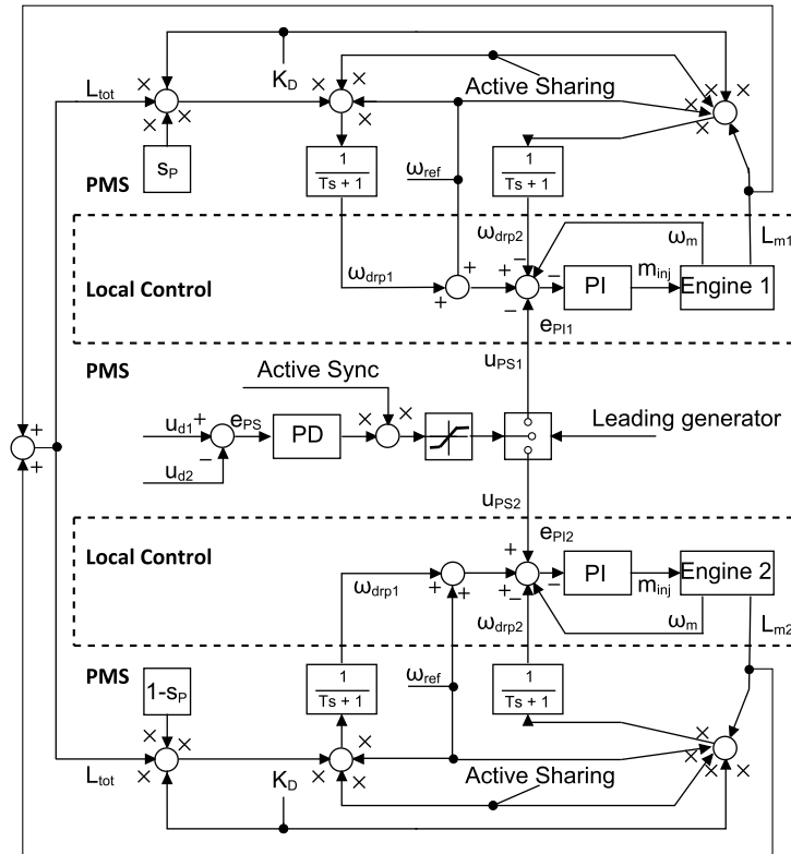
Figure 6.12: Engine speed control, active power sharing and phase synchronization for two gensets. Note that the leading generator, the one active having voltage output, is not affected by synchronization control
