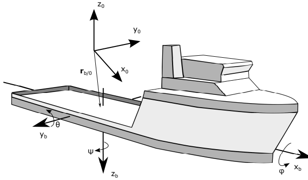
Figure 5.1: Illustration of kinematics of a marine vehicle.
