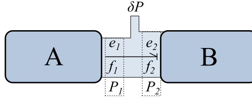
Figure 3.14: Power flow between two subsystems in a co-simulation
