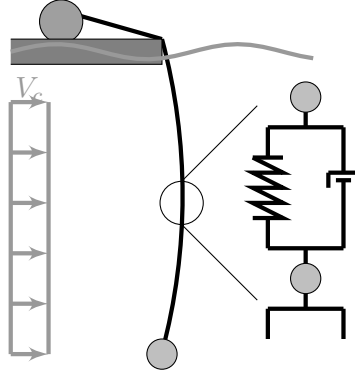
Figure 5.12: Sketch of winch in operation.
