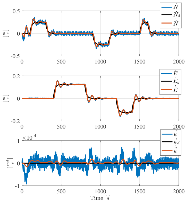
Figure 8.21: Simulation results comparing the estimated north-, east- and heading rates ( \hat{N} , \hat{E} and \hat{\psi} ) with the actual rates ( \dot{N} , \dot{E} and \dot{\psi} ) and the commanded rates ( \dot{N}_d , \dot{E}_d and \dot{\psi}_d )
