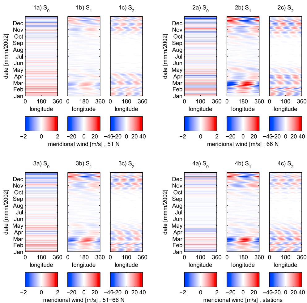
Figure 3. Hovmöller diagram of longitudinal wave components S_0 (a), S_1 (b), S_2 (c) using the “ideal” longitudinal fit for anomaly meridional UKMO winds (top left) at 51^\circ\text{N} , (top right) at 66^\circ\text{N} , and for the latitude band (bottom left) 51\text{--}66^\circ\text{N} for year 2002. (bottom right) Hovmöller diagram of longitudinal wave components using the anomaly meridional UKMO wind only at the coordinates of the SuperDARN chain for year 2002. Red and blue colors signify poleward and equatorward winds, respectively.
