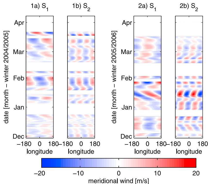
Figure 7. Longitudinal wave components (a) S_1 and (b) S_2 of the mean meridional wind anomalies, for (left) winter 2004–2005 and (right) winter 2005–2006. Red and blue colors signify poleward and equatorward winds, respectively.
