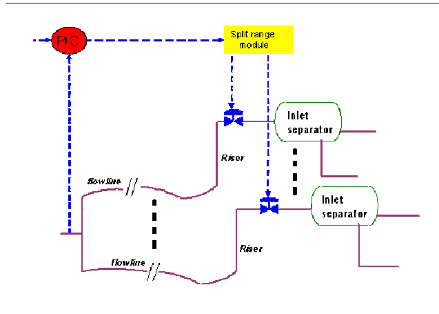
Figure 11: Slug control
