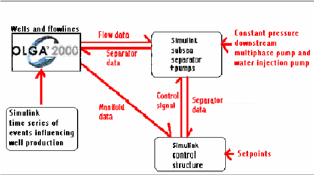
Figure 4: Simulation of wells and subsea separator
