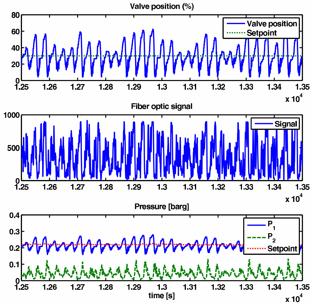
Figure A.7: Control quality when setpoint outer loop is 30%
