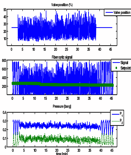
Fig. 21. Experimental results using a PI controller with density \rho as single measurement (no outer loop added)
