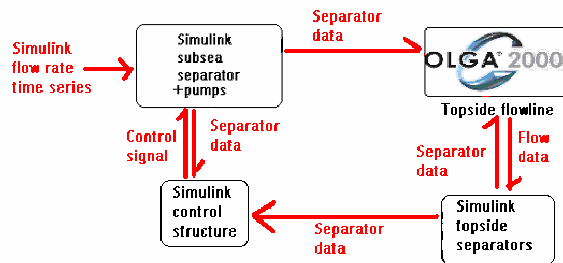
Figure 5: Simulation of subsea separator and topside pipelines
