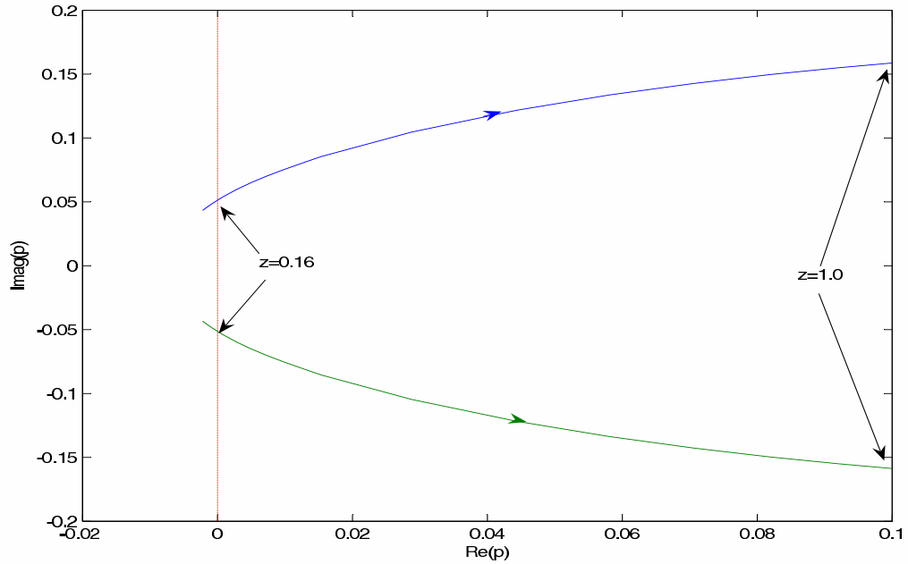
Figure 2.8: Root-locus plot showing the trajectories of the RHP open-loop poles when the valve opening varies from 0 (closed) to 1 (fully open)
