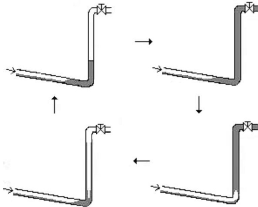
Figure 2.2: Graphic illustration of a slug cycle
