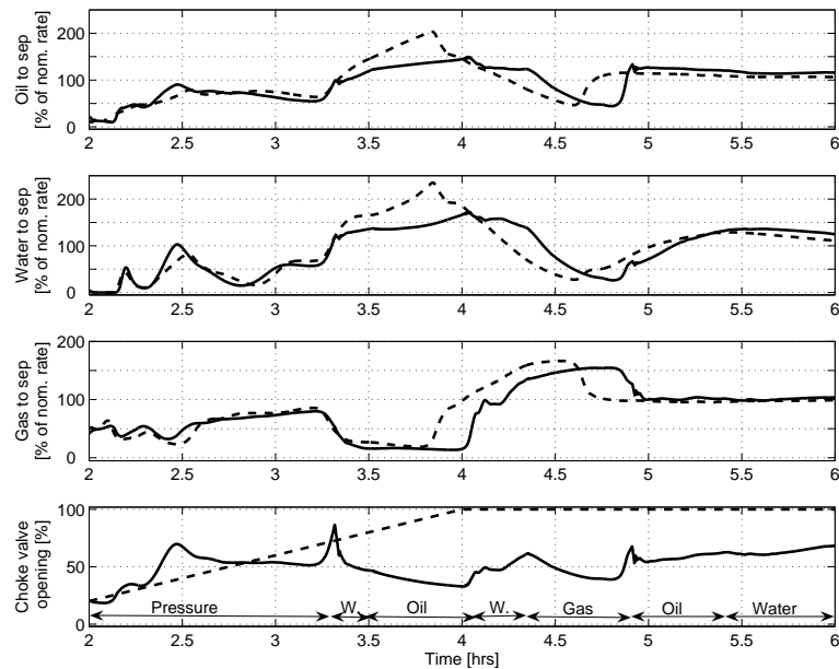
Figure 7.8: Startup-phase (A) for the oil-dominated case. Solid lines for controlled case, dashed lines for uncontrolled.
