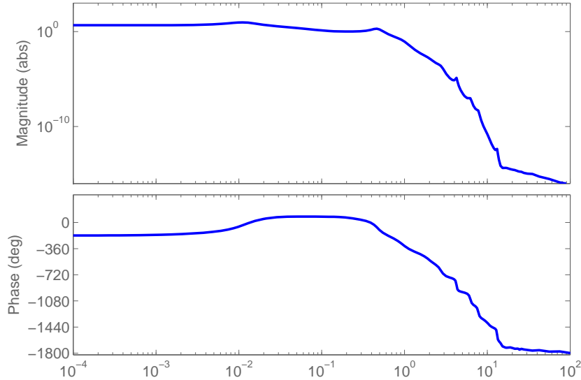
Figure 2.16: Bode diagram for process model G(s) , y = P_I at Z = 30\%
