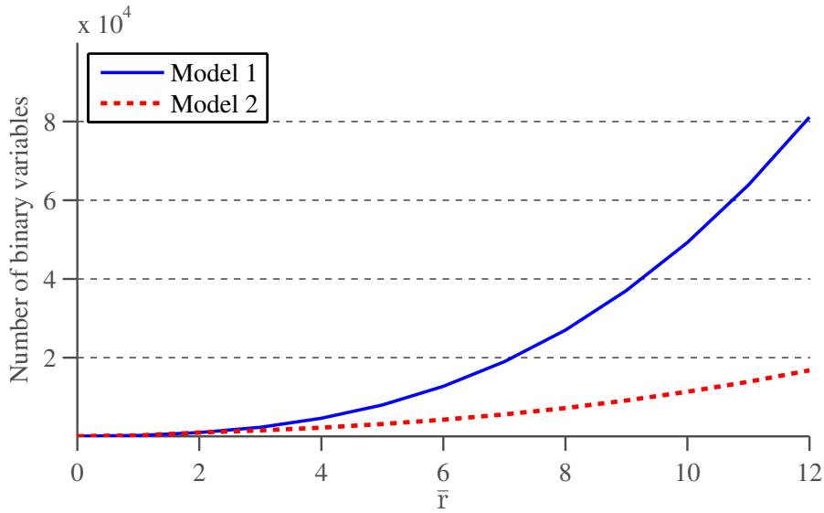
Figure 3: The number of binary variables in the two models as functions of the number of requests, \bar{r} , in the case when there are three demand responsive vehicles, eight transfer locations and two fixed route departures from each transfer location. The blue solid line corresponds to Model 1 and the red dotted line to Model 2.
